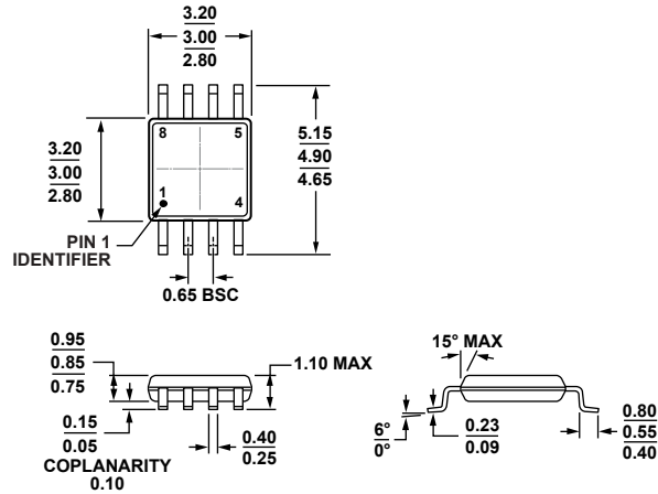
Figure 50. 8-Lead Mini Small Outline Package [MSOP] (RM-8) Dimensions shown in millimeters
