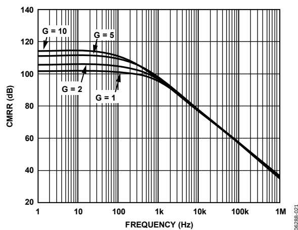
Figure 20. CMRR vs. Frequency, 1 k \Omega Source Imbalance
