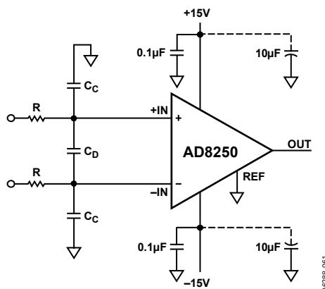
Figure 54. RFI Suppression
