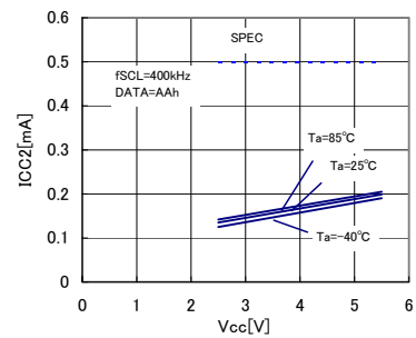
Fig.11 Current consumption at READ action ICC2 ( f_{SCL}=400kHz )
