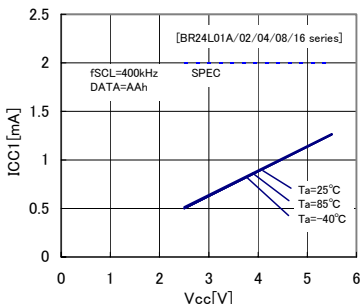
Fig.9 Current consumption at WRITE action ICC1 ( f_{SCL}=400kHz )
