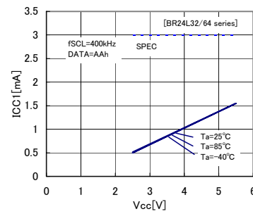
Fig.10 Current consumption at WRITE action ICC1 ( f_{SCL}=400kHz )
