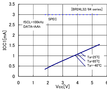
Fig.13 Current consumption at WRITE action ICC1 ( f_{SCL}=100kHz )
