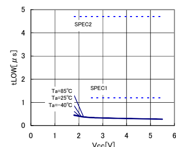
Fig.18 Data clock "L" time t_{LOW}
