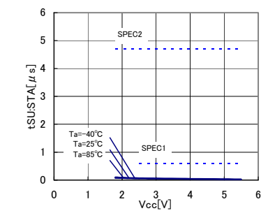
Fig.20 Start condition setup time t_{SU:STA}
