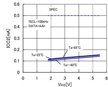
Fig.14 Current consumption at READ action ICC2 ( f_{SCL}=100kHz )
