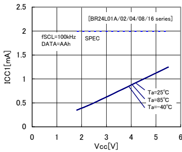
Fig.12 Current consumption at WRITE action ICC1 ( f_{SCL}=100kHz )
