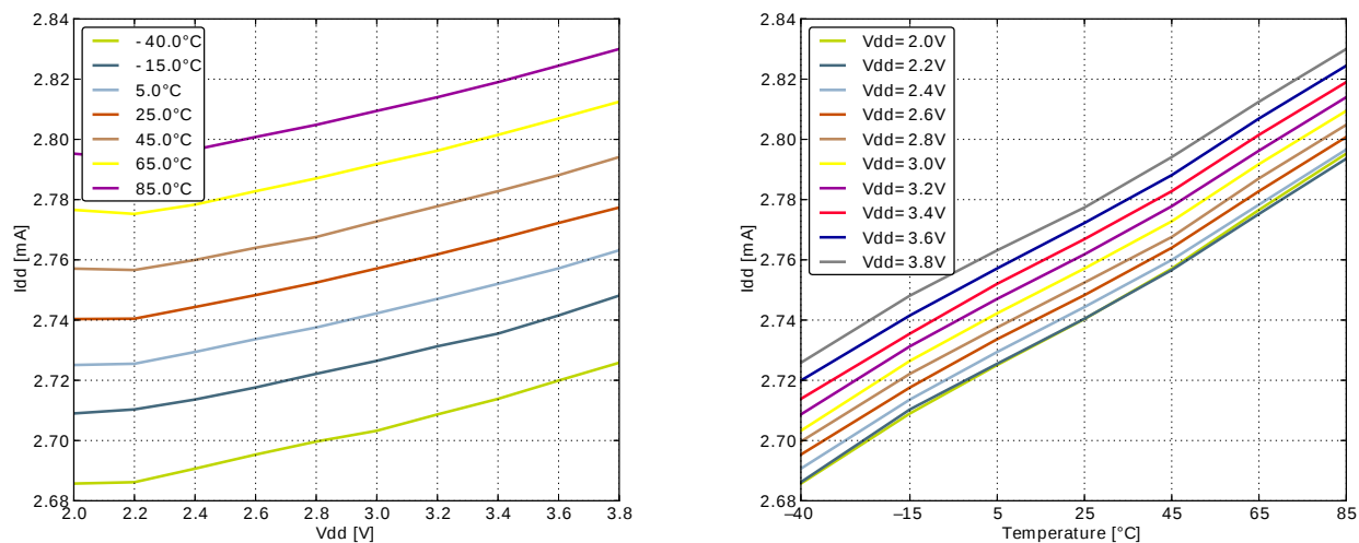
Figure 3.2. EM0 Current consumption while executing prime number calculation code from flash with HFRCO running at 21 MHz
