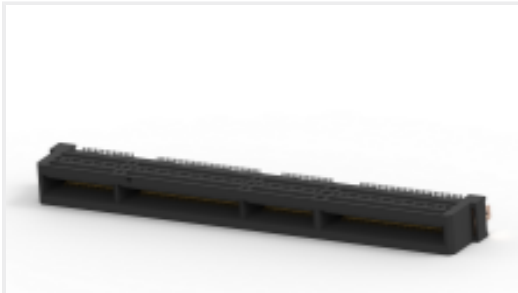
TE Part #7-2371899-7 PCIE G5 CONN,98P,ASSY,SLOT CUT, 30u",TR
