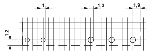
Drilling diagram
