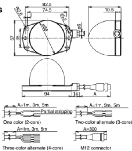
Mounting Hole Layout
