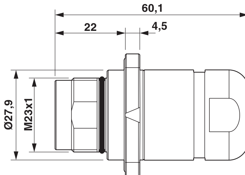
Dimensional drawing
