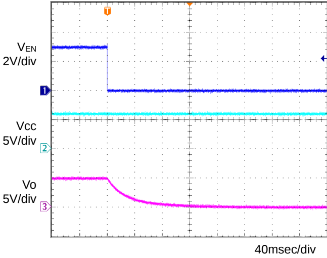
Fig.20 OFF sequence 2 C_o = 1\mu\text{F} , T_a = 125^\circ\text{C}
