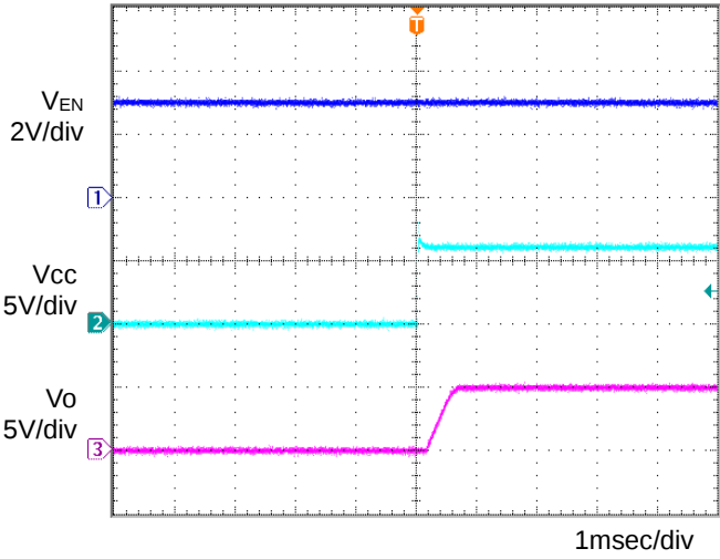
Fig.11 Input sequence 1 C_o=1\mu F, T_a=125^{\circ}C
