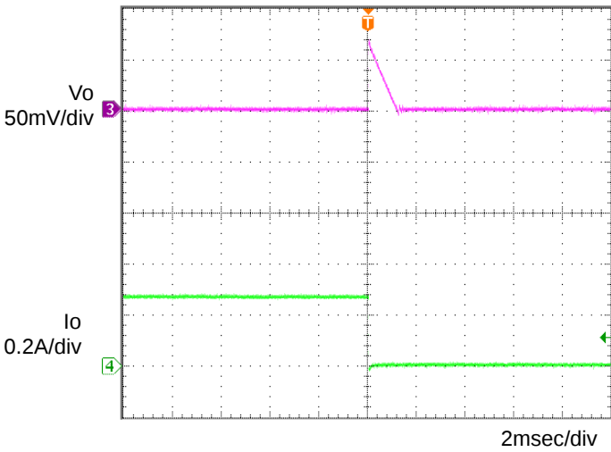
Fig.8 Transient Response (0.3→0A) Co=1μF,Ta=125°C
