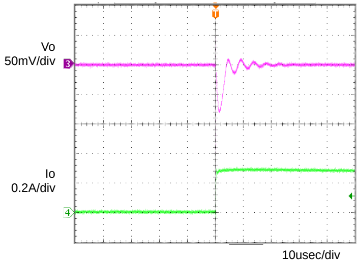
Fig.5 Transient Response (0→0.3A) Co=1\mu F , T_a=125^\circ C
