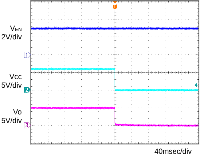
Fig.14 OFF sequence 1 C_o=1\mu F, T_a=125^{\circ}C
