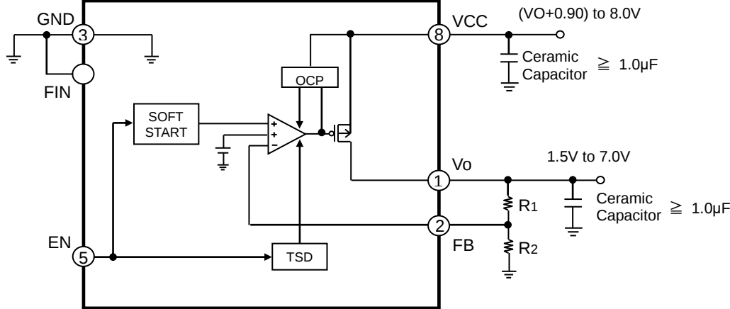
Fig.1 Block Diagram (Variable type)
