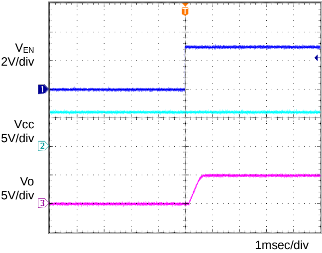
Fig.17 Input sequence 2 C_o=1\mu F, T_a=125^{\circ}C
