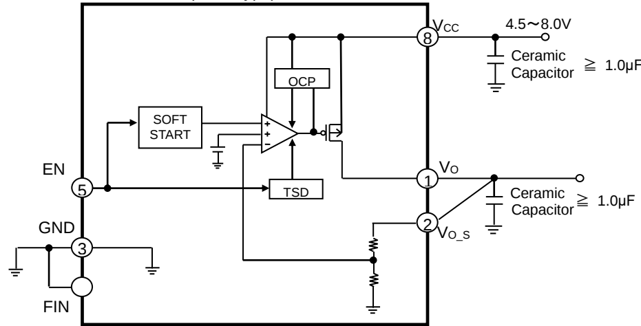
Fig.2 Block Diagram (Fixed type)
