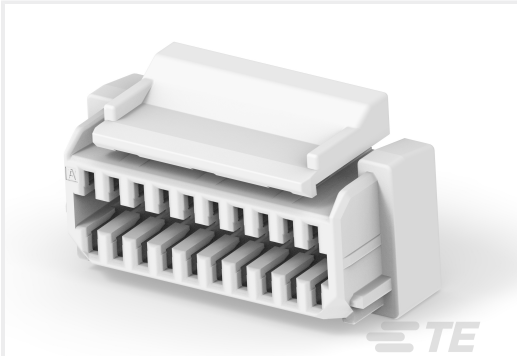
TE Part #2-2456588-0 Plug HSG, VT, KeyA, 20pos, SGI 1.25
