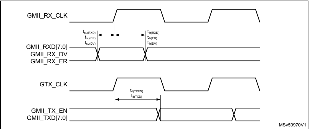
Figure 60. Ethernet GMII timing diagram
