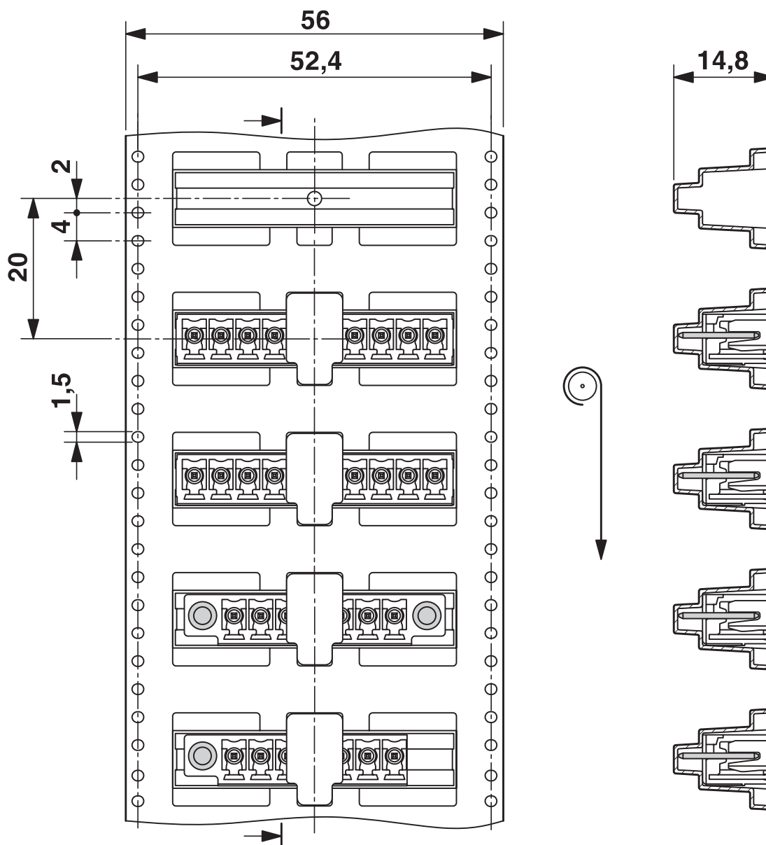
Dimensional drawing
