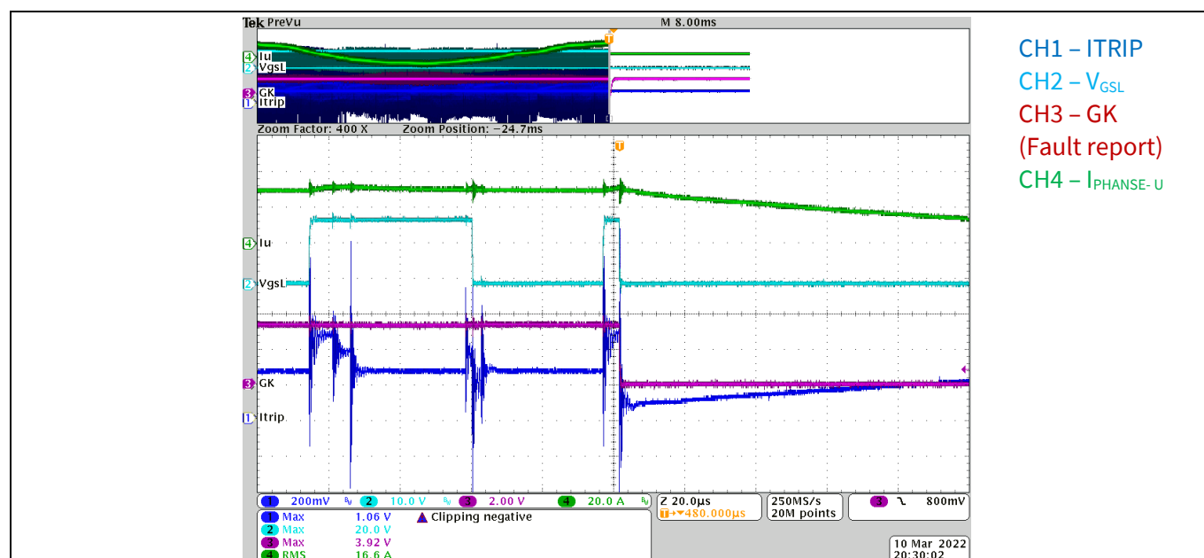
Figure 25 Overcurrent protection
