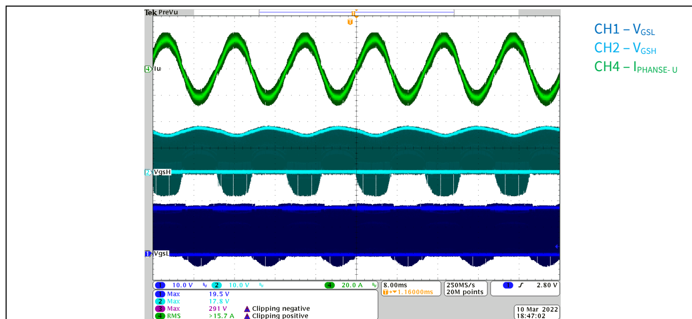
Figure 24 Phase U output current 15.7 A waveform at V_{IN} = 510 V, P_{IN} = 3 kW, F_{SW} = 12 kHz
