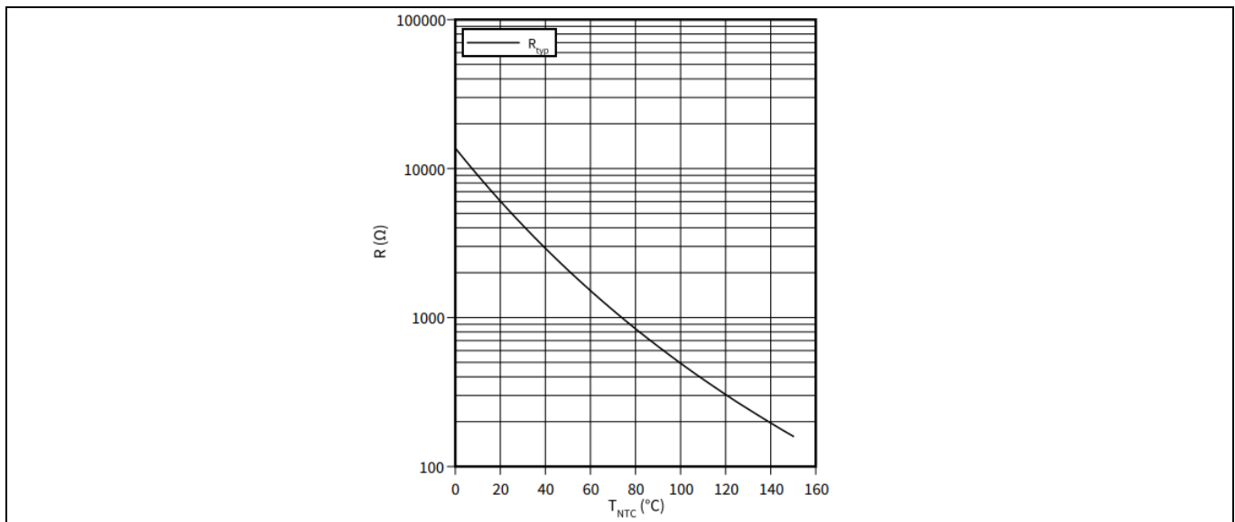
Figure 14 Typical temperature characteristic of the NTC thermistor
