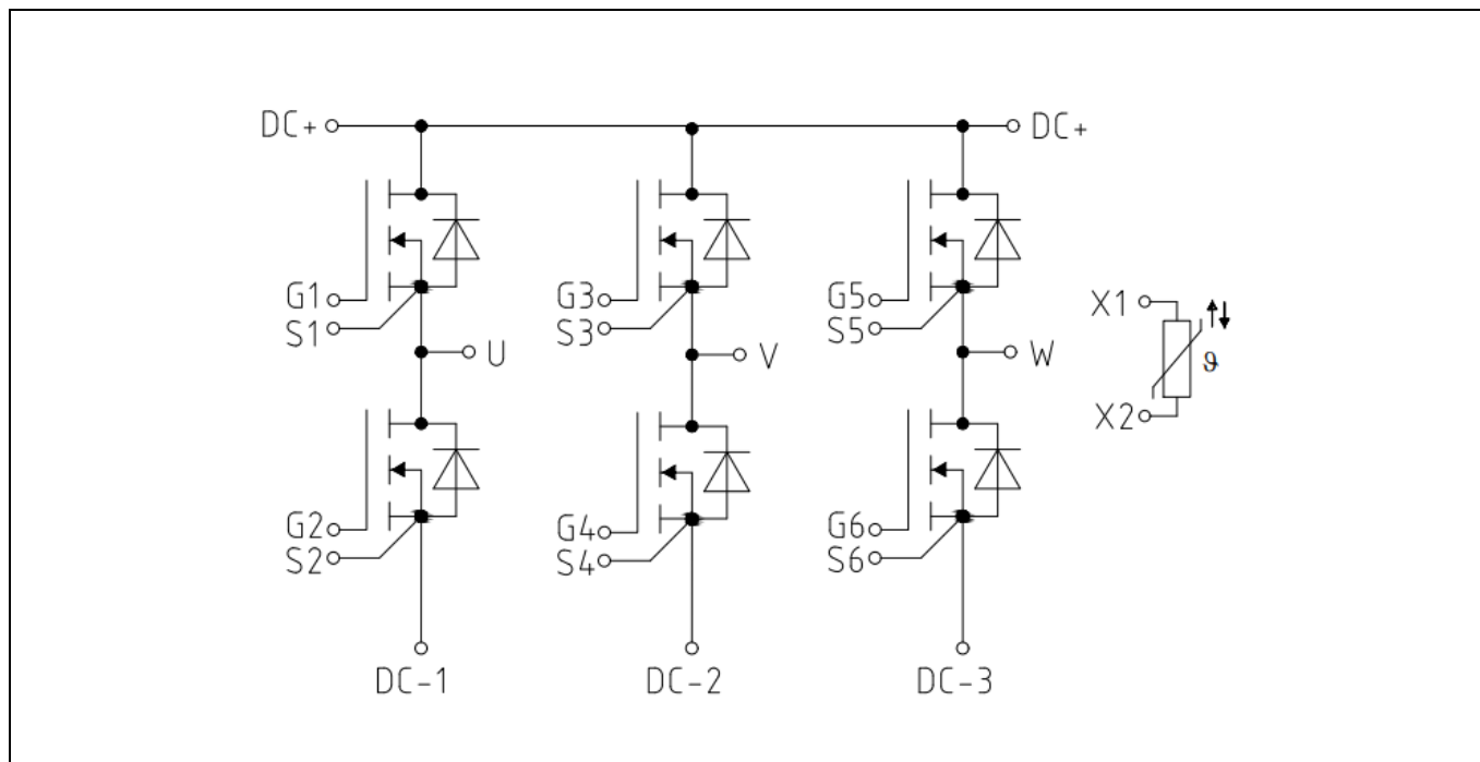
Figure 9 Circuit diagram
