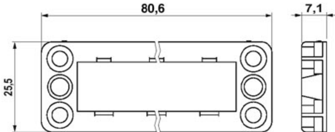
Dimensioned drawing
