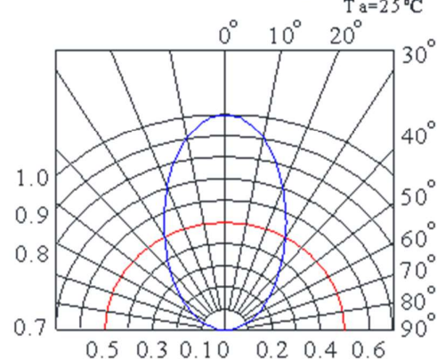
Radiation Diagram
