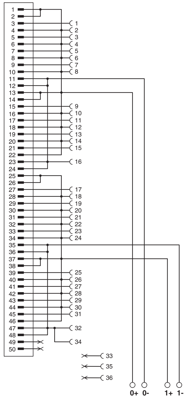
Circuit diagram
