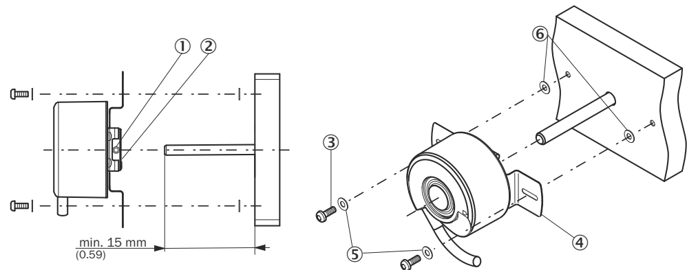
Figure 4: Mounting through hollow shaft with stator coupling 0, B, D, E, G (clamping at the front)
