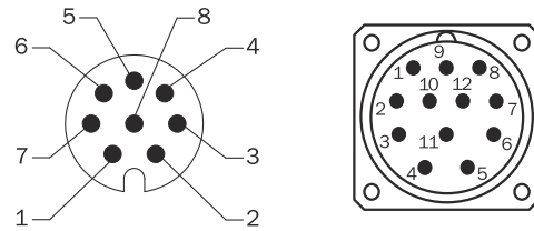
Figure 15: Left = View of M12 device plug Right = View of M23 device plug
