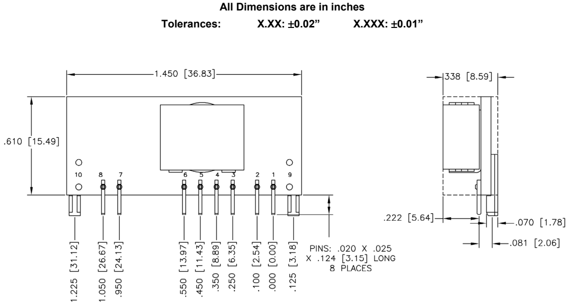
Figure 23. Mechanical Drawing
