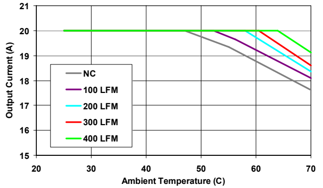
Figure 17. Derating Curves at Vo=3.3Vdc
