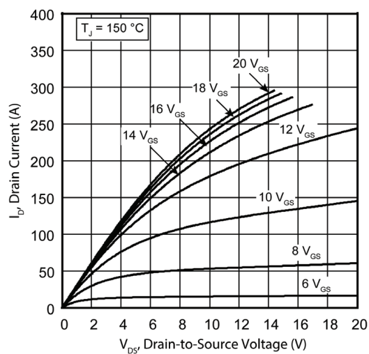
Figure 1-3. Drain Current vs. V_{DS} at V_{GS}
