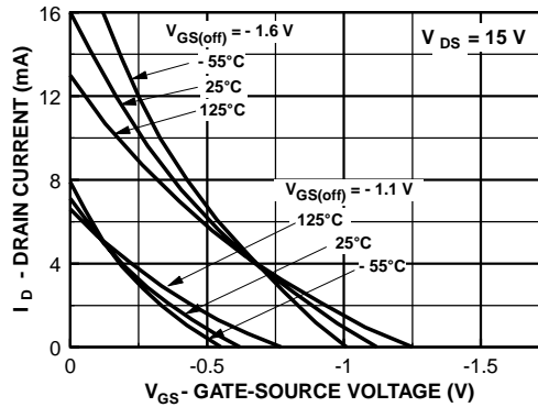
Transfer Characteristics
