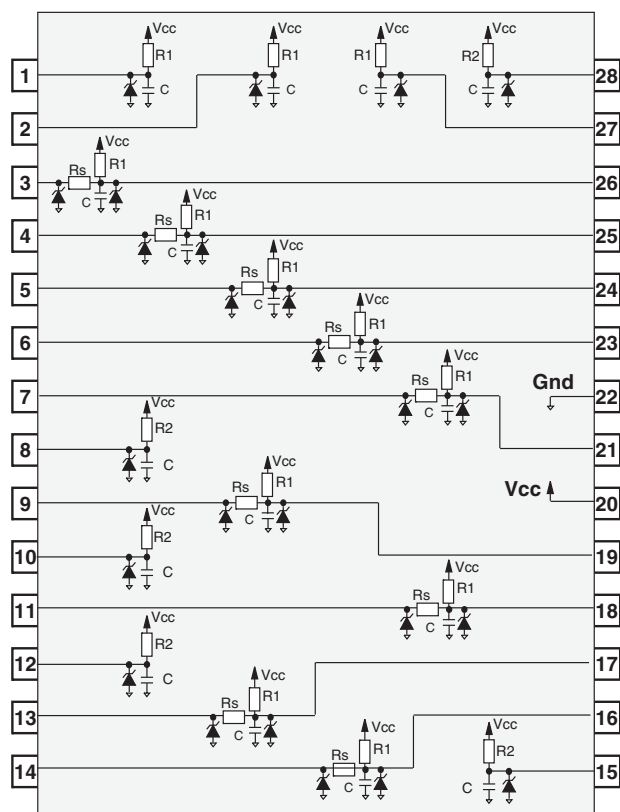
Figure 1. Schematic diagram
