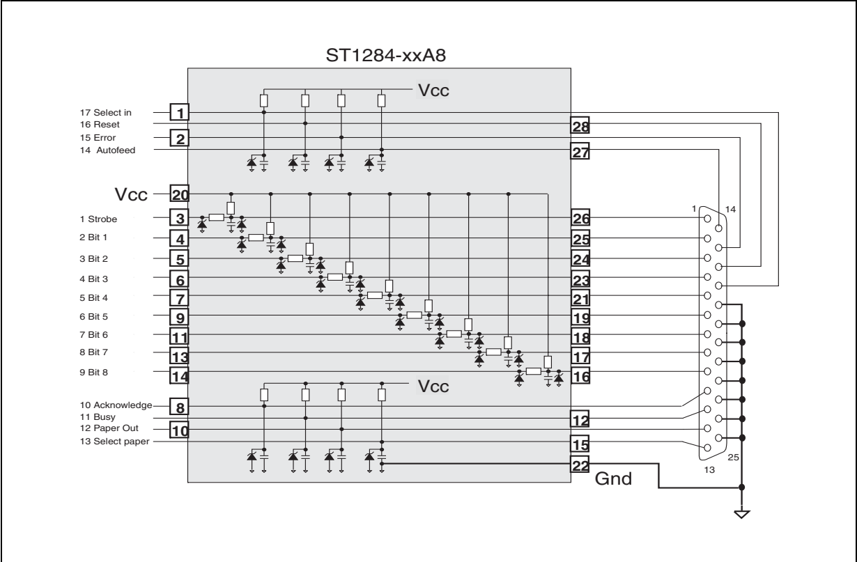
Figure 4. Functional diagram
