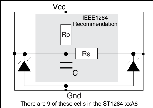
Figure 4. Functional diagram
