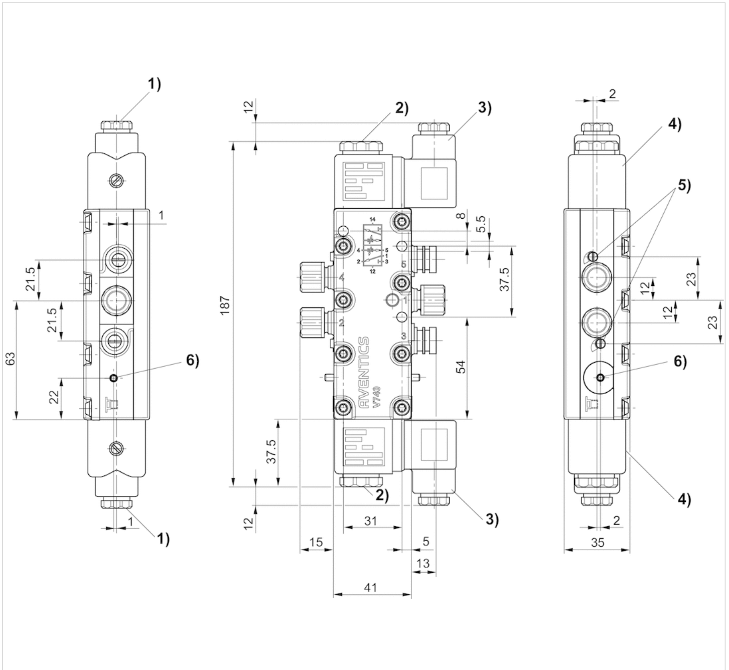
1) Gland fitting M16x1.52) M5 internal thread accessible under cap3) Valve plug connector can be rotated at 90° intervals4) Coil can be plugged at 45° intervals5) Flow control screw for exhausts 5 (R) and 3 (S)6) Manual override and position indicator
