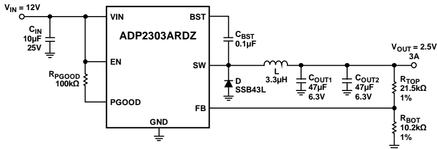
Figure 61. ADP2303 Typical Application, V_{IN} = 12\text{ V} , V_{OUT} = 2.5\text{ V} , 3 A
