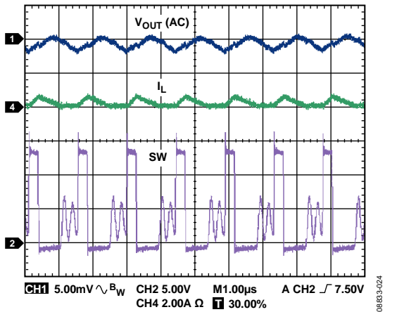
Figure 24. Discontinuous Conduction Mode (DCM), V_{OUT} = 3.3\text{ V} , V_{IN} = 12\text{ V}
