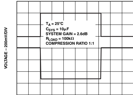
TPC 10. Large Signal Transient Response
