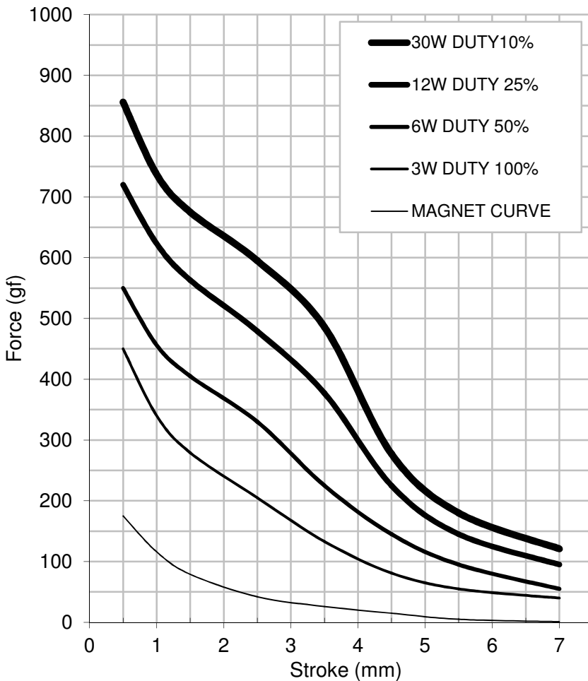
Force/Stroke Characteristics
