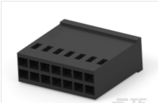
TE Part # 1-86177-4 14 MODIV HSG COMP DR .100CL
