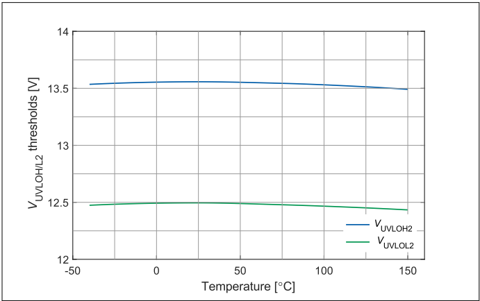
Figure 11 V UVLOH2 and V UVL0L2 (2ED3146MC12L) vs. temperature
