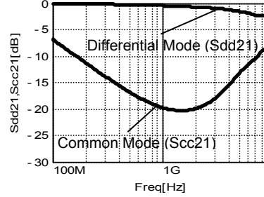
Insertion Loss
