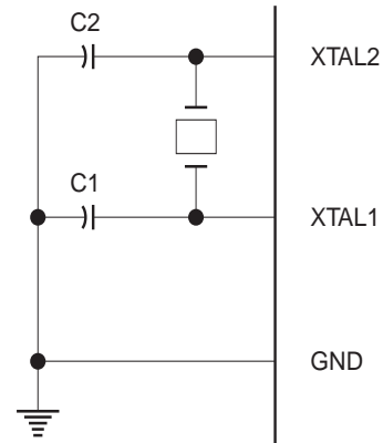
Figure 7. Oscillator Connections
