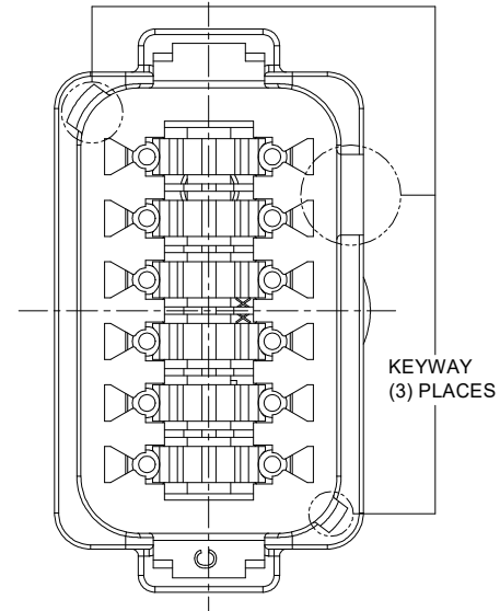
P/N AT04-12PC KEY-C CONFIGURATION STANDARD COLOR: GREEN
