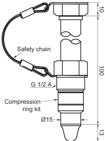
G 1/2 A hygienic, sliding connection, 100 mm adjustable, including compression ring kit ZPX1-006 (BCID: A03)
