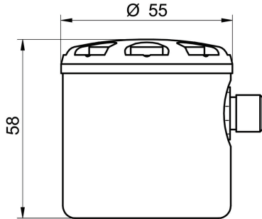
Housing with connector M12-A, 4-pin
