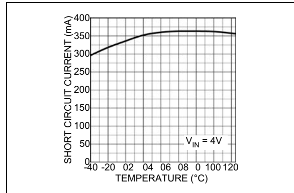
FIGURE 2-16: Short-Circuit Current vs. Temperature.
