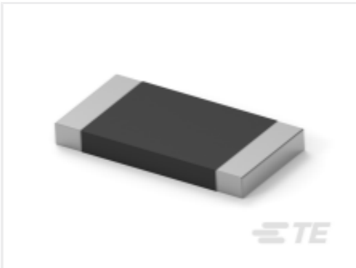
TE Part #6-2176422-7 TLRP 2512 3.0W R050 1% 50PPM 4K RL
