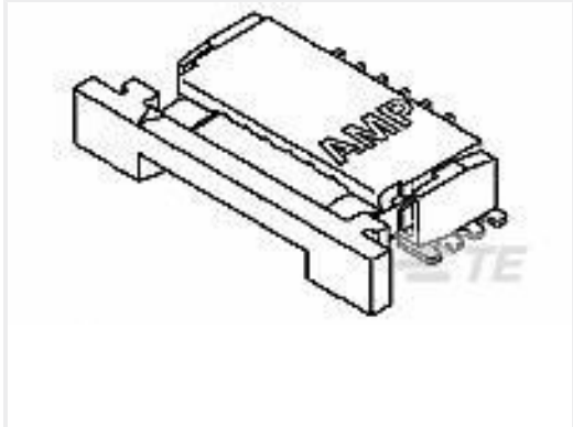
TE Part #1-84952-5 1MM FPC HORZ.BTTM CONT.ASS.15P
