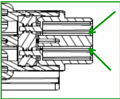
Orientation Feature
