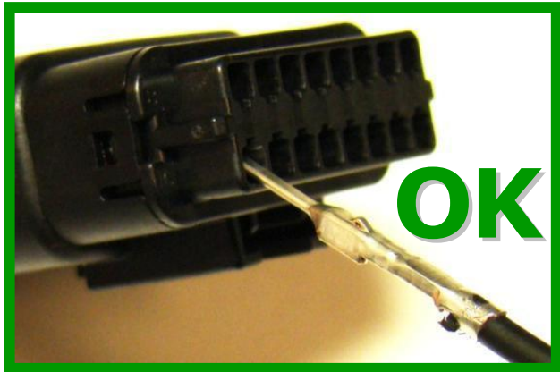
Orientation Feature
