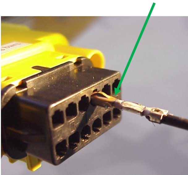
Correct Orientation
