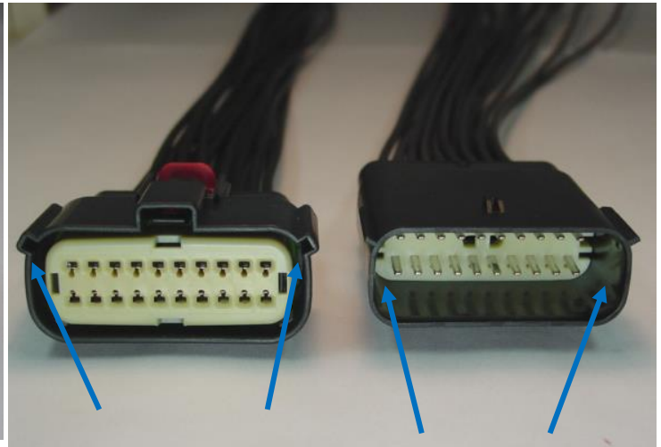
Keying Features
