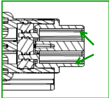
Orientation Feature
