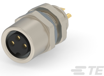
TE Part #T4033014031-000 M8.FMLE.PNLFRONT.3POS.STR
