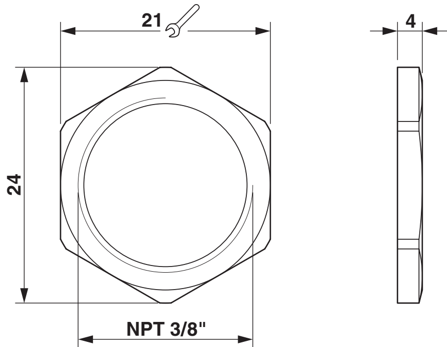
Dimensional drawing
