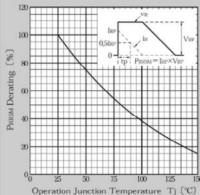
Repetitive Surge Reverse Power Derating Curve
