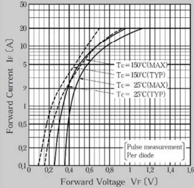
Forward Voltage
