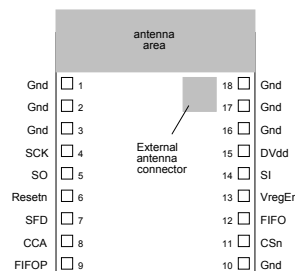
Figure 1. EasyBee pinout
