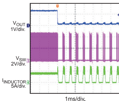
Short-Circuit Entry
