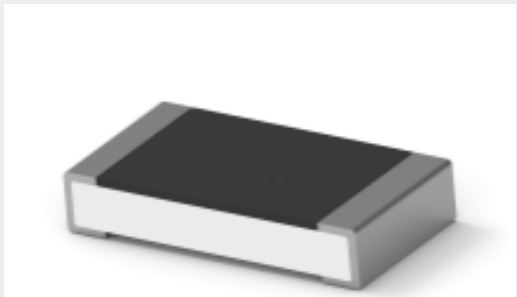
TE Part #5-2176389-1 RQ 1206 357R 0.1% 10PPM 5K RL
