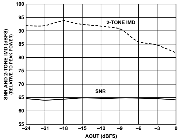
Figure 35. SNR and SFDR vs. P_{OUT} ( f_{OUT} = 12.5 MHz, f_{DATA} = 50 MSPS, 4× Interpolation)
