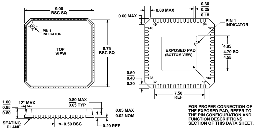
*COMPLIANT TO JEDEC STANDARDS MO-220-VMM4-4 EXCEPT FOR EXPOSED PAD DIMENSION Figure 6. 64-Lead Lead Frame Chip Scale Package [LF CSP_VQ] 9 mm x 9 mm Body, Very Thin Quad (CP-64-1) Dimensions shown in millimeters
