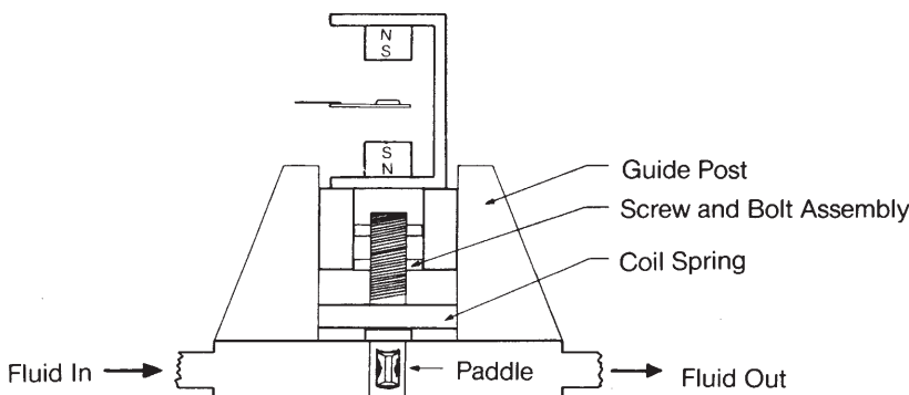
Figure 9 LOHET™ Float Meter
