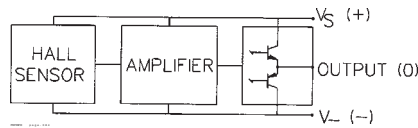
Figure 2 Block Diagram
