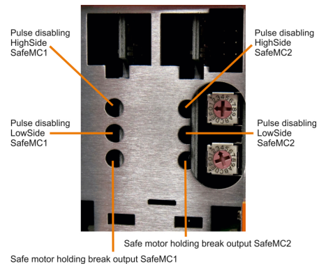
Figure 5: 2-axis modules
