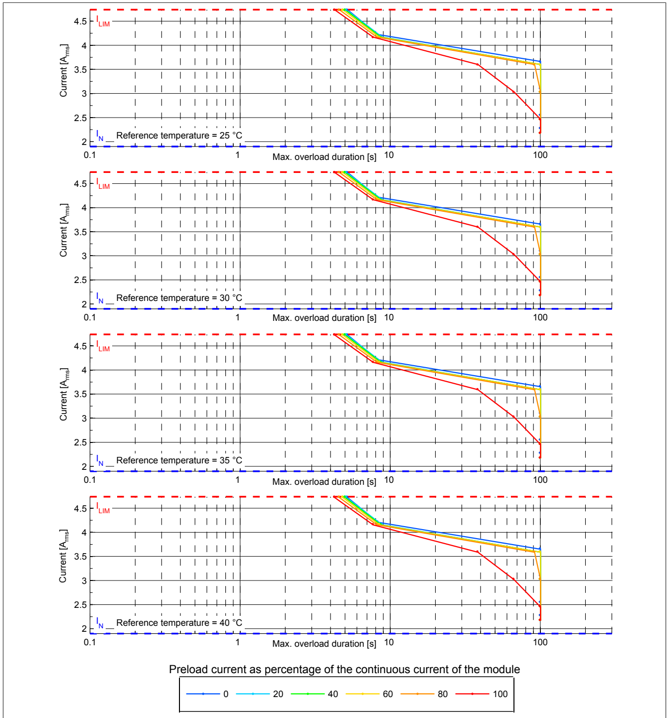
Figure 2: 8BVI0014HWDx.000-x - Overload characteristics, overload response - ERROR + STOP
