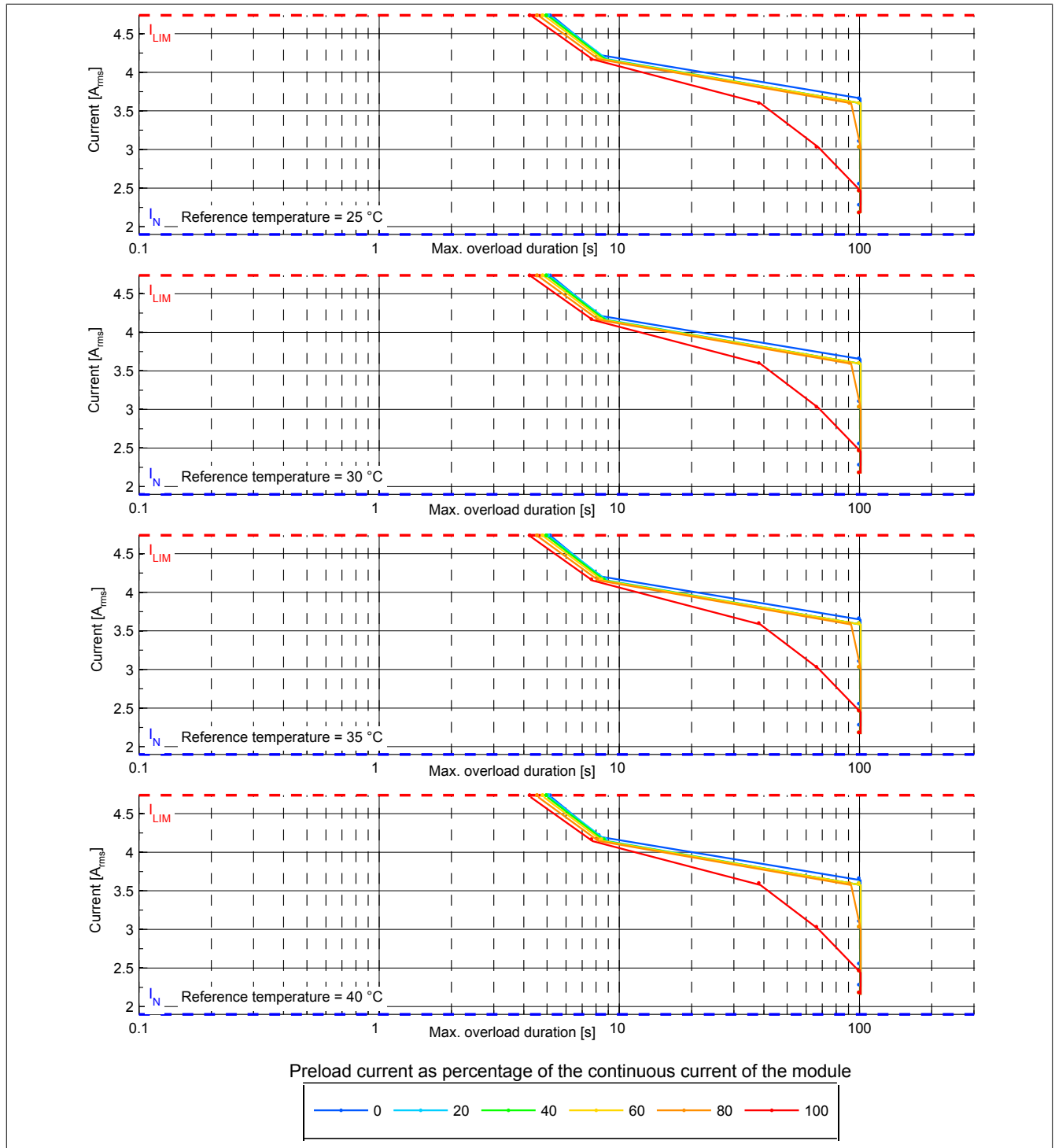
Figure 1: 8BVI0014HWDS.000-x - Overload characteristics, overload response - WARNING
