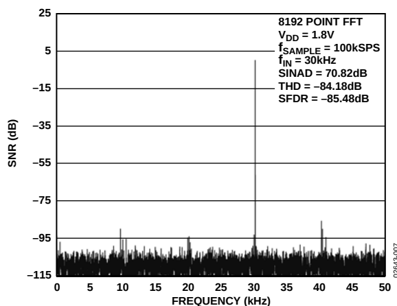
Figure 6. AD7466 Dynamic Performance at 100 kSPS
