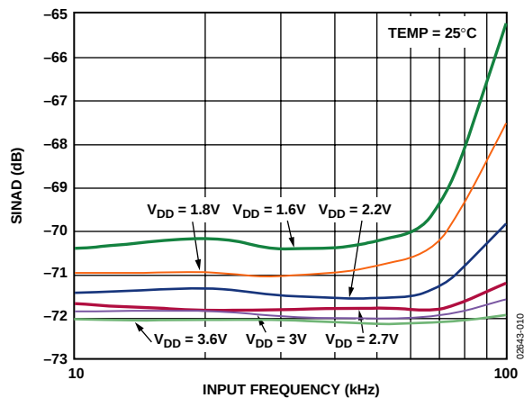
Figure 9. AD7466 SINAD vs. Analog Input Frequency at 100 kSPS for Various Supply Voltages
