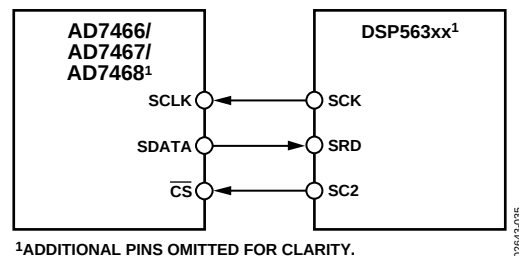
Figure 34. Interfacing to the DSP563xx
