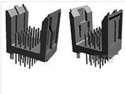
TE Part #5536501-3 2MM FB,ASY,96,SIG,HDR,SL,4.25
