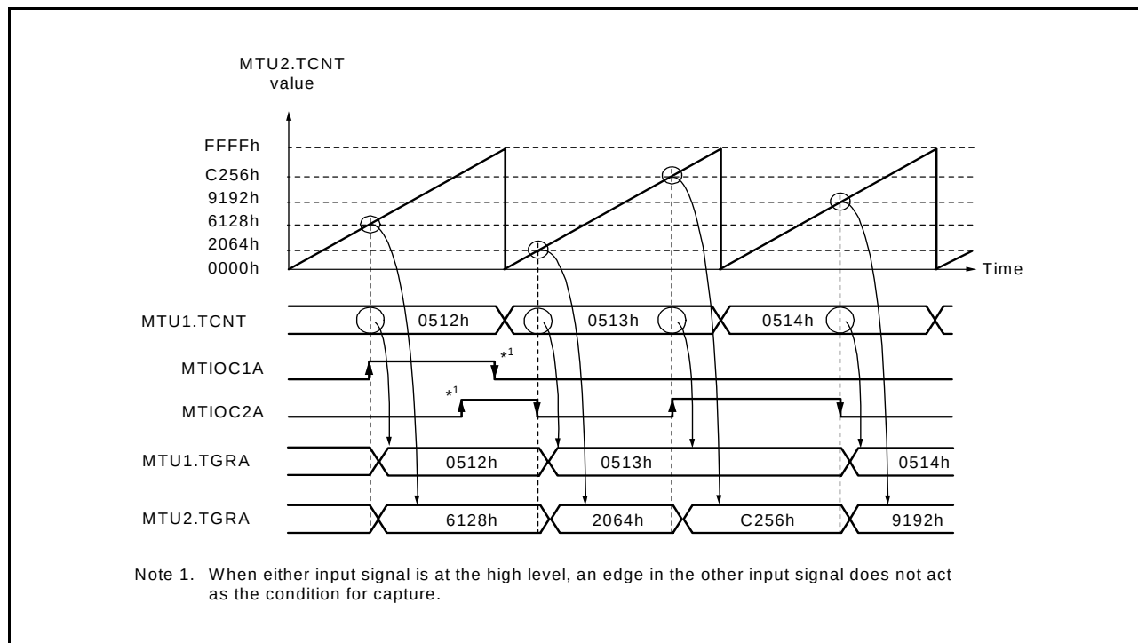
Figure 22.23 Cascaded Operation Example (c)
