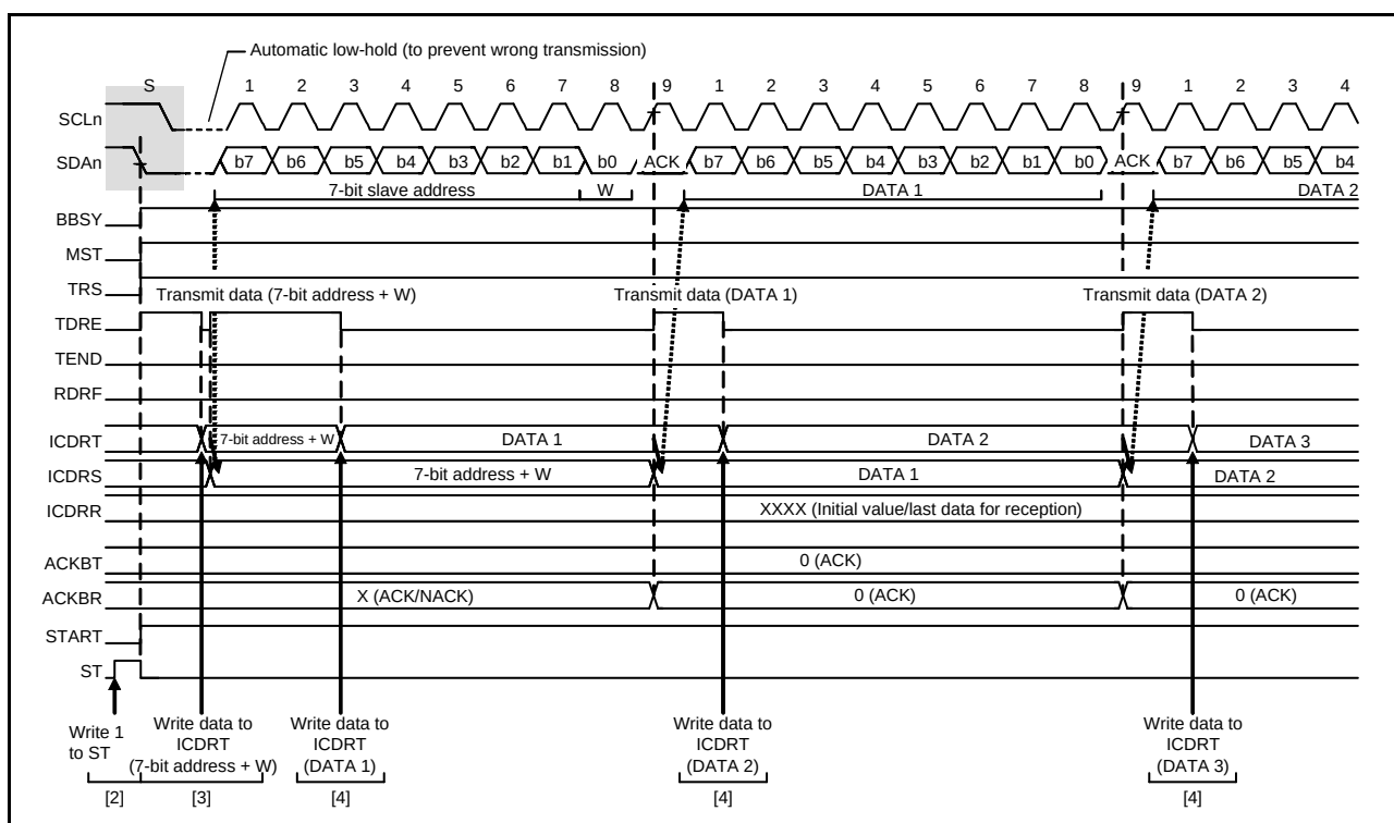
Figure 33.7 Master Transmit Operation Timing (1) (7-Bit Address Format)
