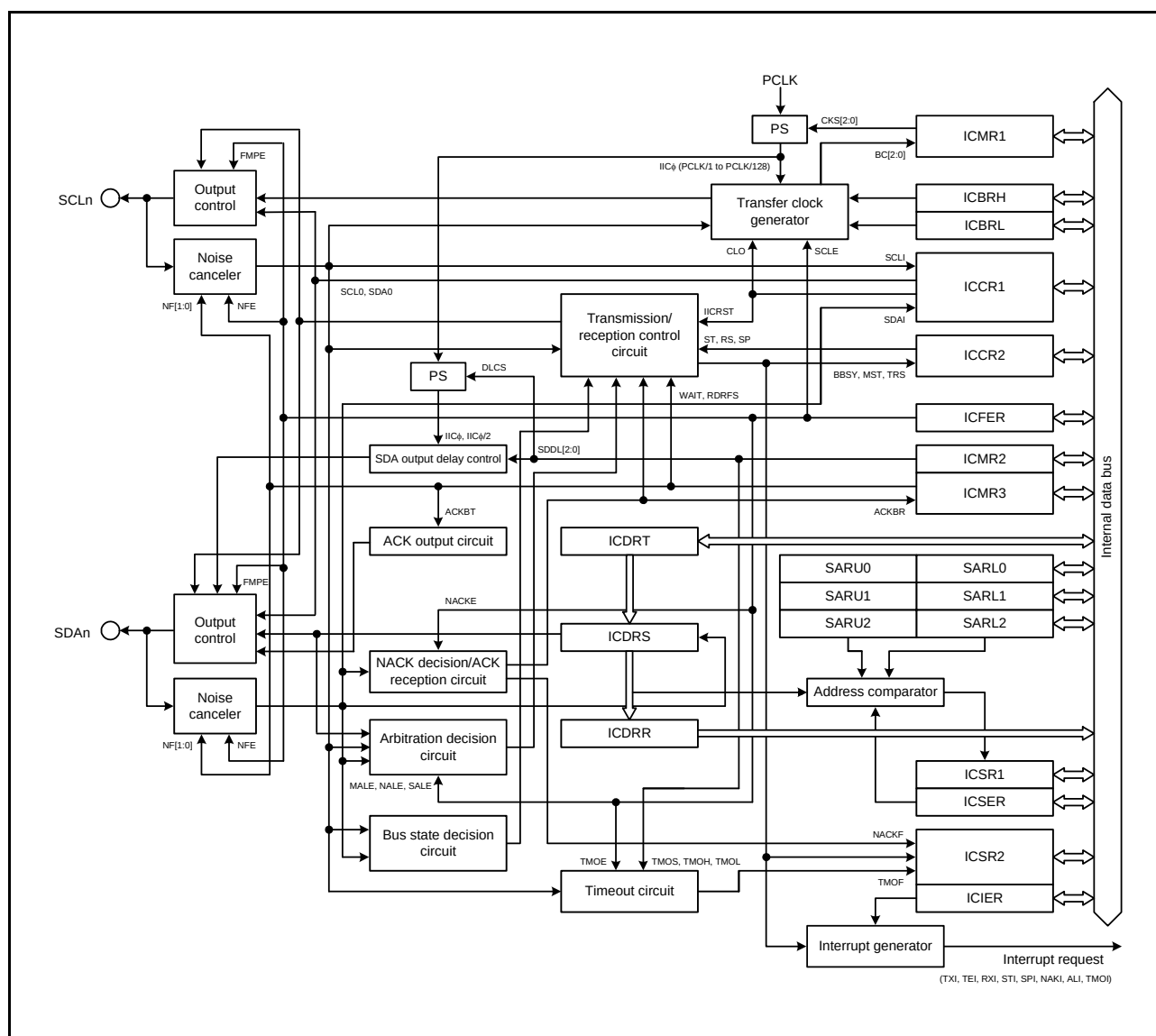
Figure 33.1 Block Diagram of RIIC
