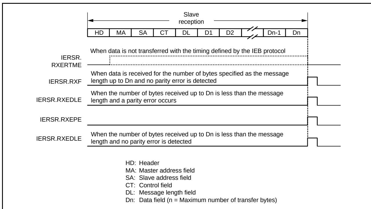
Figure 36.17 Timing of Operations when Reception is Not Completed within Maximum Number of Transfer Bytes
