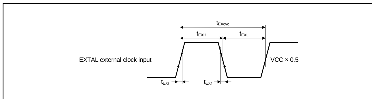
Figure 45.4 EXTAL External Clock Input Timing
