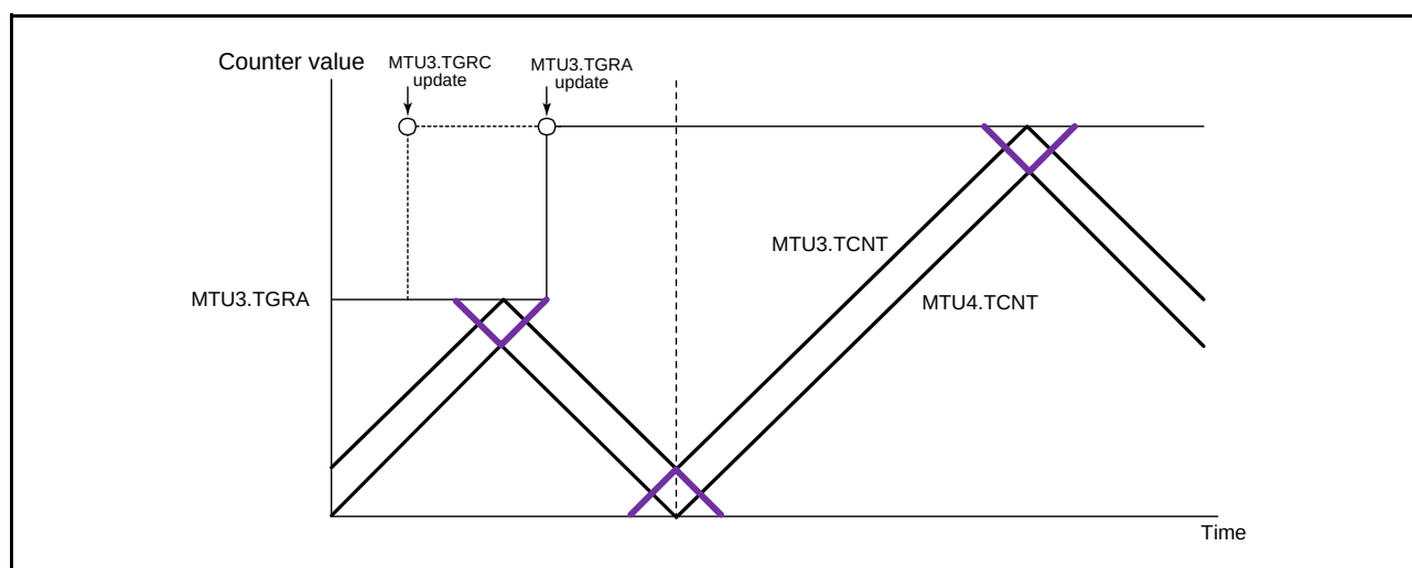
Figure 22.42 Example of PWM Cycle Updating
