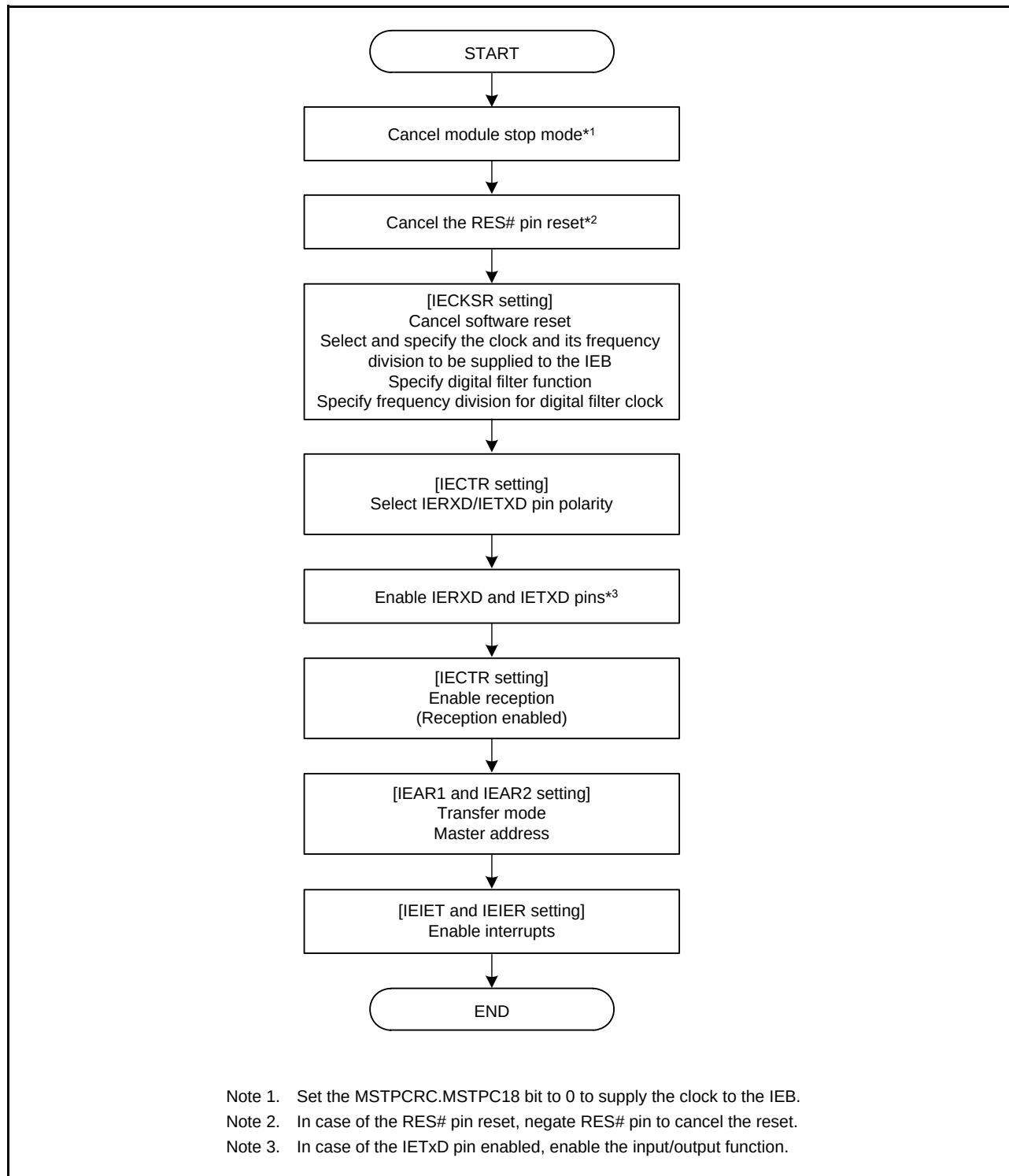
Figure 36.6 Flowchart for Initial Setting
