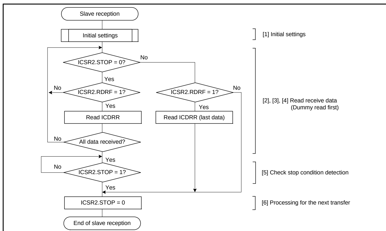
Figure 33.17 Example of Slave Reception Flowchart
