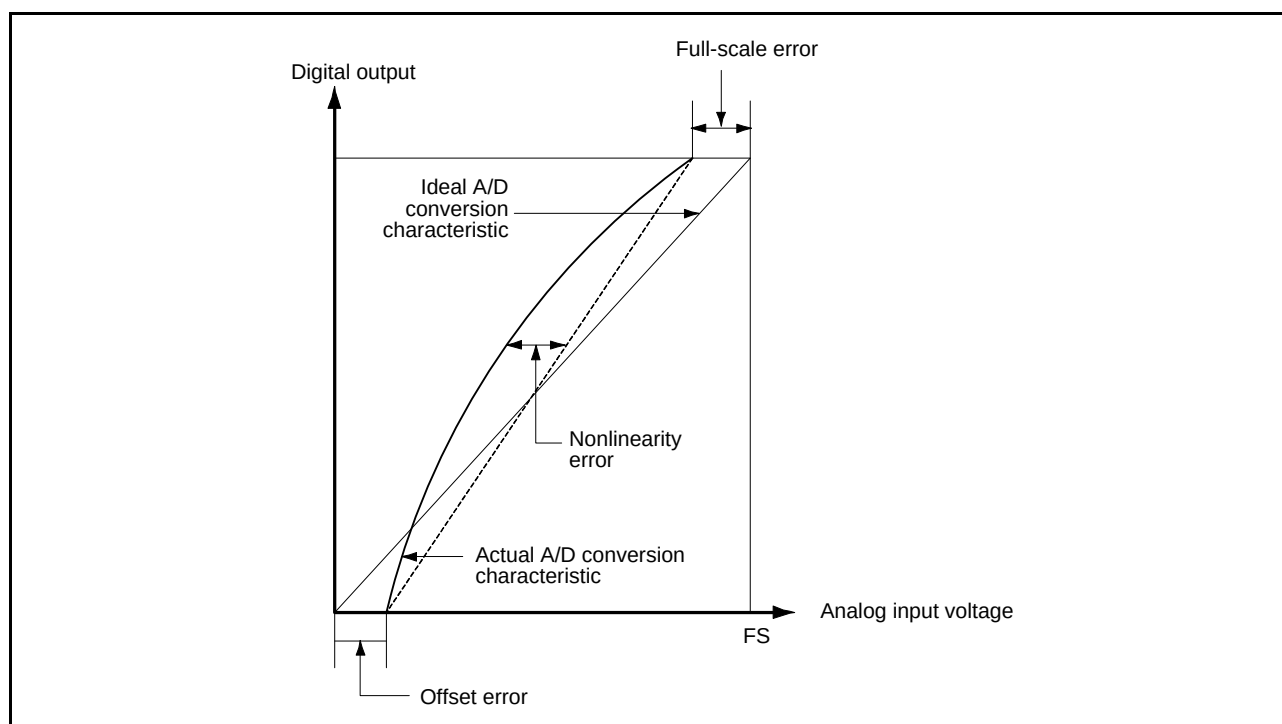
Figure 39.15 A/D Conversion Accuracy Definitions (2)
