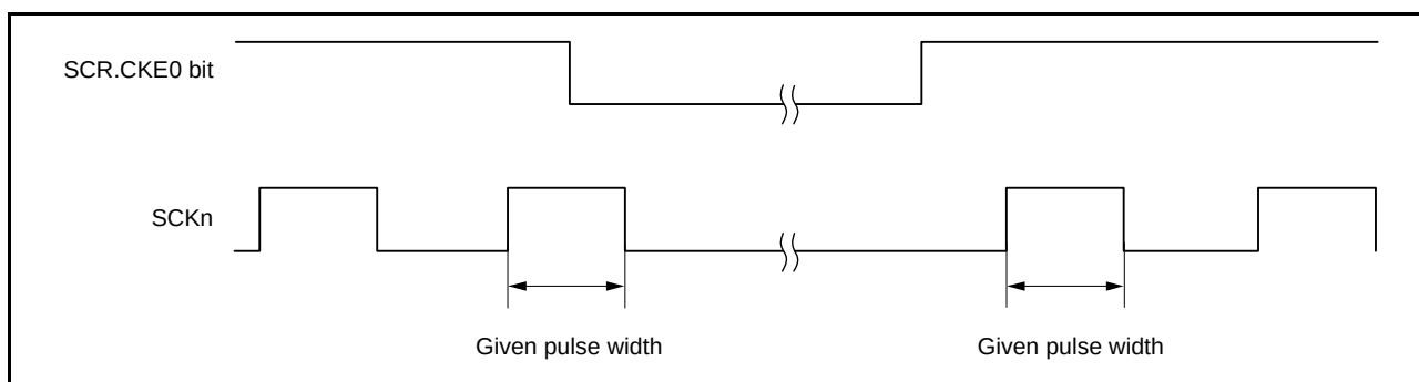
Figure 32.38 Clock Output Fixing Timing
