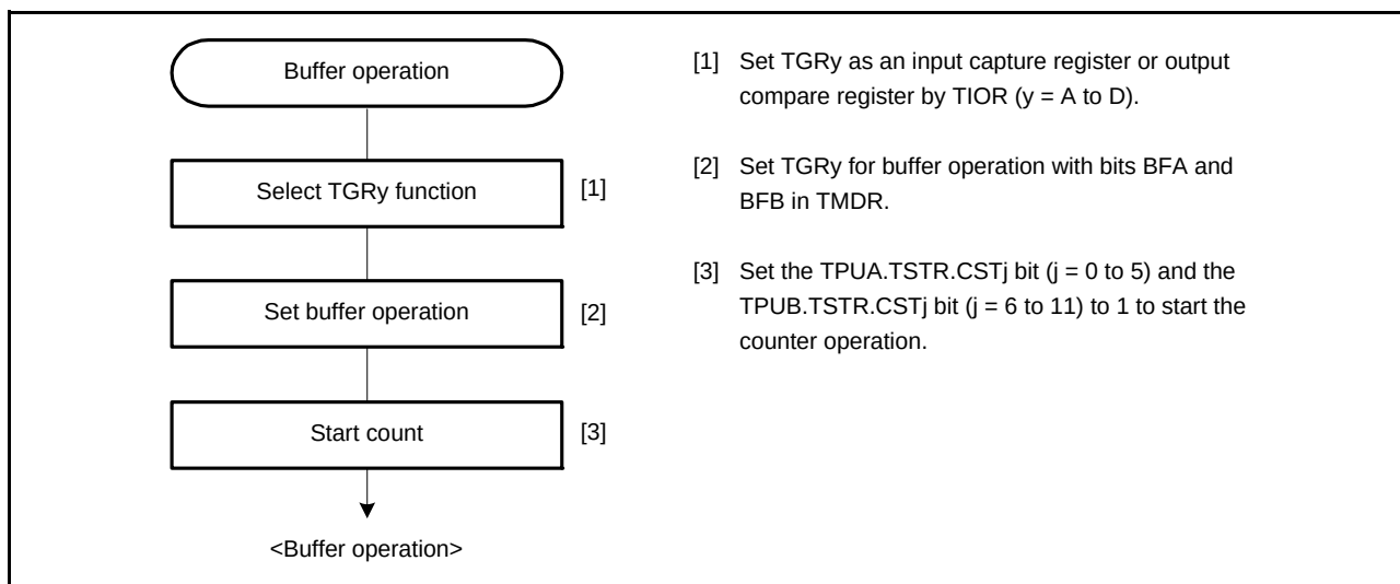
Figure 24.15 Example of Buffer Operation Setting Procedure
