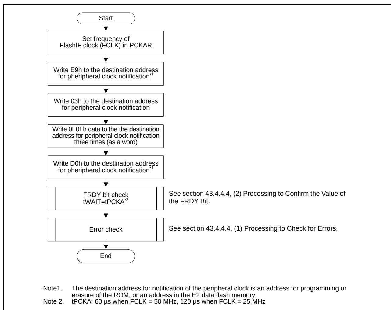
Figure 43.12 Using the Peripheral Clock Notification Command
