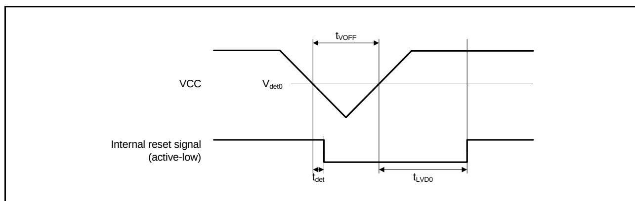
Figure 45.41 Voltage Detection Circuit Timing ( V_{det0} )
