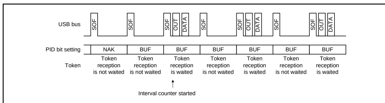
Figure 31.14 Relationship between Frames and Expected Token Reception when IITV ≠ 0
