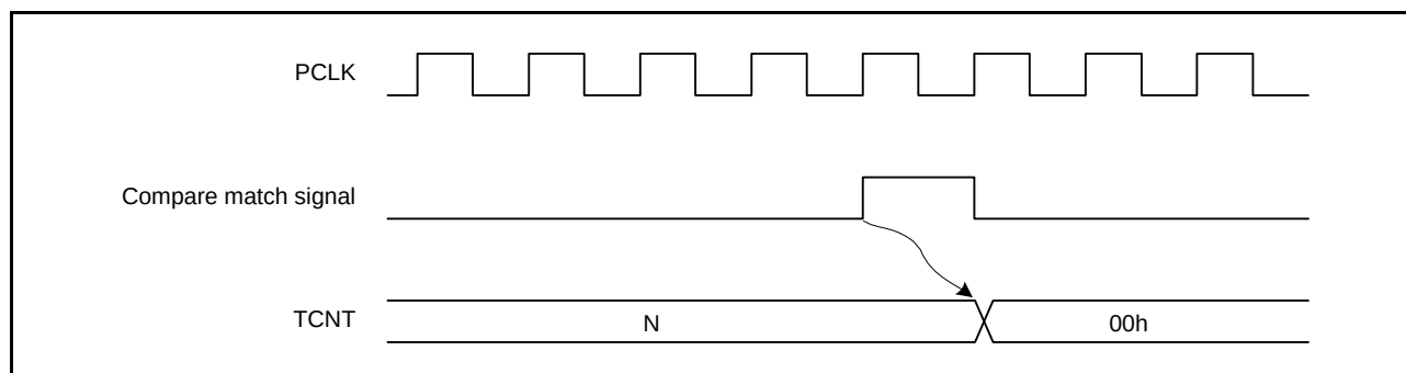
Figure 26.9 Timing of Counter Clear by Compare Match
