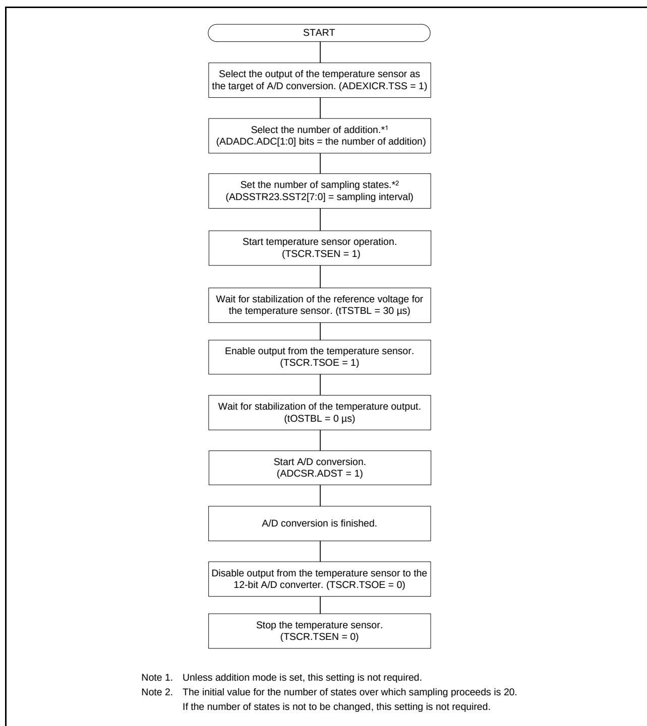
Figure 41.2 Procedure for Using the Temperature Sensor
