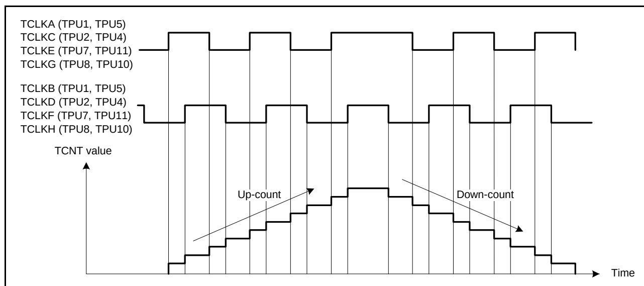
Figure 24.26 Example of Phase Counting Mode 1 Operation
