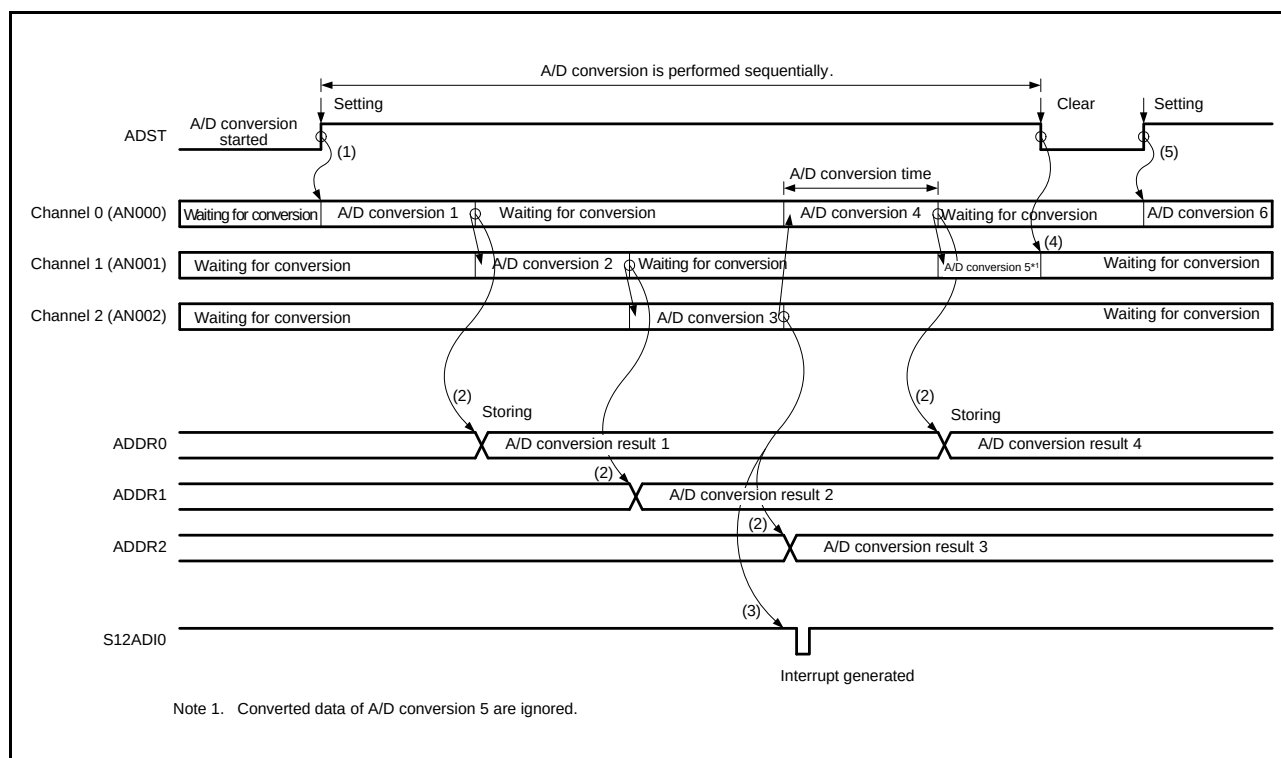
Figure 38.5 Example of Operation of Continuous Scan Mode (Basic Operation: AN000 to AN002 Selection)
