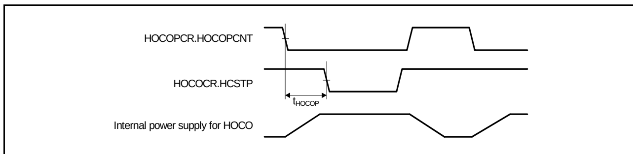
Figure 45.9 HOCO Power Supply Control Timing
