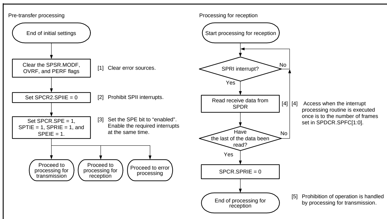
Figure 35.36 Flowchart in Master Mode (Reception)
