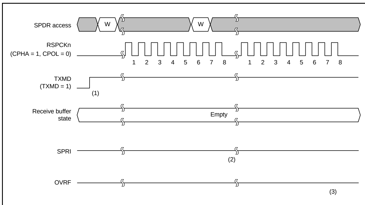
Figure 35.26 Operation Example of SPCR.TXMD = 1
