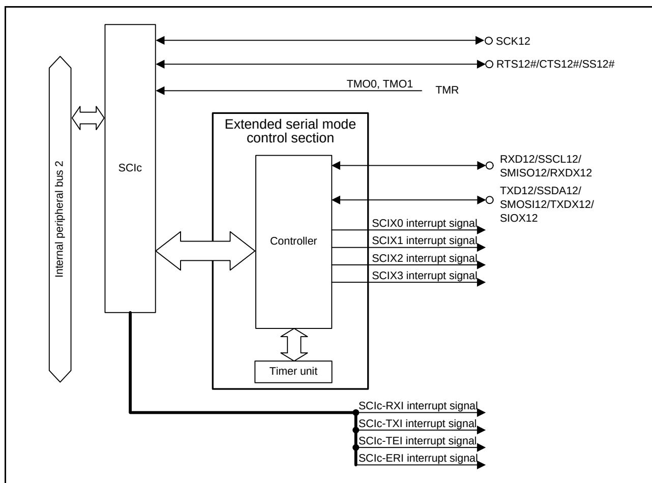
Figure 32.3 Block Diagram of SCI2 (SCId)
