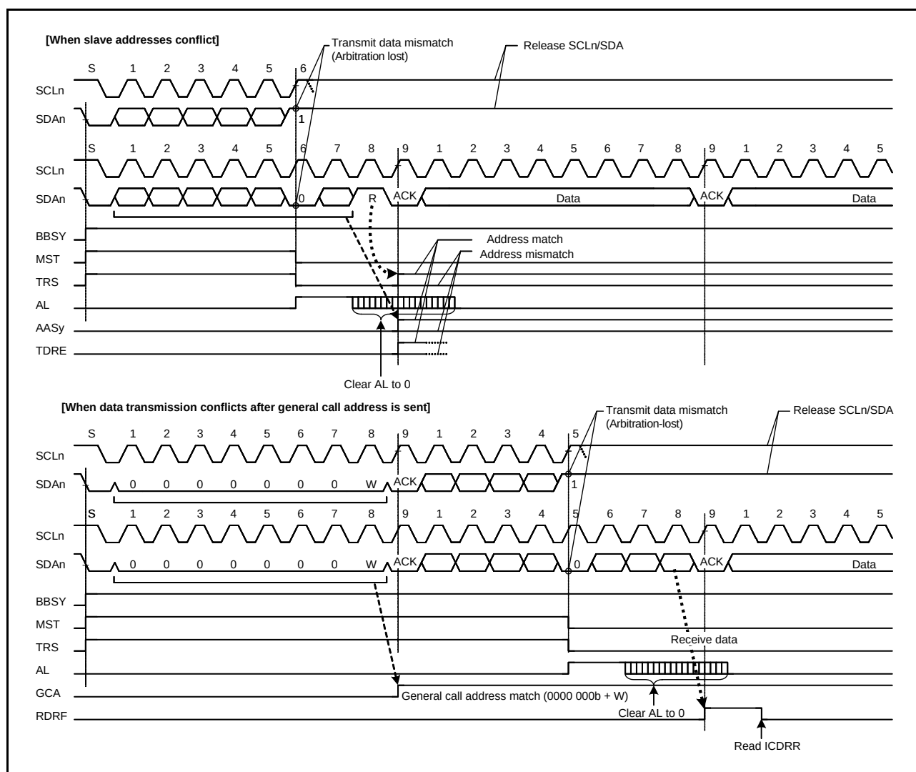
Figure 33.32 Examples of Master Arbitration-Lost Detection (MALE = 1)
