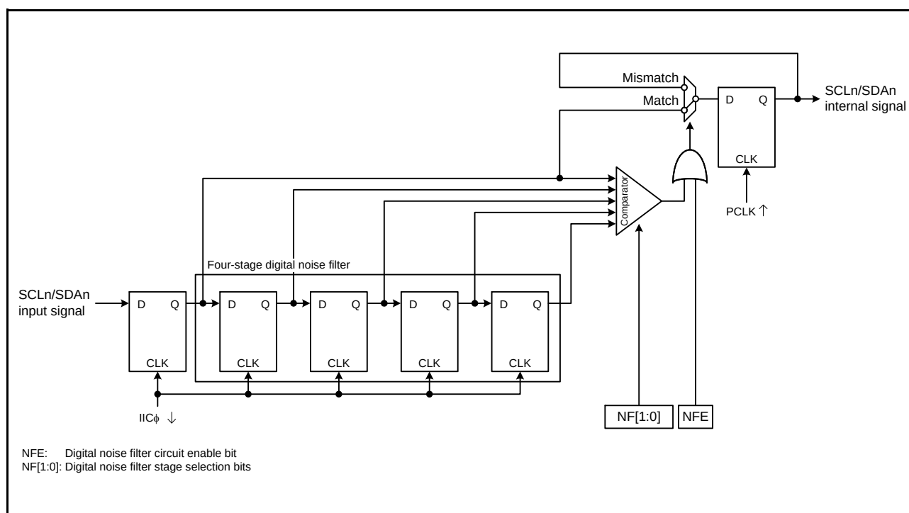
Figure 33.22 Block Diagram of Digital Noise Filter Circuit
