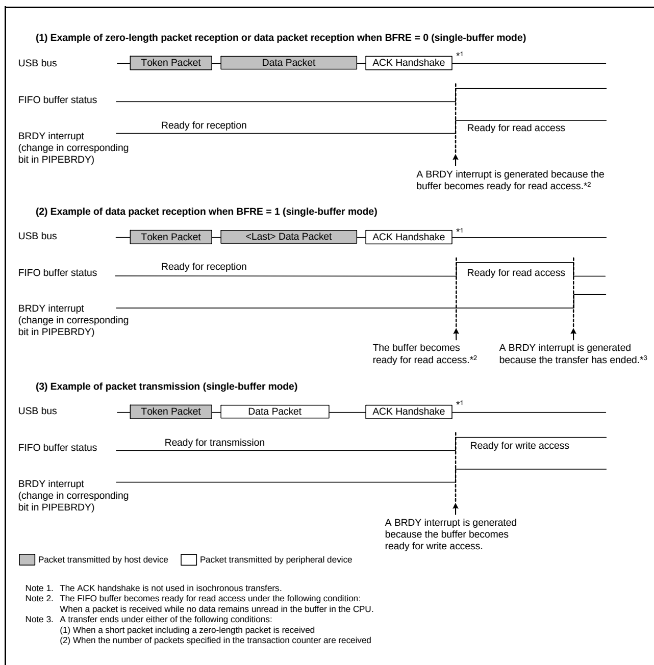
Figure 31.8 Timing of BRDY Interrupt Generation
