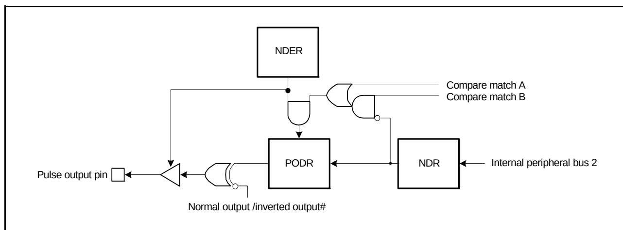
Figure 25.9 Non-Overlapping Pulse Output
