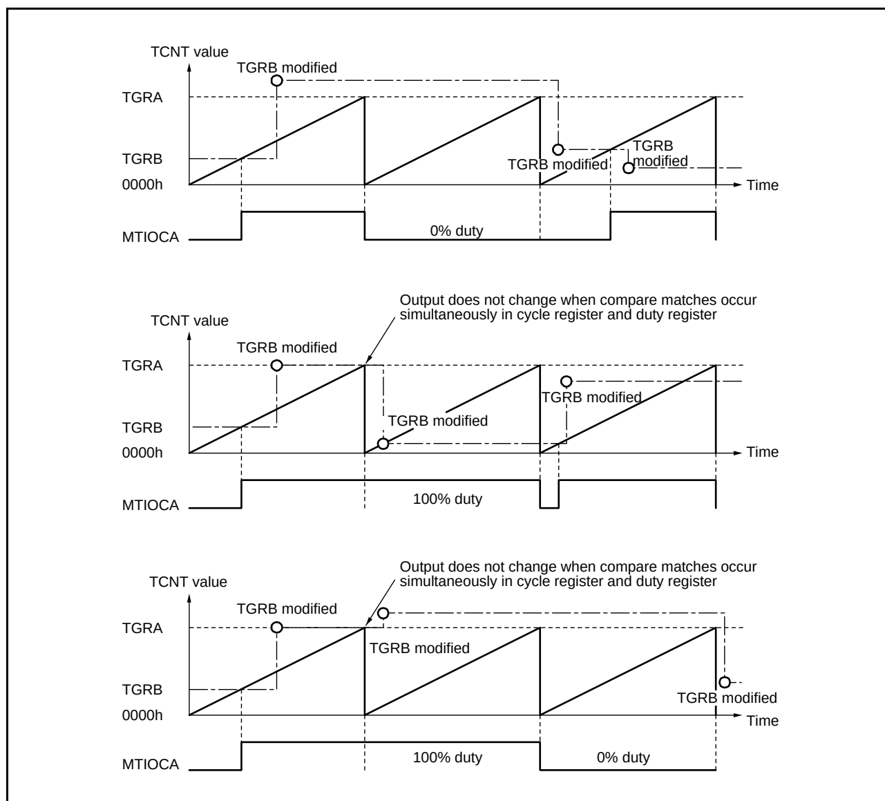
Figure 22.28 Examples of PWM Mode Operation
