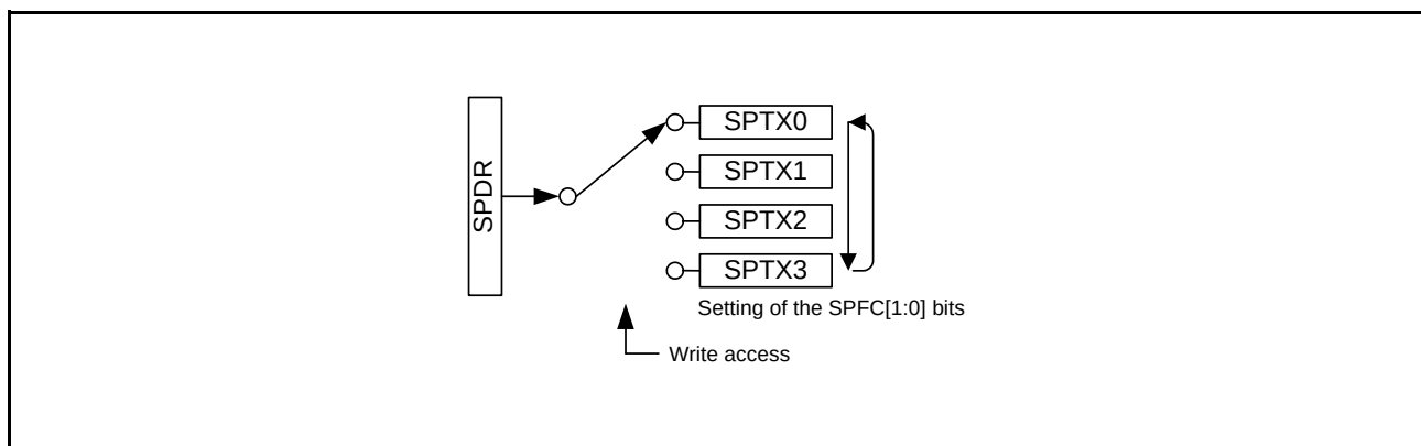
Figure 35.3 Configuration of SPDR (Writing)
