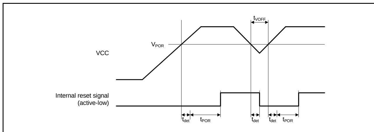
Figure 45.40 Power-on Reset Timing
