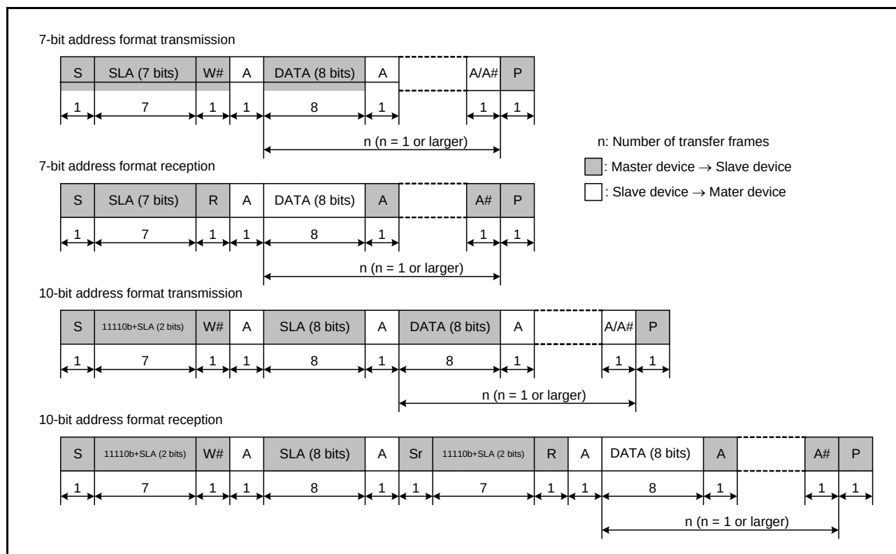
Figure 32.40 I 2 C Bus Master Format
