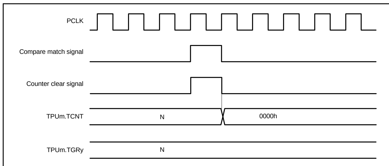
Figure 24.36 Counter Clear Timing (Compare Match)
