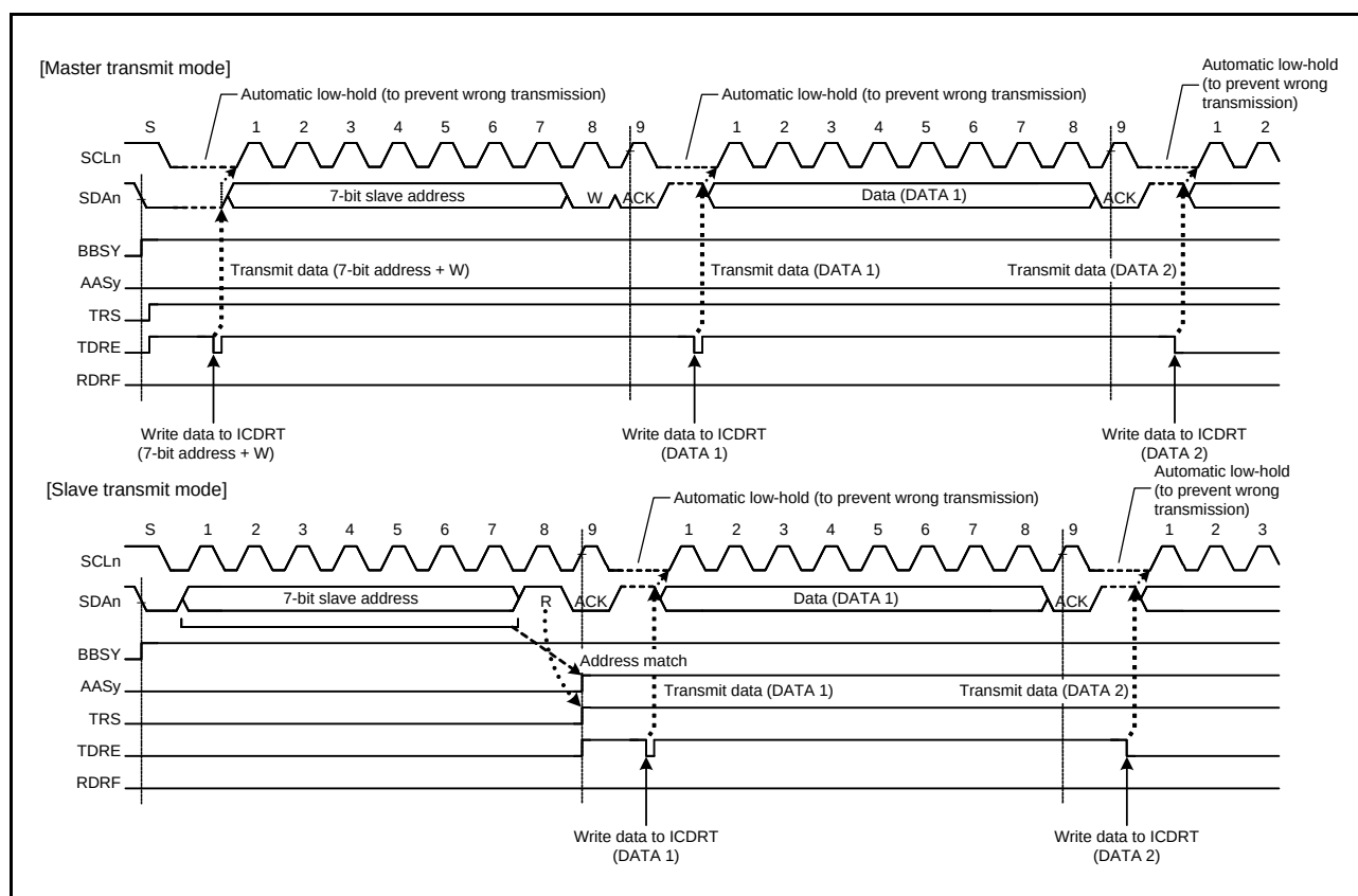
Figure 33.29 Automatic Low-Hold Operation in Transmit Mode
