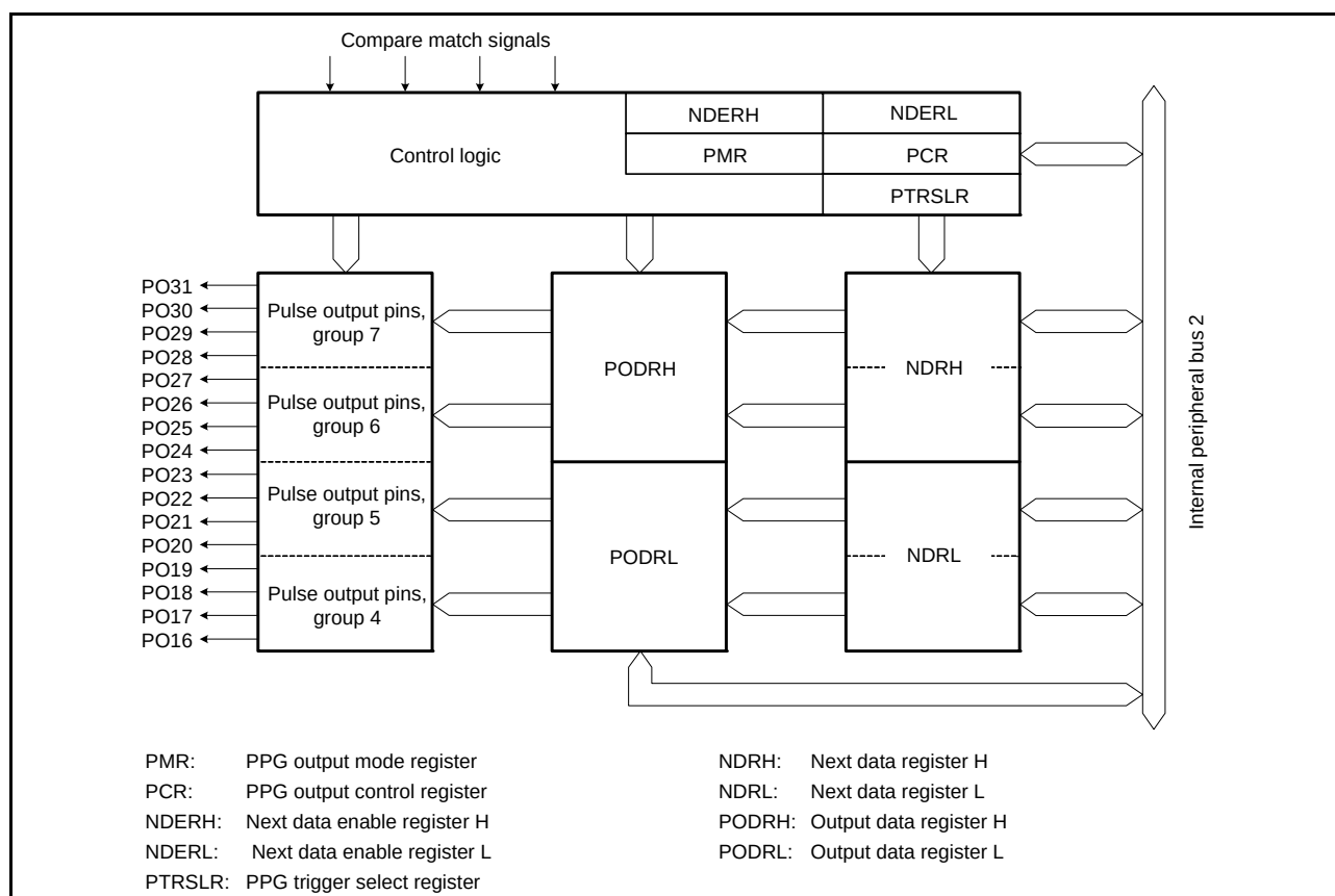
Figure 25.2 Block Diagram of PPG1
