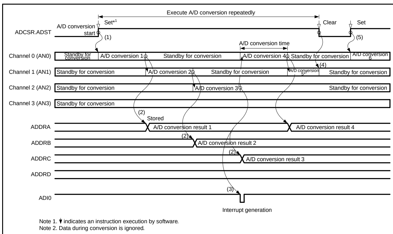
Figure 39.3 Example of 10-Bit A/D Converter Operation (Continuous Scan Mode)
