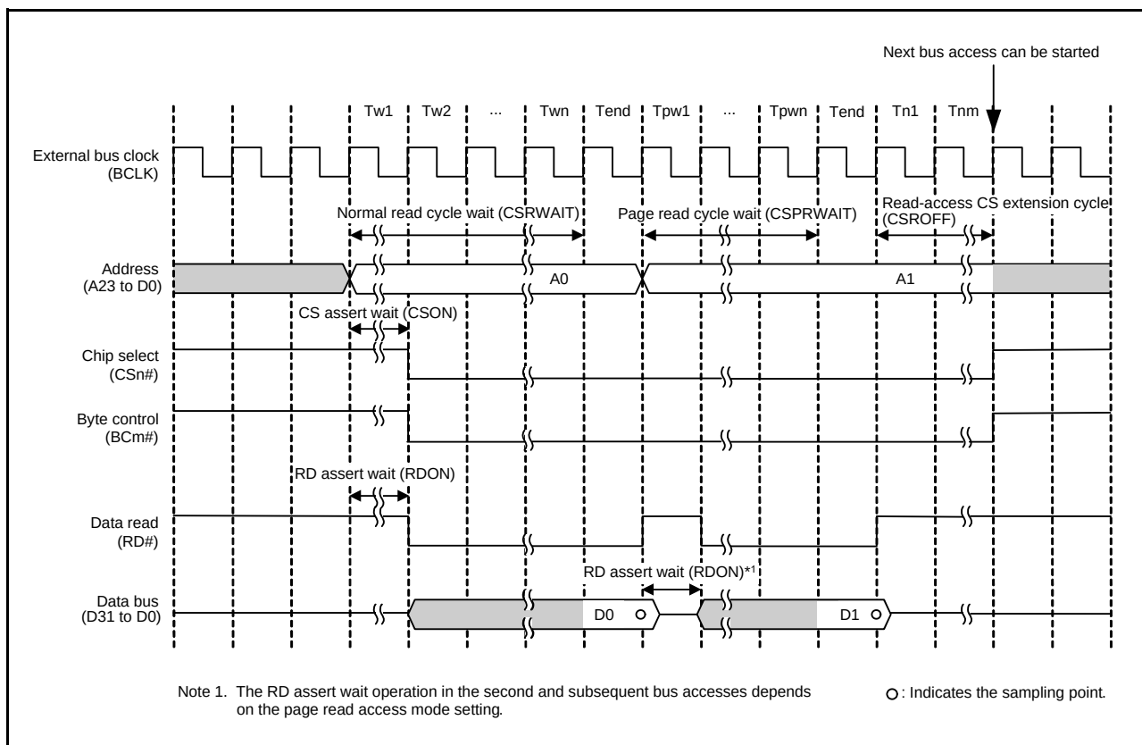
Figure 16.24 Page-Read Access Timing (n = 0 to 7, m = 0 to 3)
