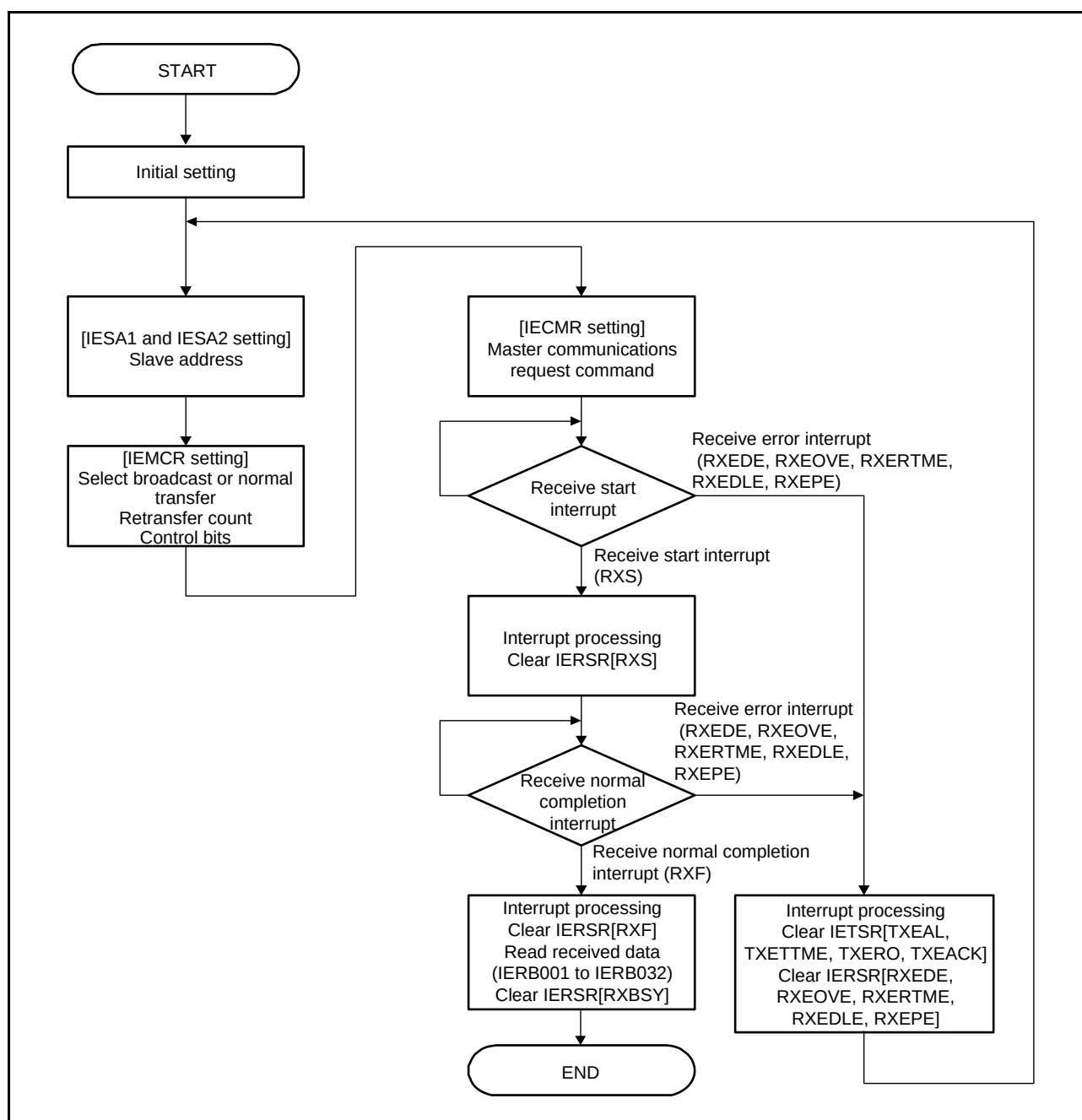
Figure 36.9 Flowchart for Master Reception
