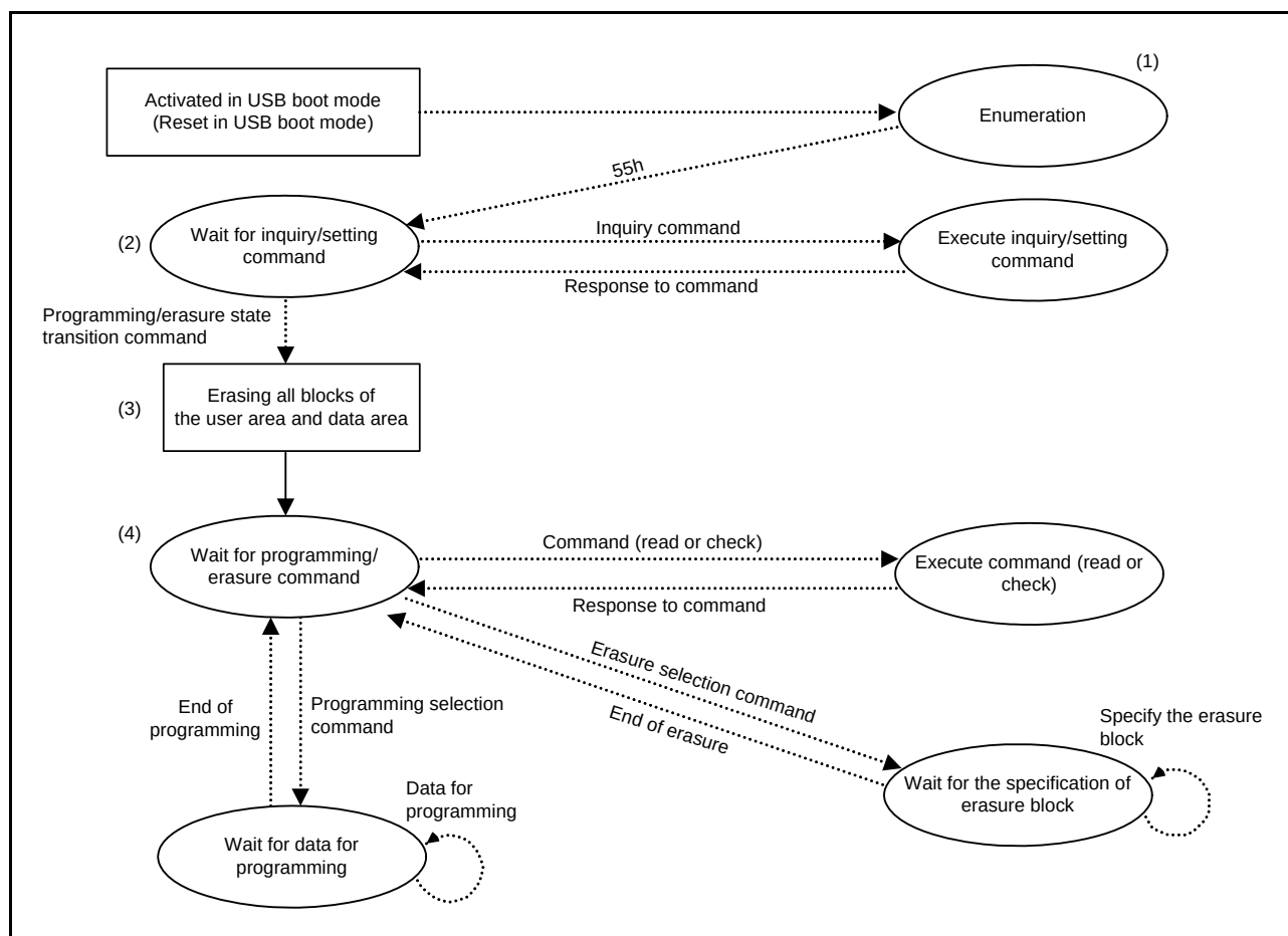
Figure 43.36 State Transitions in USB Boot Mode
