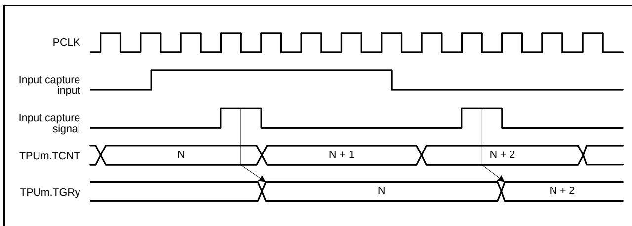
Figure 24.35 Input Capture Signal Timing
