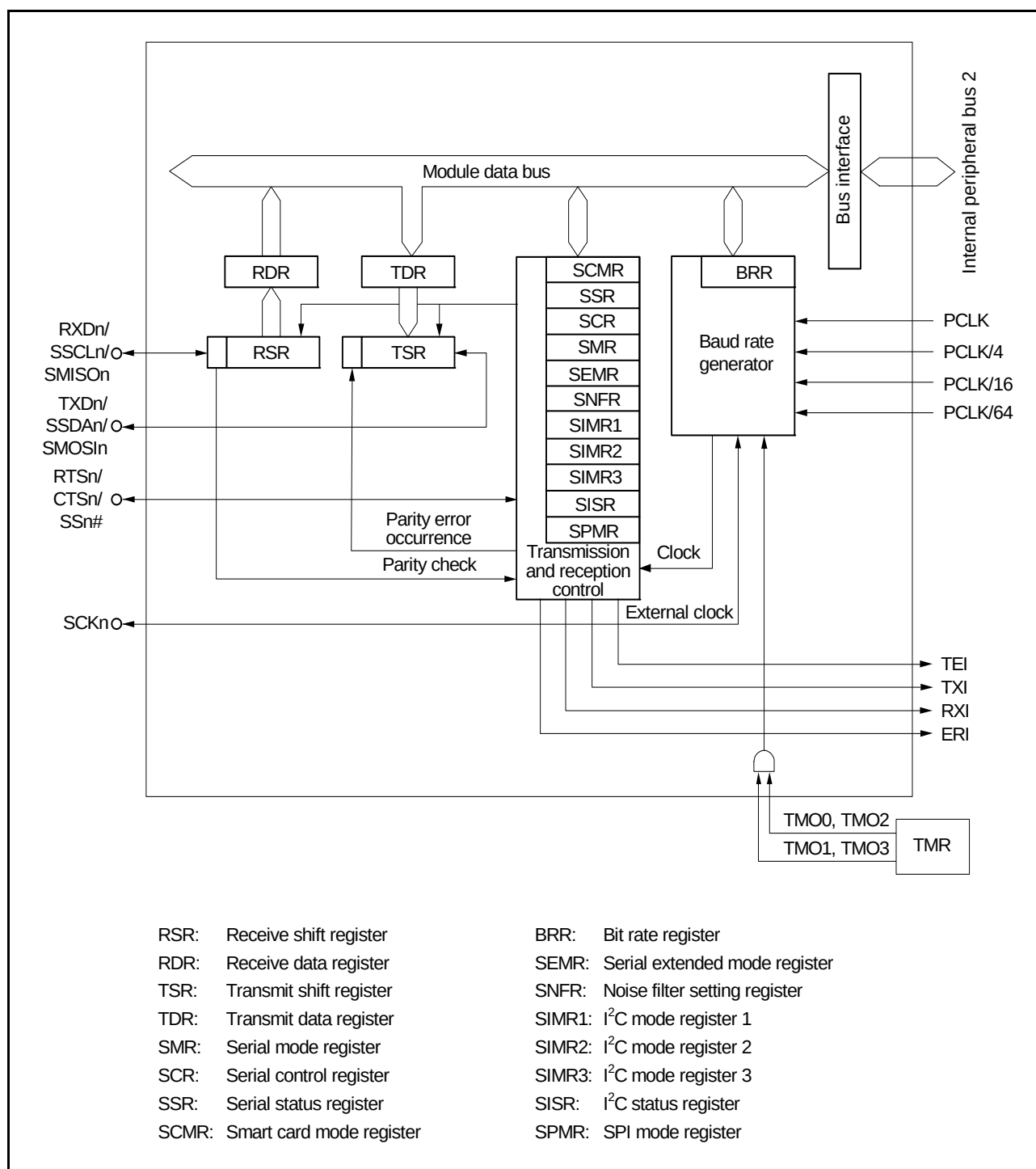
Figure 32.2 Block Diagram of SCI5 and SCI6
