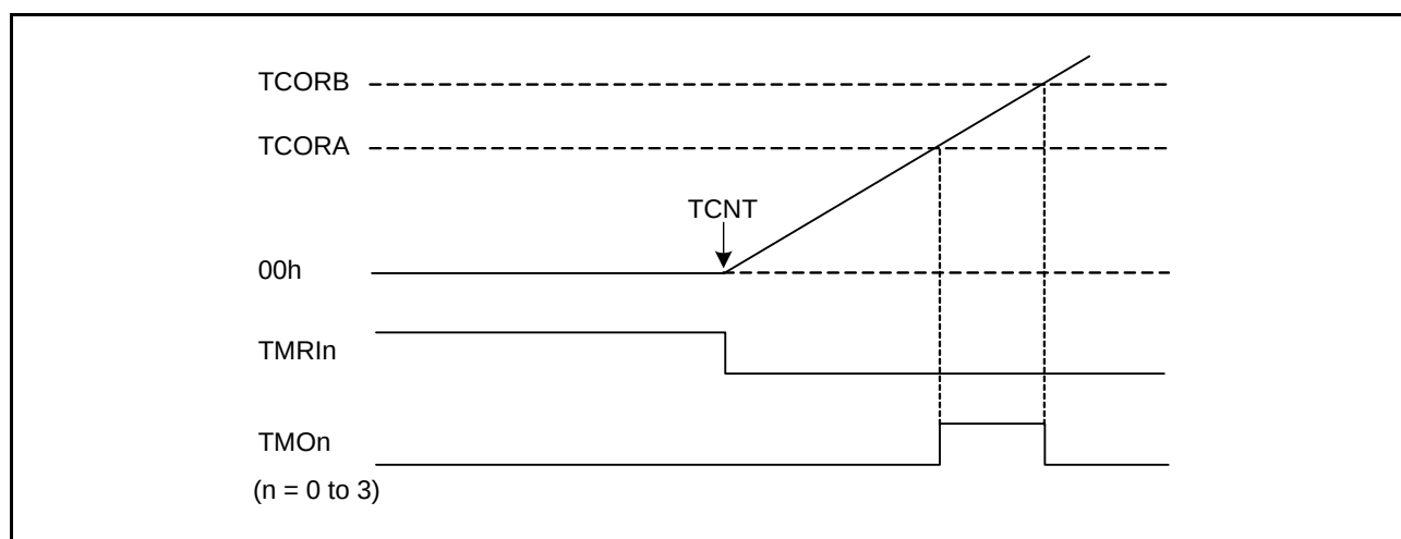
Figure 26.4 Example of Reset Input
