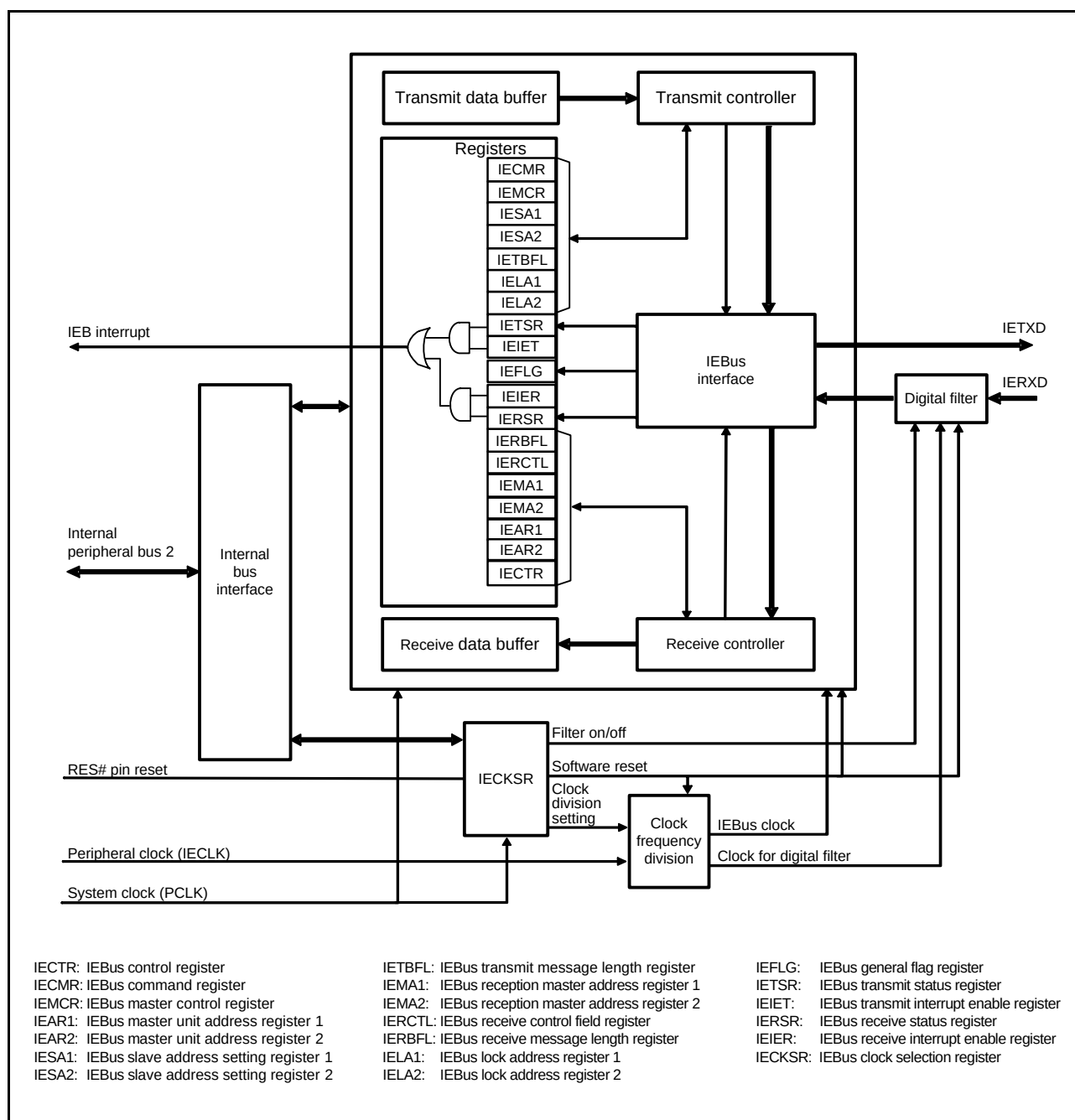
Figure 36.3 Block Diagram of IEB
