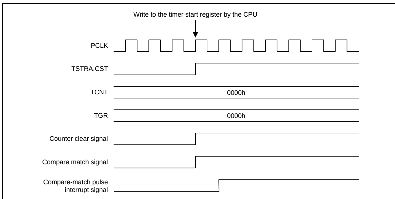
Figure 24.54 Continuous Output of Compare-Match Pulse Interrupt Signal
