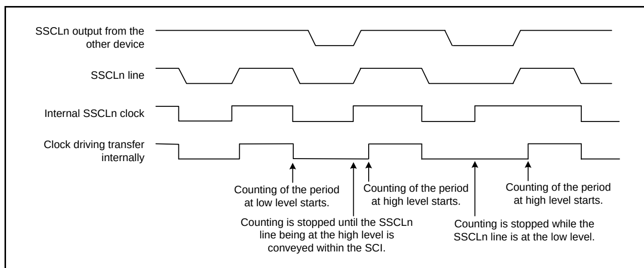
Figure 32.43 Example of Operations for Clock Synchronization
