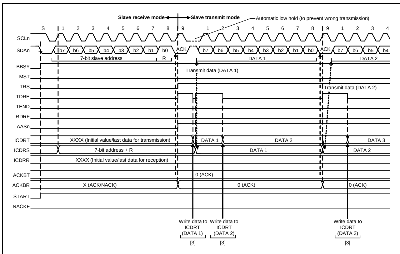
Figure 33.15 Slave Transmit Operation Timing (1) (7-Bit Address Format)
