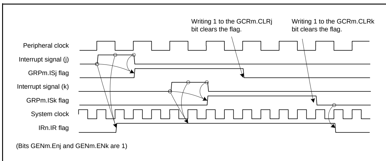
Figure 15.11 Operation Example in Which Multiple Edge Detection Interrupt Requests allocated to a Group are Generated
