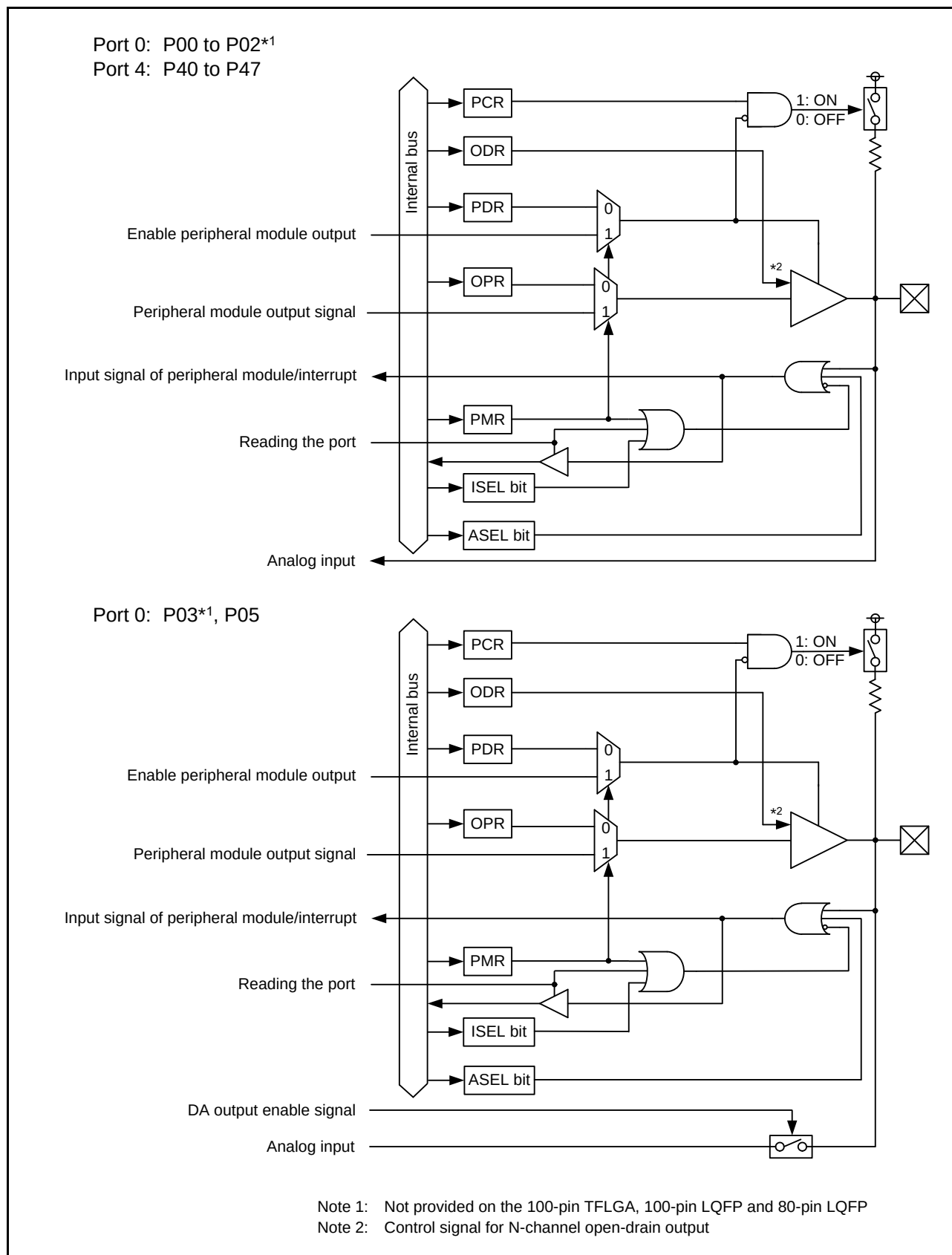
Figure 20.1 I/O Port Configuration (1)
