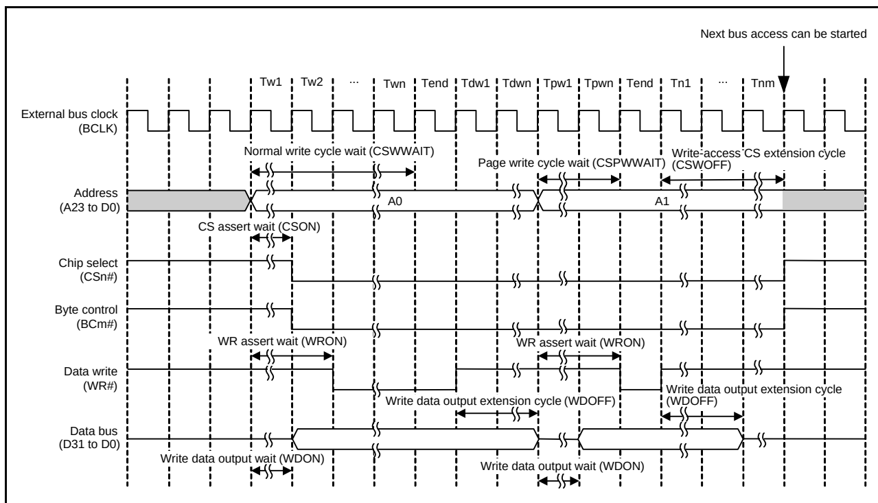
Figure 16.25 Page-Write Access Timing (n = 0 to 7, m = 0 to 3)
