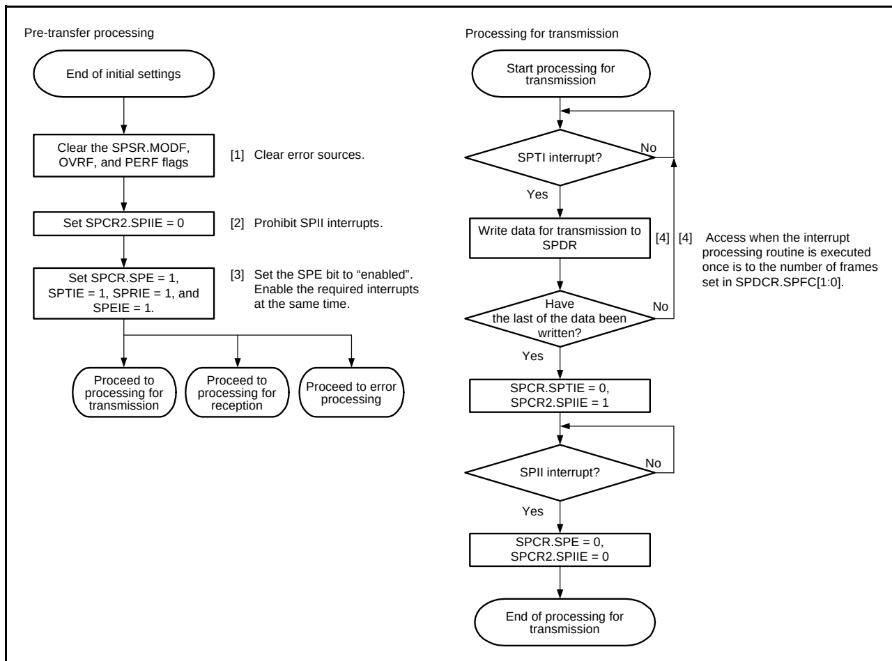
Figure 35.35 Flowchart in Master Mode (Transmission)
