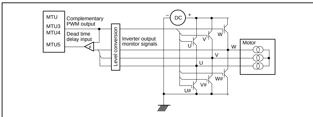
Figure 22.81 Example of Motor Control Circuit Configuration
