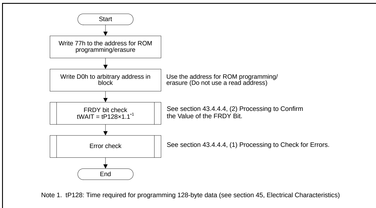
Figure 43.15 Procedure for Programming the Lock Bit
