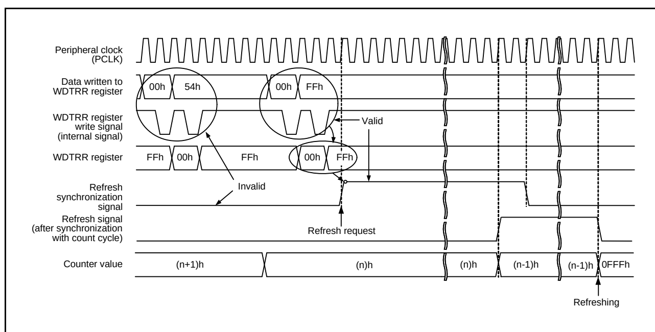
Figure 29.6 WDT Refresh Operation Waveforms (WDTCSR.CKS[3:0] = 0100b, WDTCSR.TOPS[1:0] = 01b)
