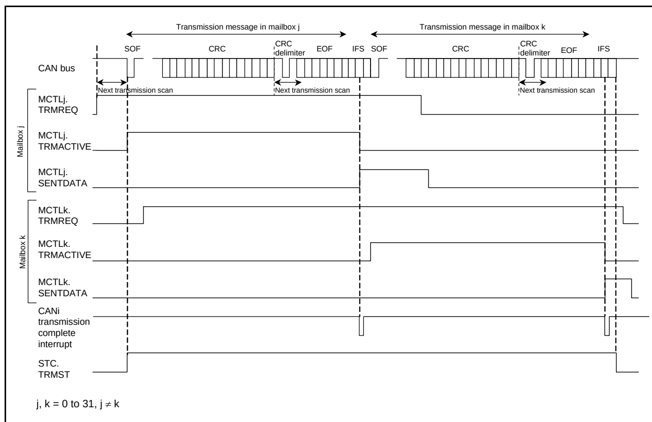
Figure 34.20 Operation Example of Data Frame Transmission
