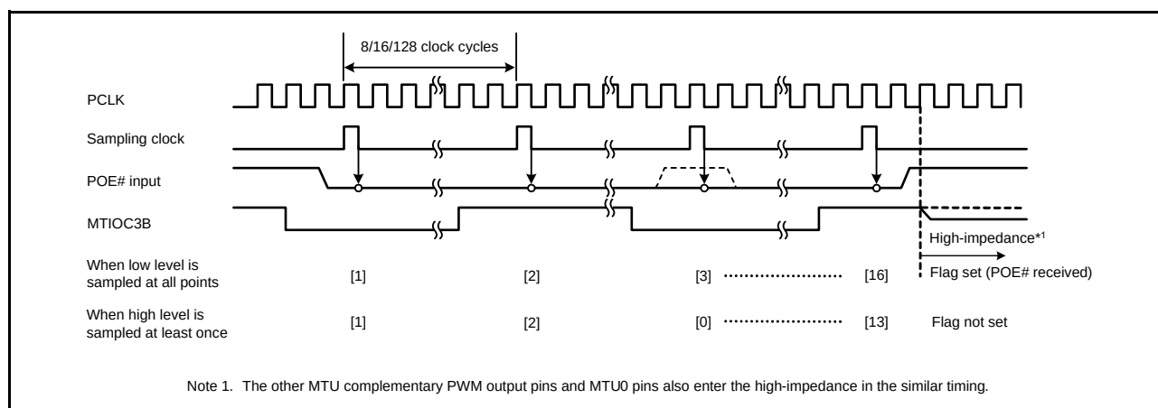
Figure 23.3 Low-Level Detection Operation
