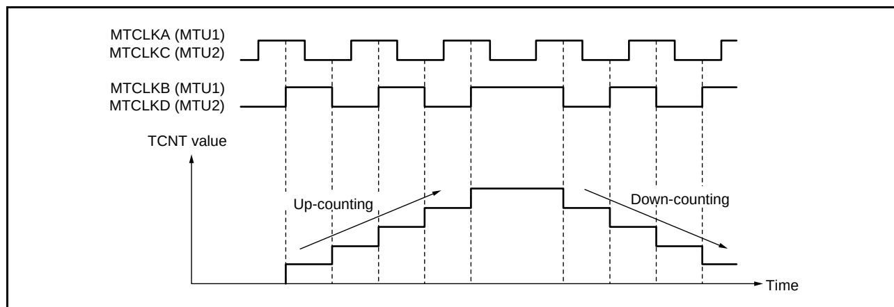
Figure 22.33 Example of Operation in Phase Counting Mode
