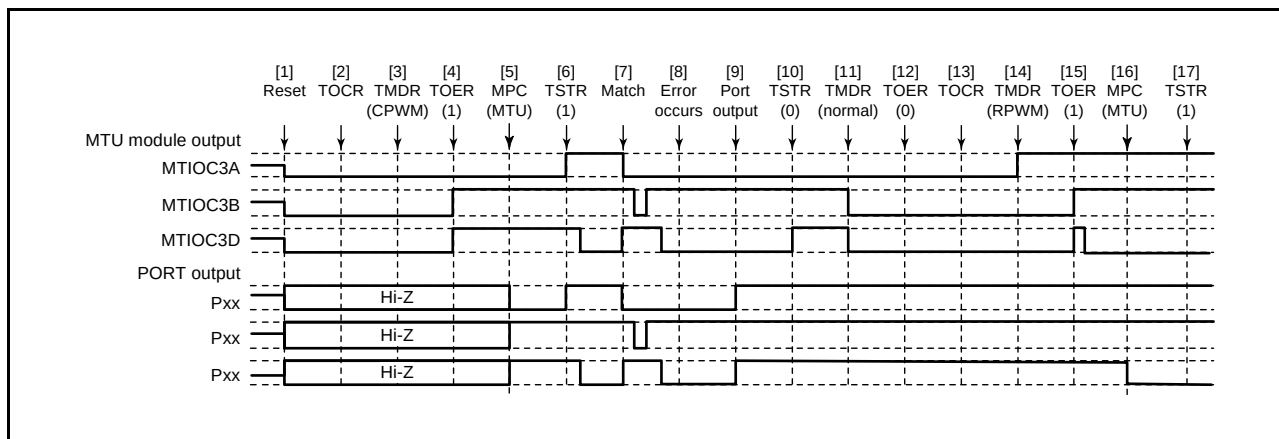
Figure 22.149 Error Occurrence in Complementary PWM Mode, Recovery in Reset-Synchronized PWM Mode
