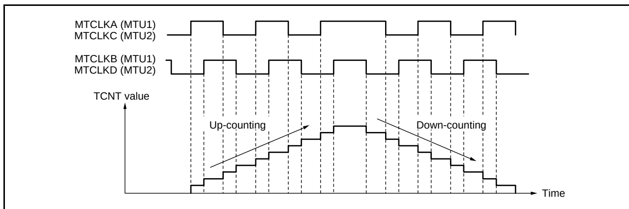
Figure 22.30 Example of Operation in Phase Counting Mode
