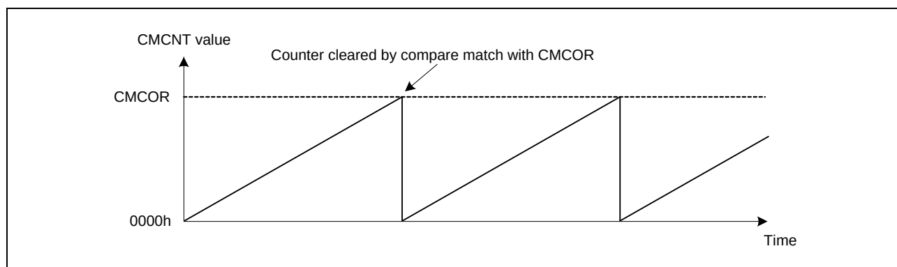
Figure 27.2 CMCNT Counter Operation
