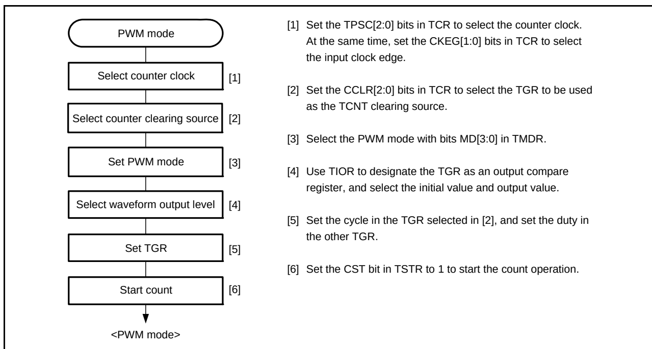
Figure 22.25 Example of PWM Mode Setting Procedure
