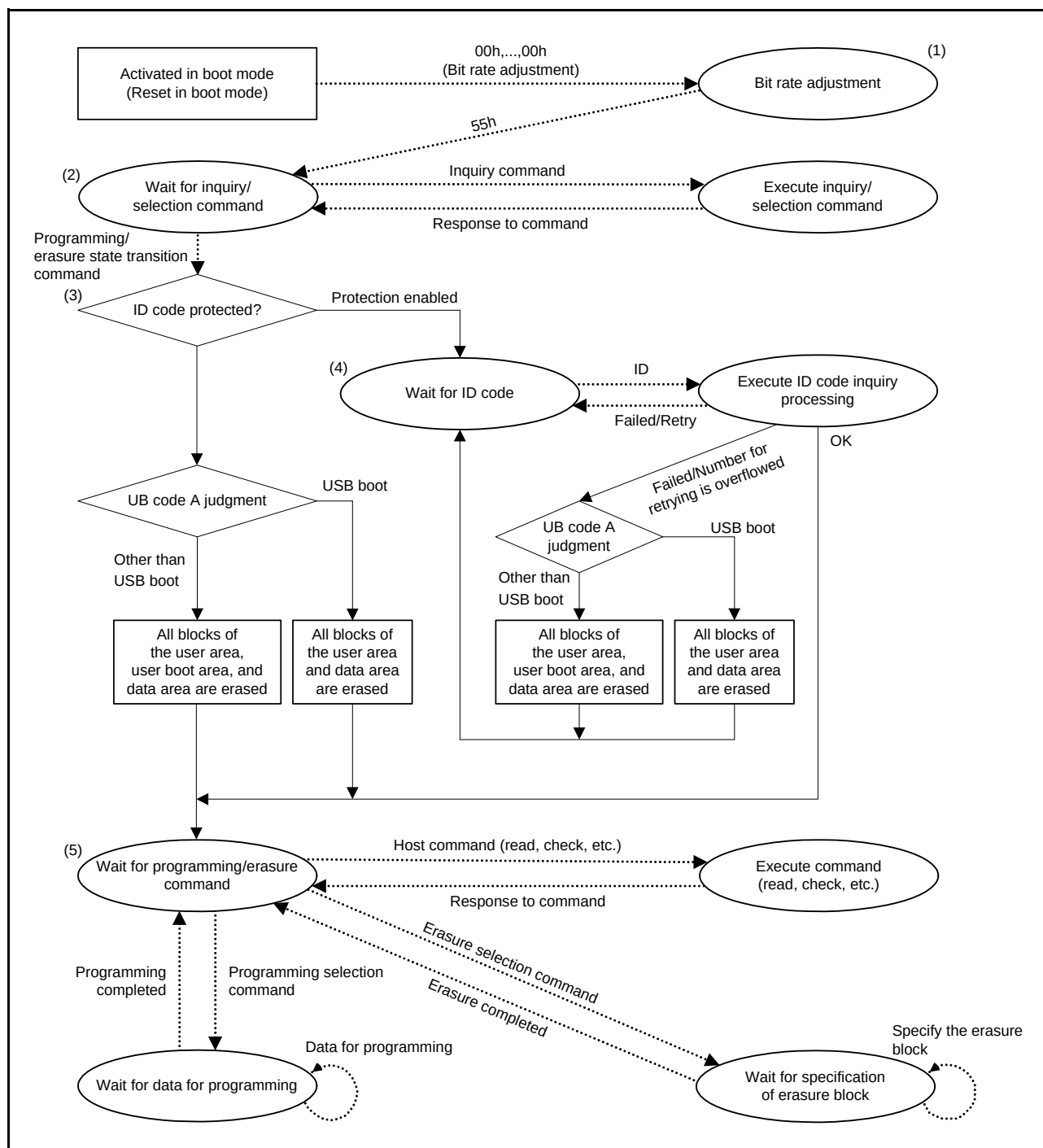
Figure 43.27 State Transitions in Boot Mode
