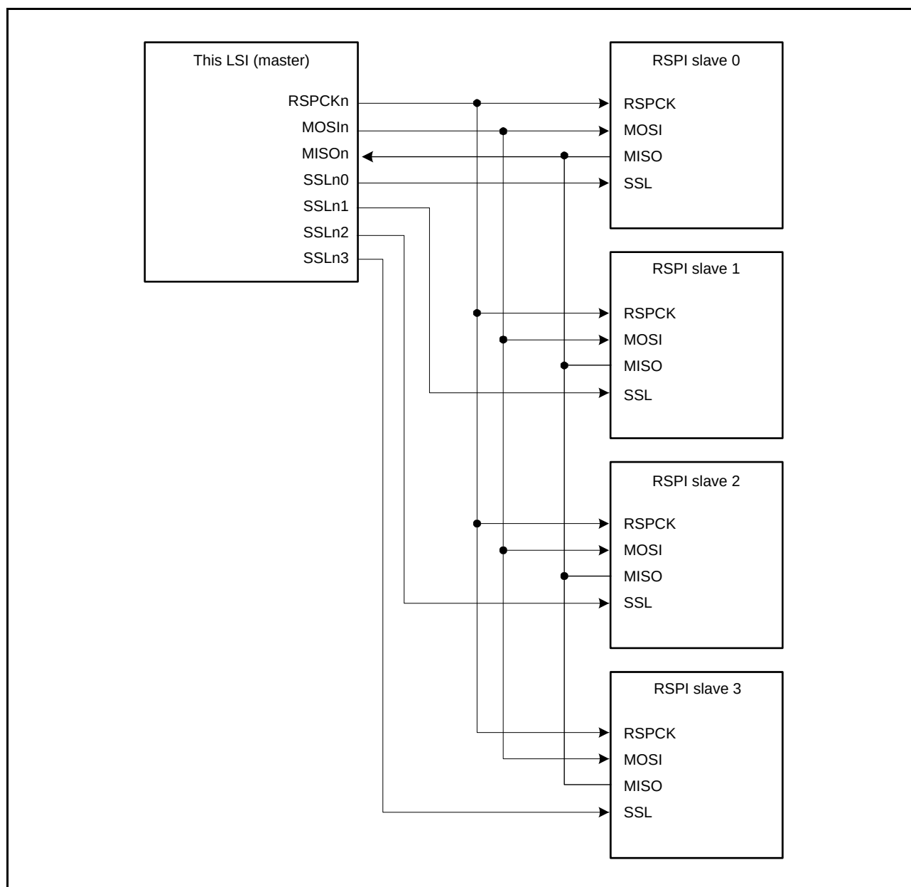
Figure 35.8 Single-Master/Multi-Slave Configuration Example (This LSI = Master)
