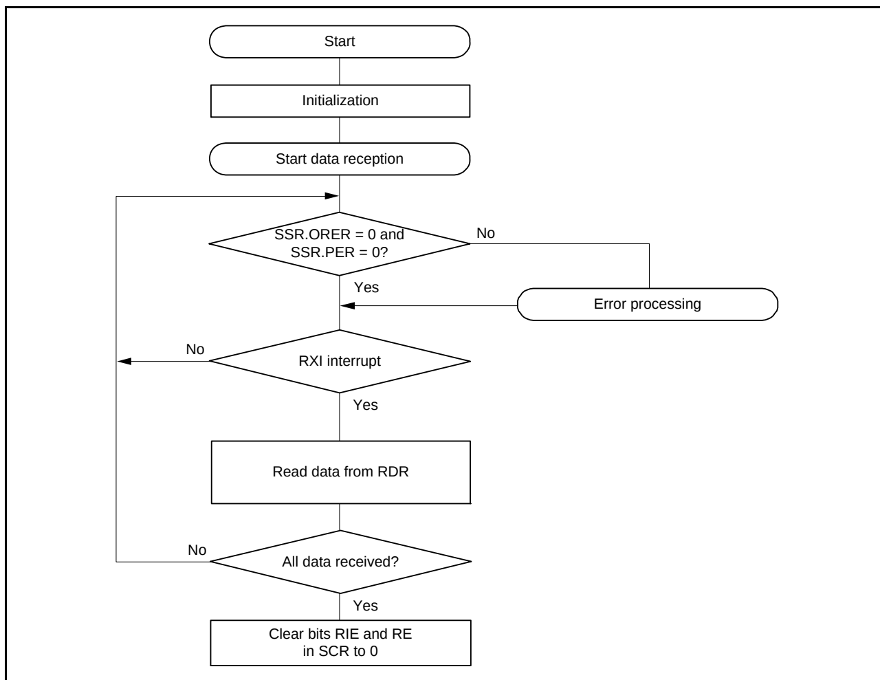
Figure 32.37 Sample Smart Card Interface Reception Flowchart
