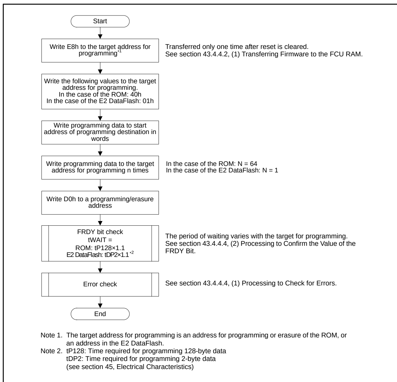
Figure 43.13 Procedure for ROM Programming
