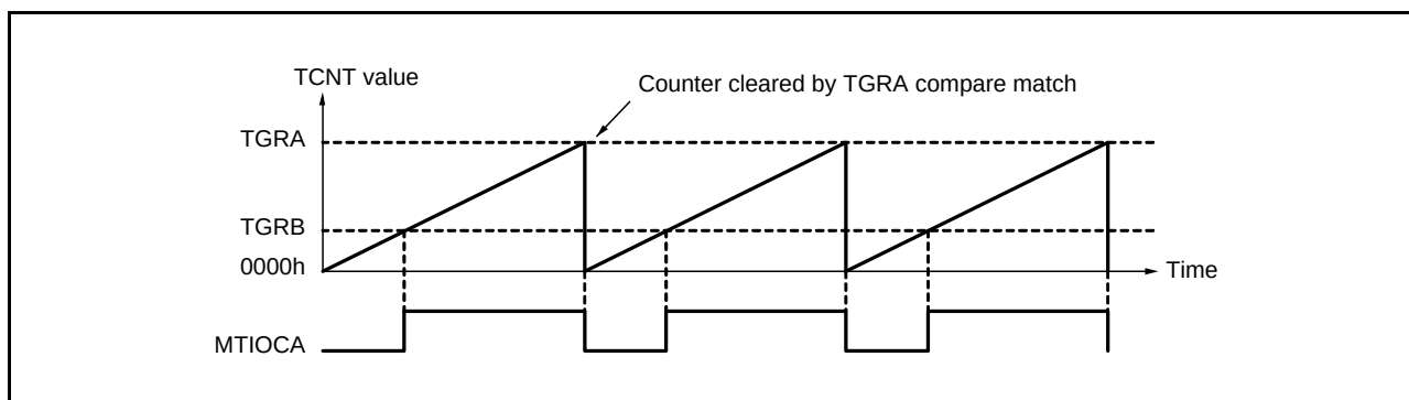
Figure 22.26 Example of PWM Mode Operation
