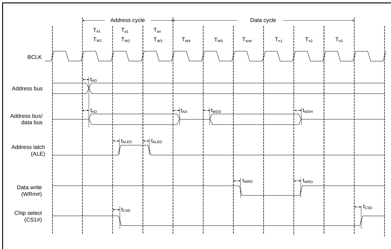
Figure 45.18 Address/Data Multiplexed Bus Write Access Timing
