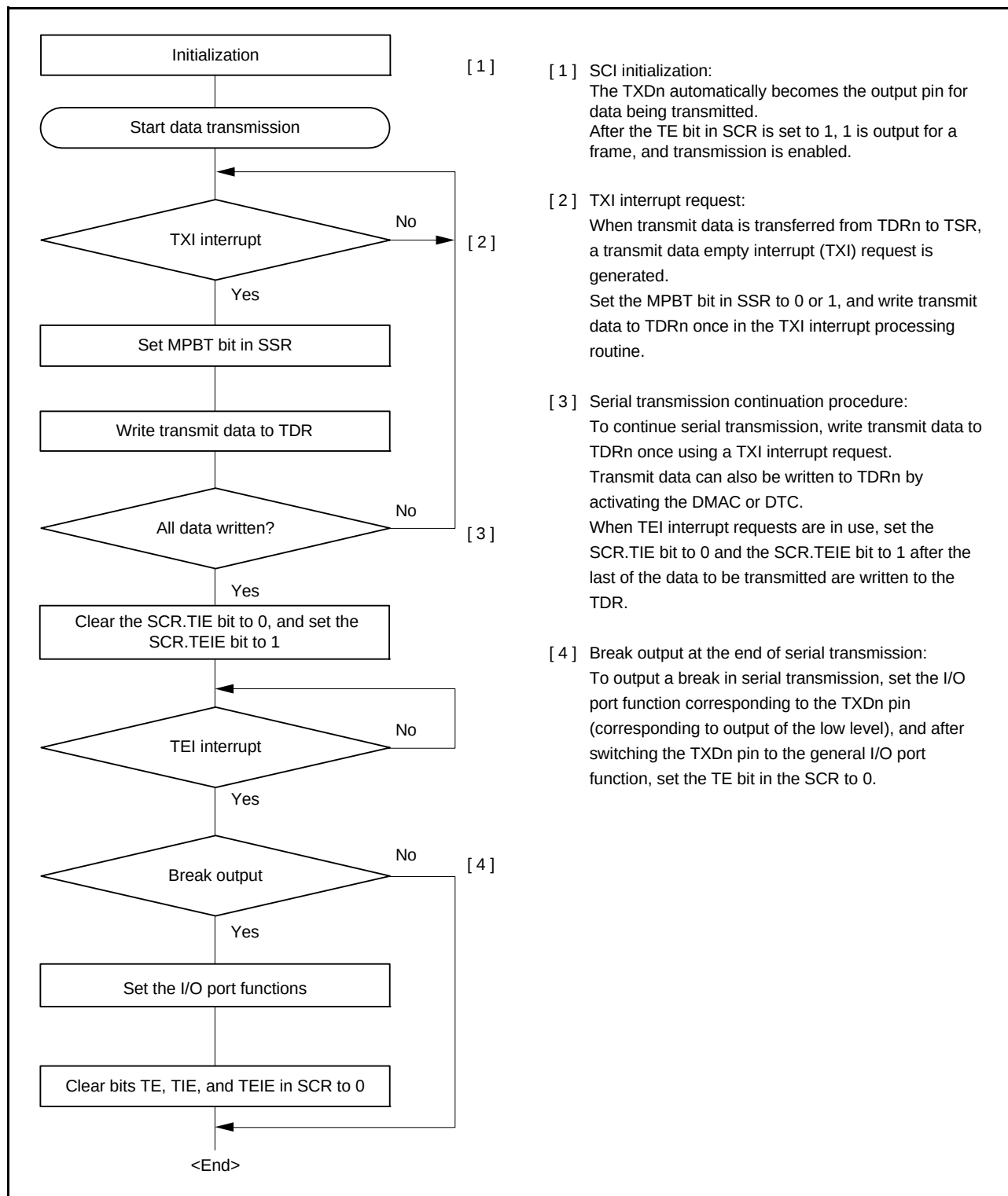
Figure 32.16 Example of Multi-Processor Serial Transmission Flowchart
