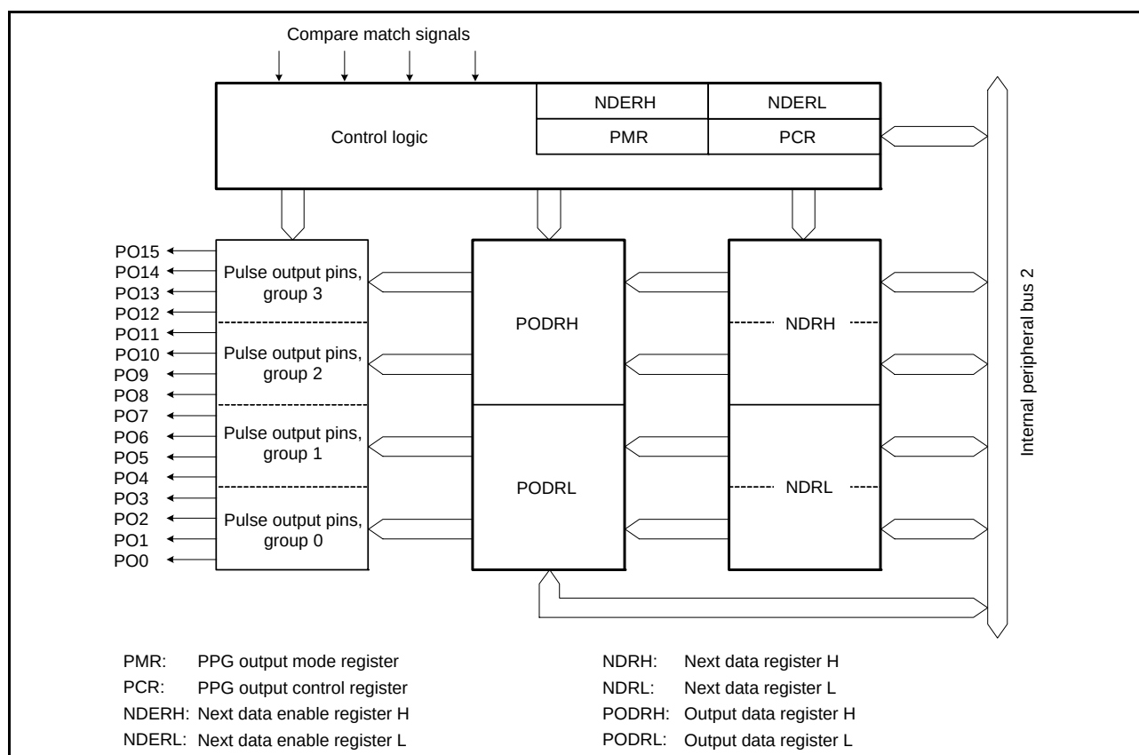
Figure 25.1 Block Diagram of PPG0
