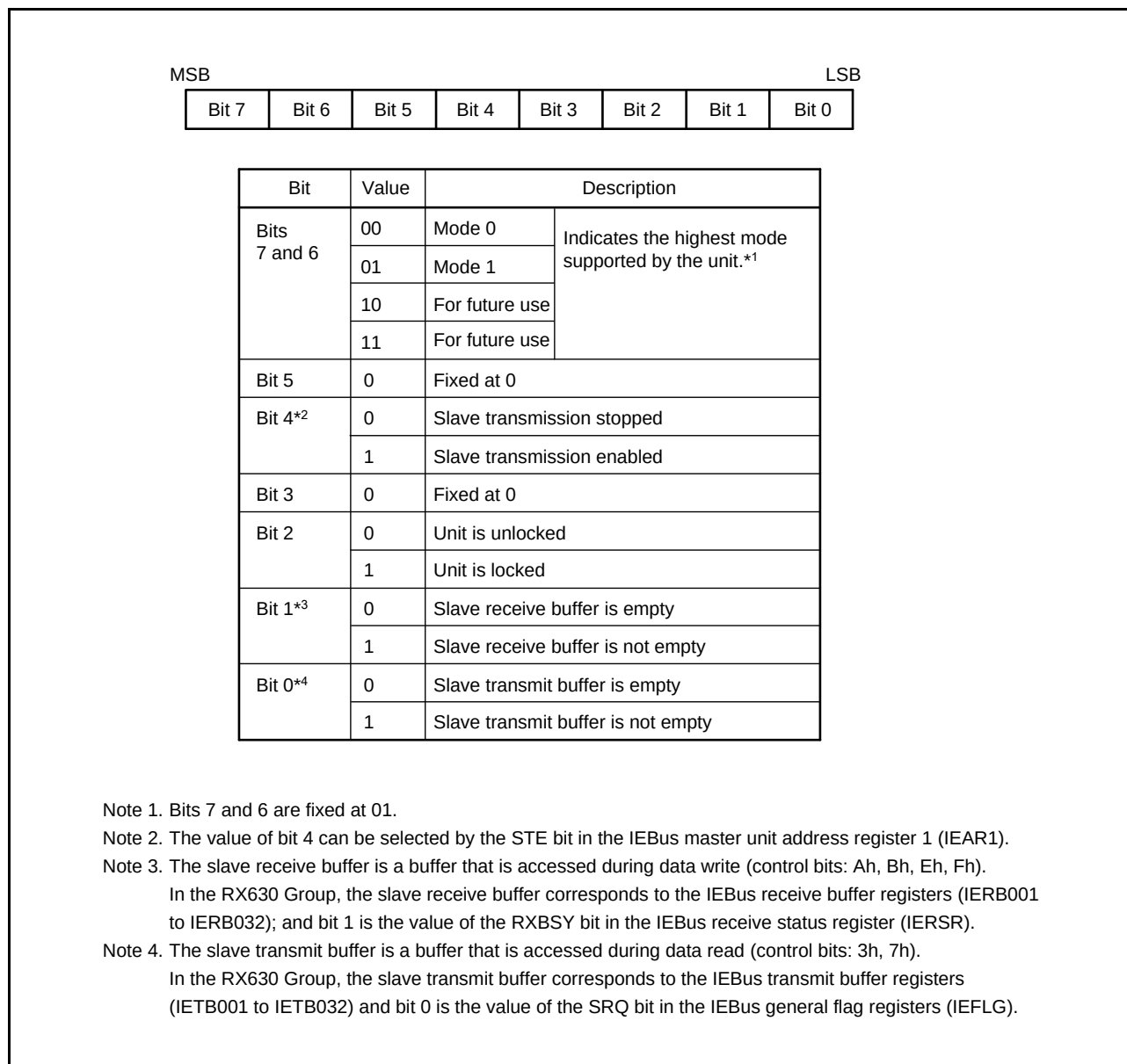
Figure 36.1 Bit Configuration of Slave Status (SSR)
