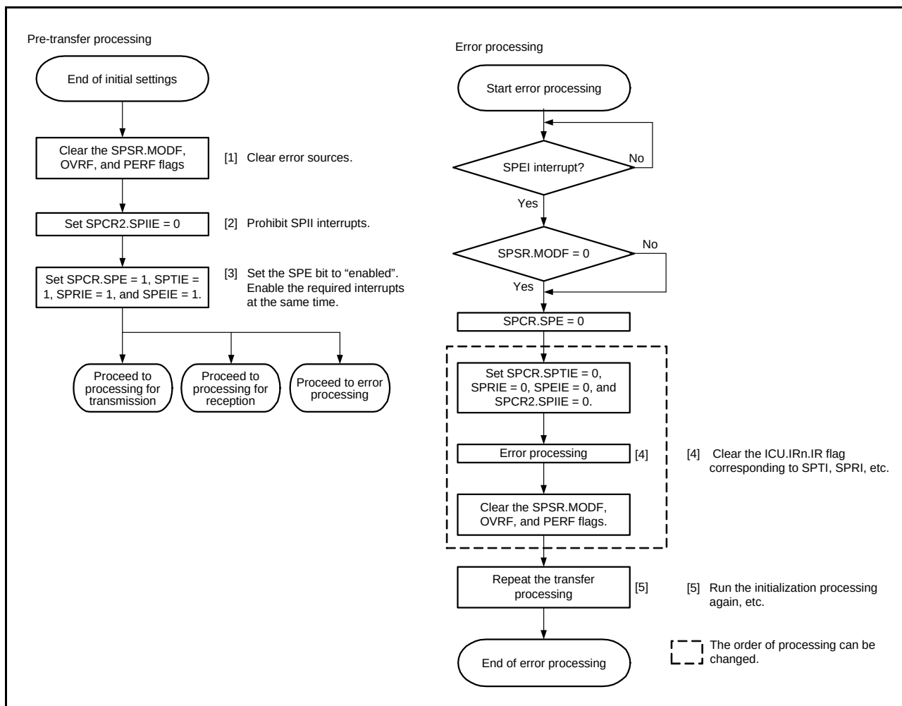
Figure 35.41 Flowchart for Slave Mode (Error Processing)
