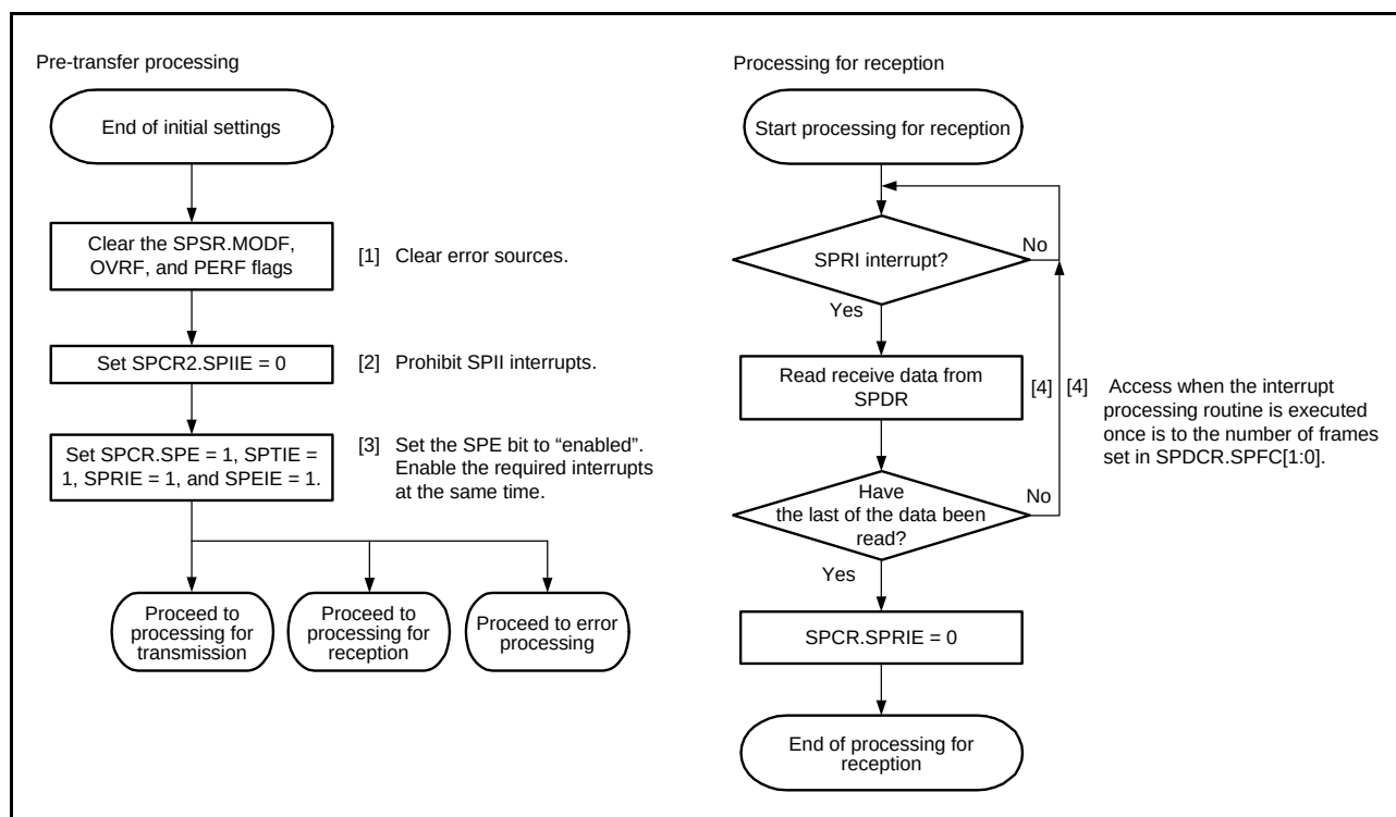
Figure 35.40 Flowchart for Slave Mode (Reception)
