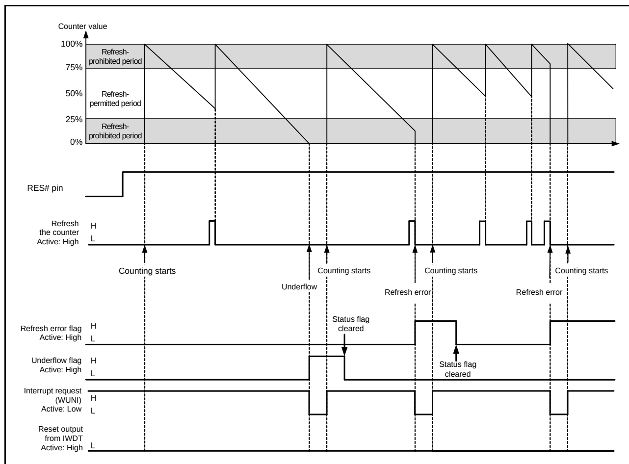
Figure 30.4 Operation Example in Auto-Start Mode
