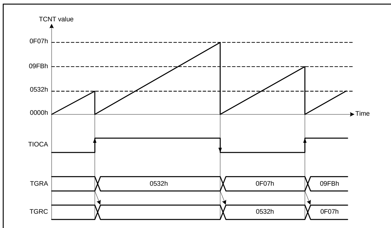
Figure 24.17 Example of Buffer Operation (2)
