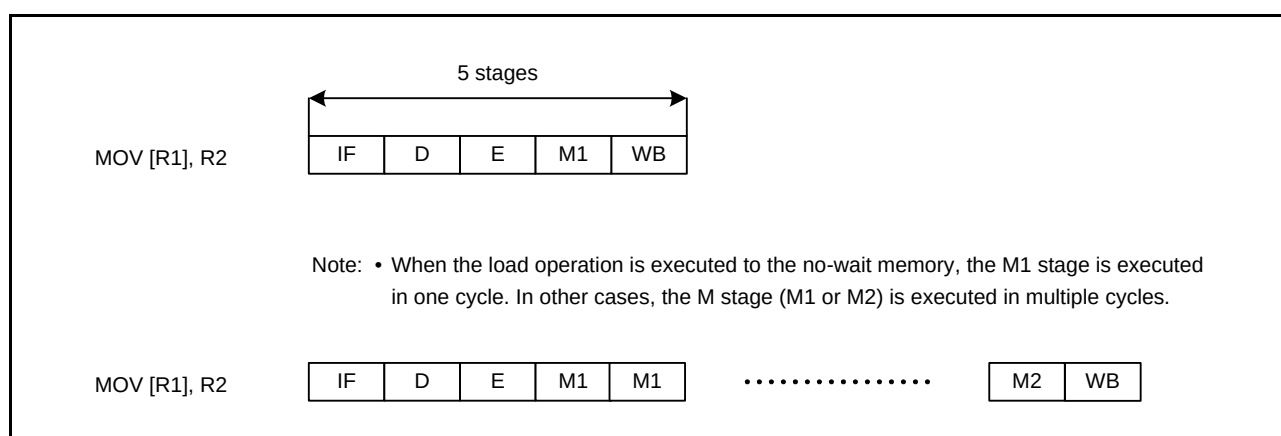
Figure 2.8 Load Operation
