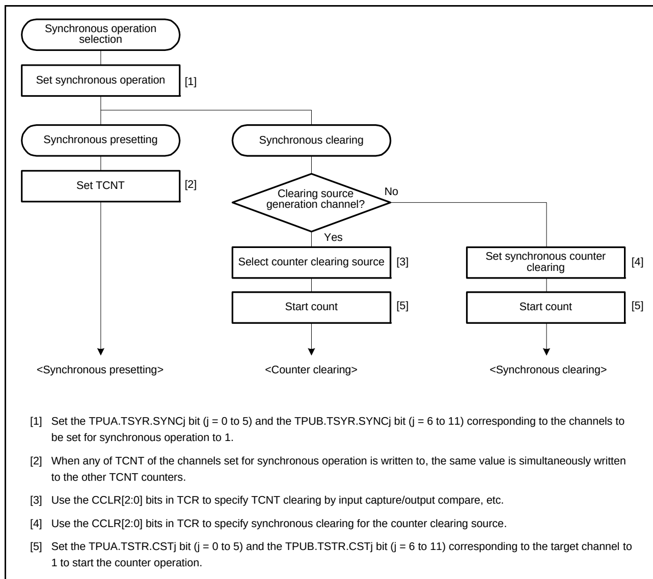
Figure 24.11 Example of Synchronous Operation Setting Procedure
