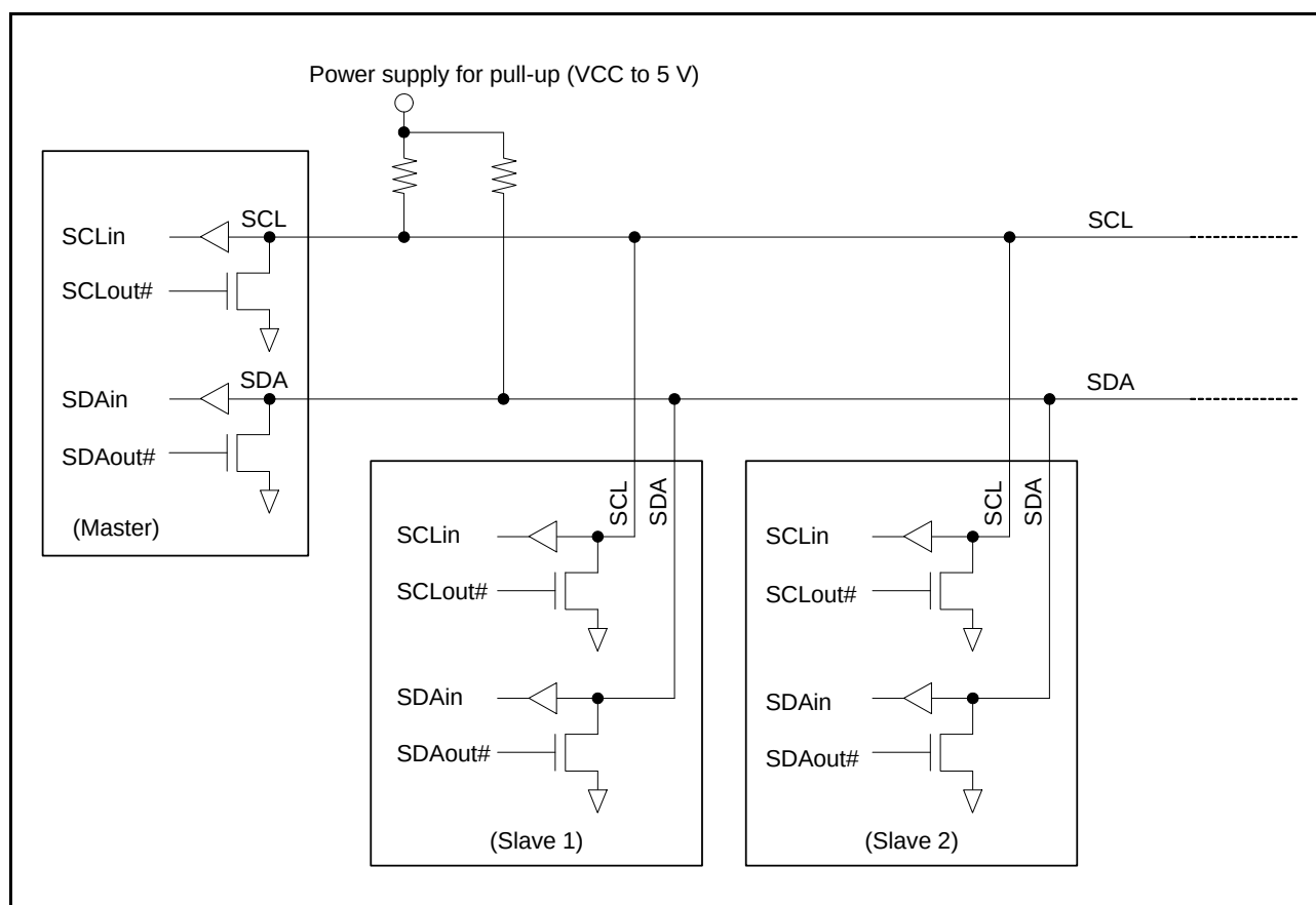
Figure 33.2 Connections to the External Circuit by the I/O Pins (I 2 C Bus Configuration Example)
