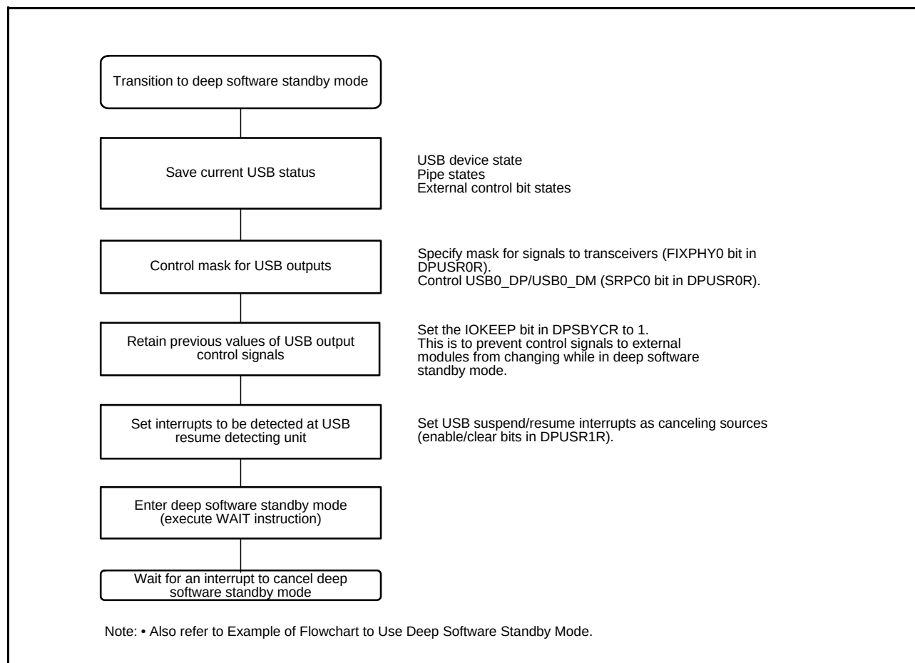
Figure 31.5 USB Setting Flowchart for Transition to Deep Software Standby Mode
