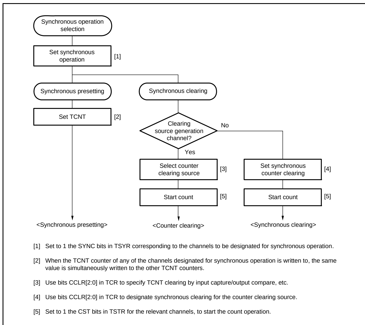
Figure 22.12 Example of Synchronous Operation Setting Procedure
