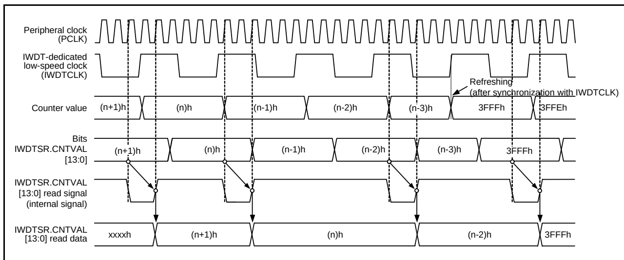
Figure 30.8 Processing for Reading IWDT Down-Counter Value (IWDTCR.CKS[3:0] = 0000b, IWDTCR.TOPS[1:0] = 11b)
