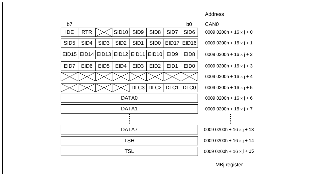
Figure 34.13 Structure of MBj (j = 0 to 31)
