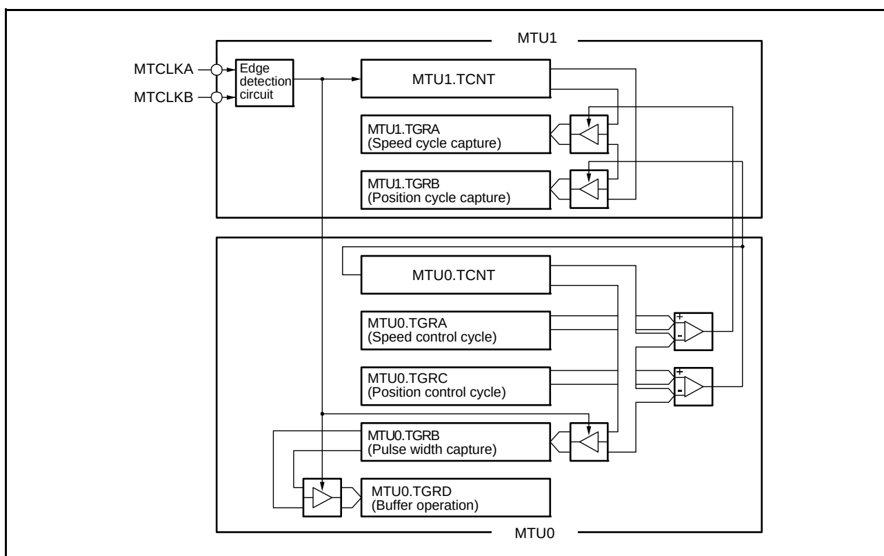
Figure 22.34 Phase Counting Mode Application Example
