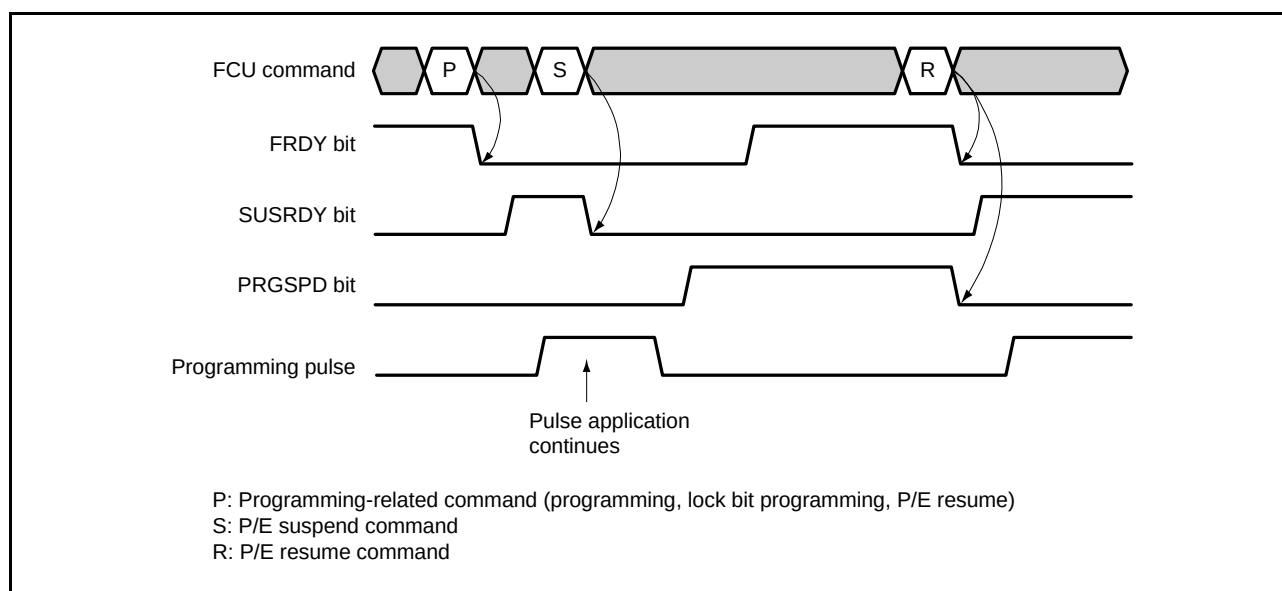
Figure 43.23 Suspension during Programming
