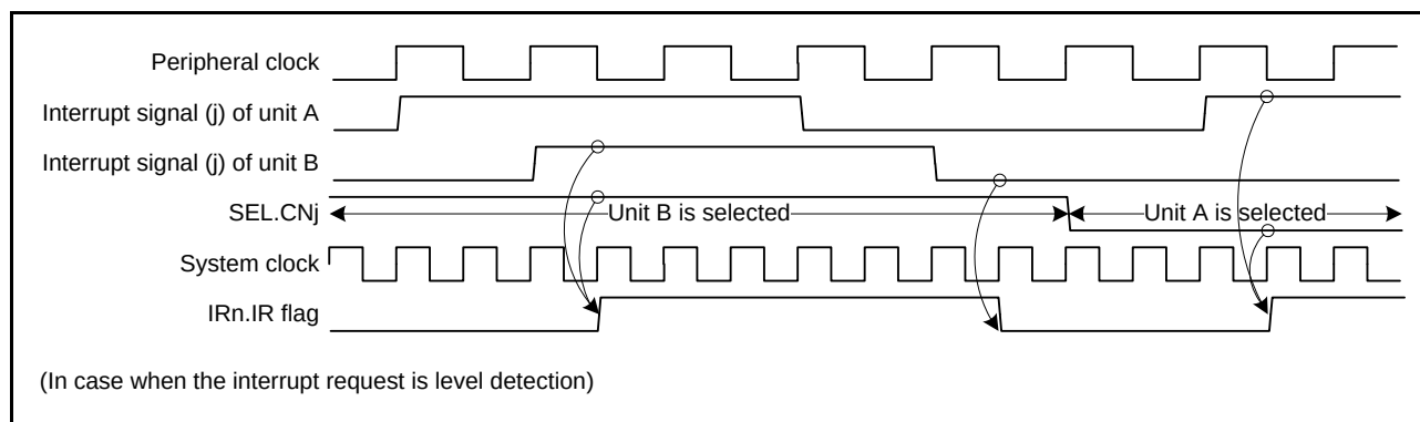
Figure 15.17 Unit Selection Example
