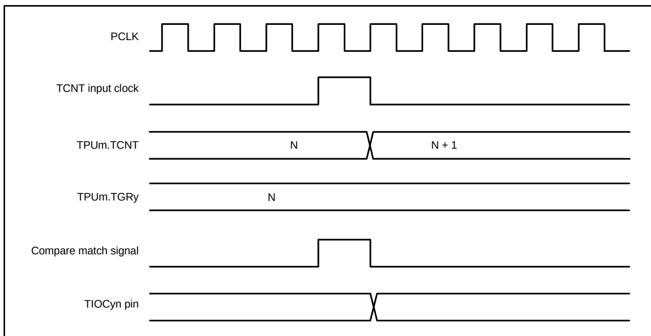
Figure 24.34 Output Compare Output Timing
