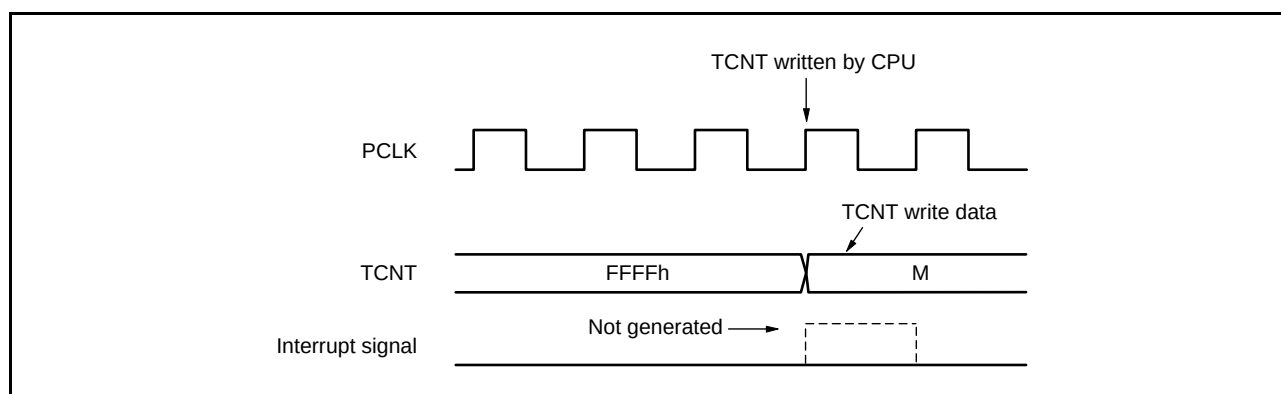
Figure 22.121 Contention between TCNT Write Operation and Overflow
