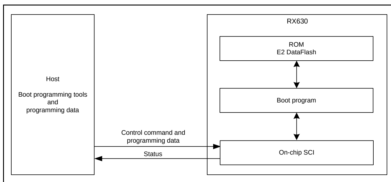
Figure 43.26 System Configuration for Operations in Boot Mode
