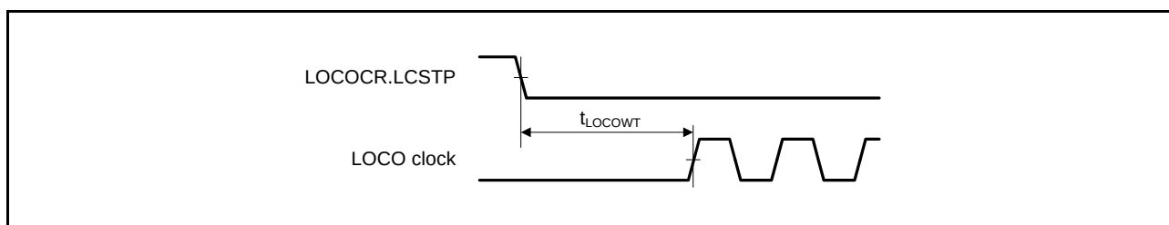
Figure 45.6 LOCO Clock Oscillation Start Timing
