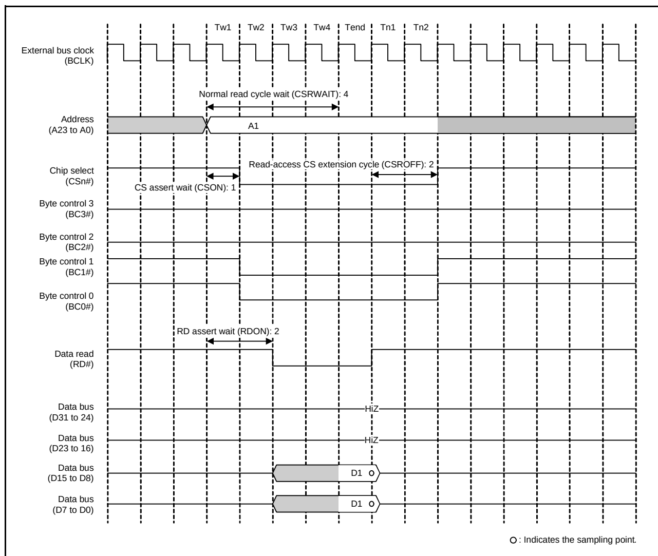
Figure 16.17 Example of Normal-Read Operation (when 32-Bit Bus Space is Accessed in 16 Bits) (n = 0 to 7)
