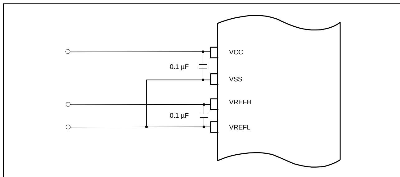
Figure 39.17 Connection Example of Power Supply Pins
