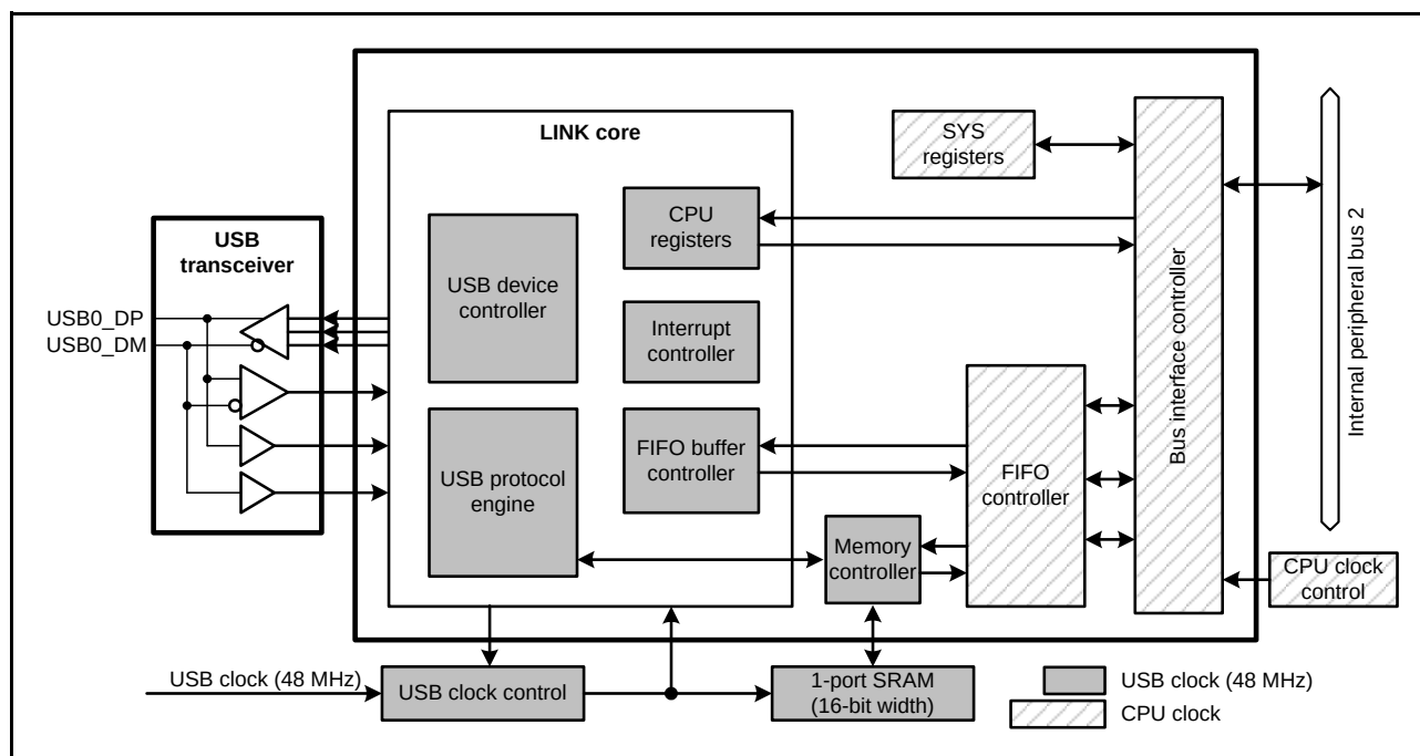
Figure 31.1 Block Diagram of USB
