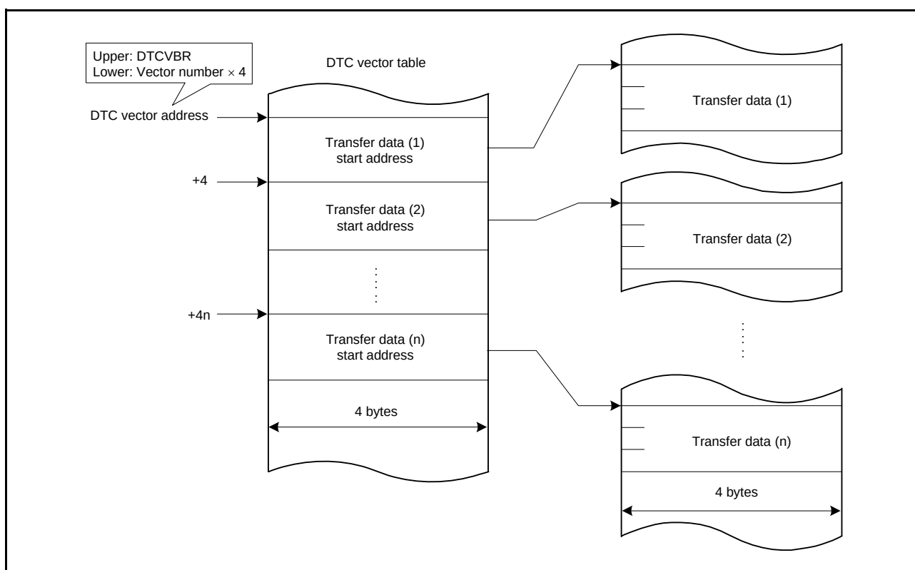
Figure 19.2 DTC Vector Table and Transfer Data
