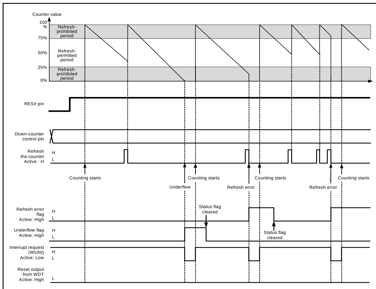
Figure 29.4 Operation Example in Auto-Start Mode
