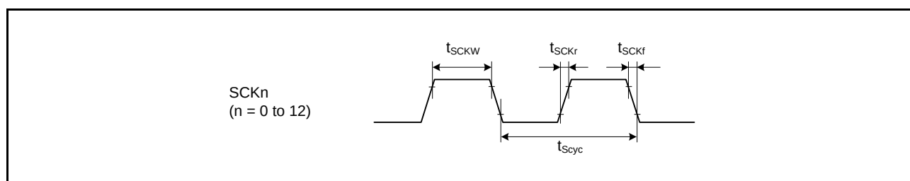
Figure 45.29 SCK Clock Input Timing
