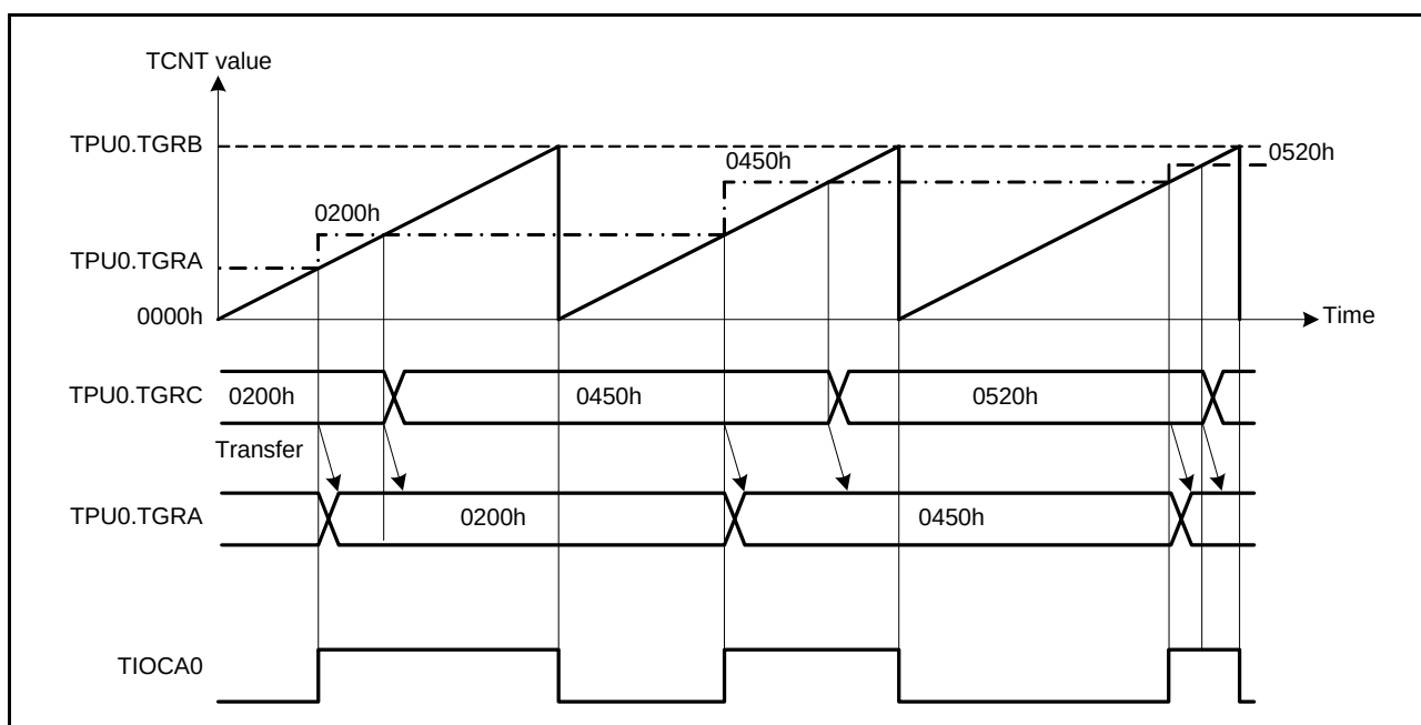
Figure 24.16 Example of Buffer Operation (1)
