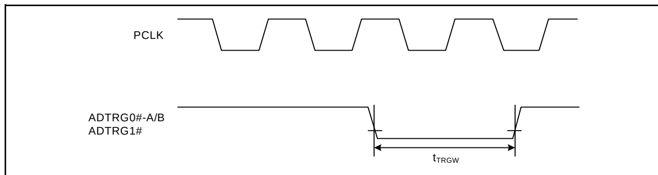
Figure 45.31 A/D Converter External Trigger Input Timing
