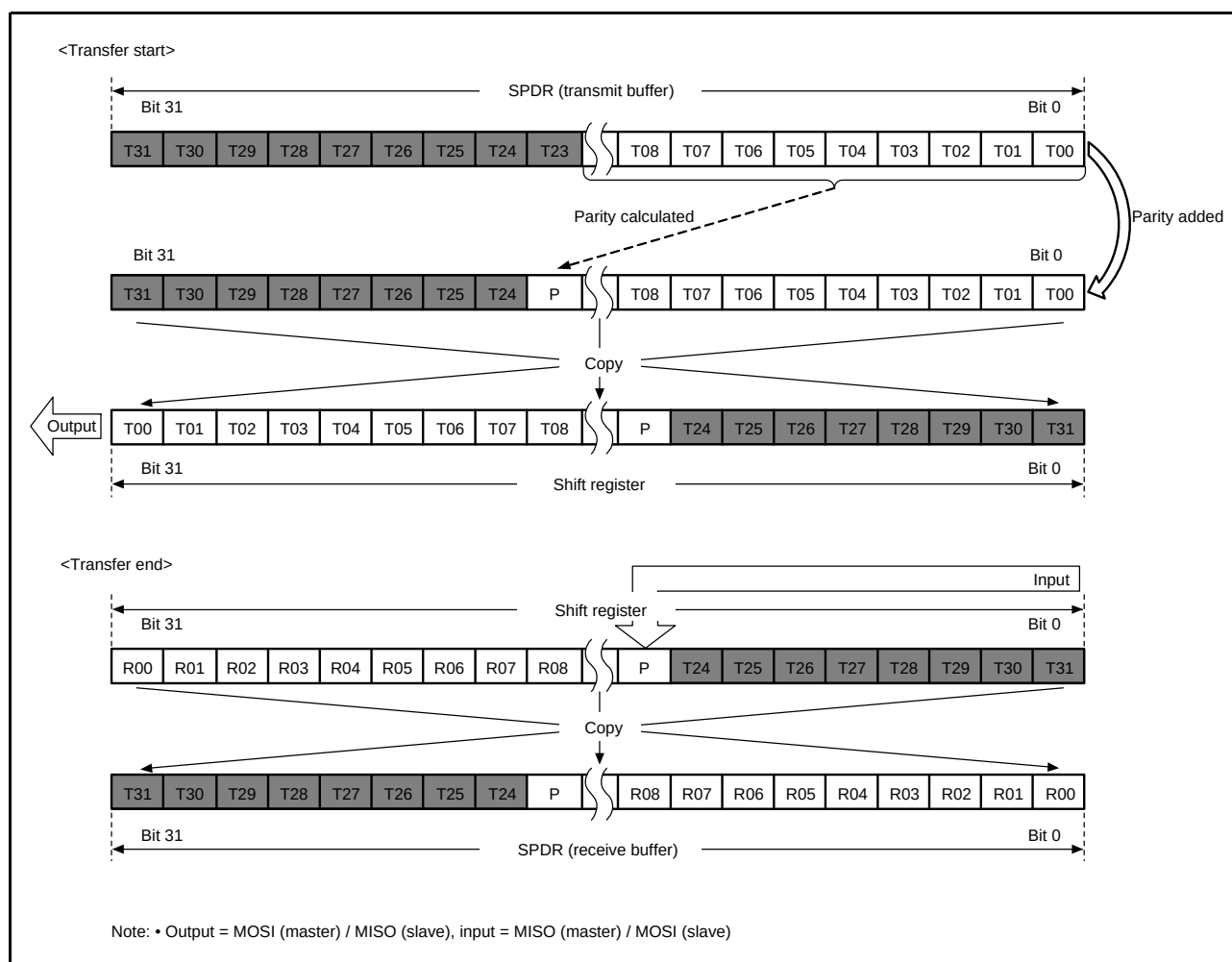
Figure 35.22 LSB-First Transfer (24-Bit Data, Parity Enabled)
