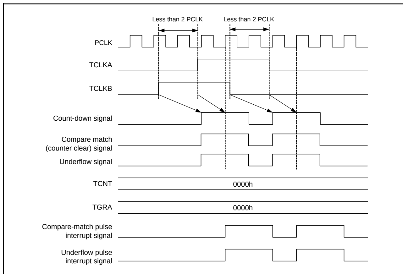
Figure 24.56 Continuous Output of Underflow Pulse Interrupt Signal
