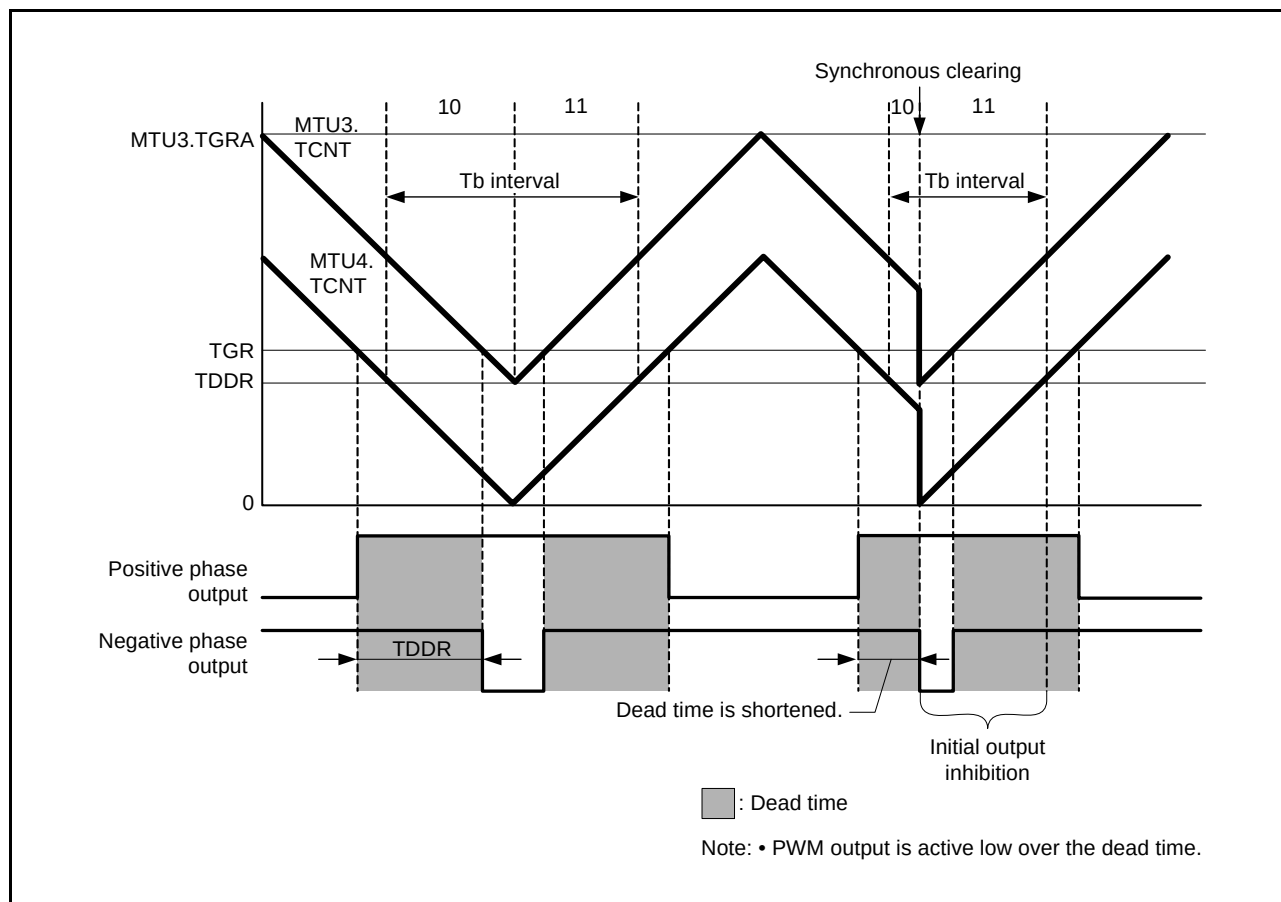
Figure 22.122 Example of Synchronous Clearing (when Condition 1 Applies)
