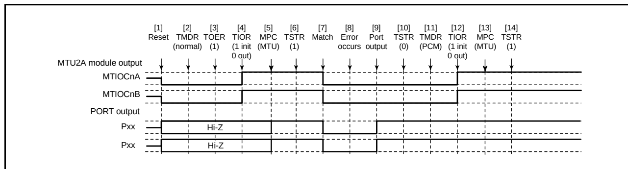
Figure 22.128 Error Occurrence in Normal Mode, Recovery in Phase Counting Mode
