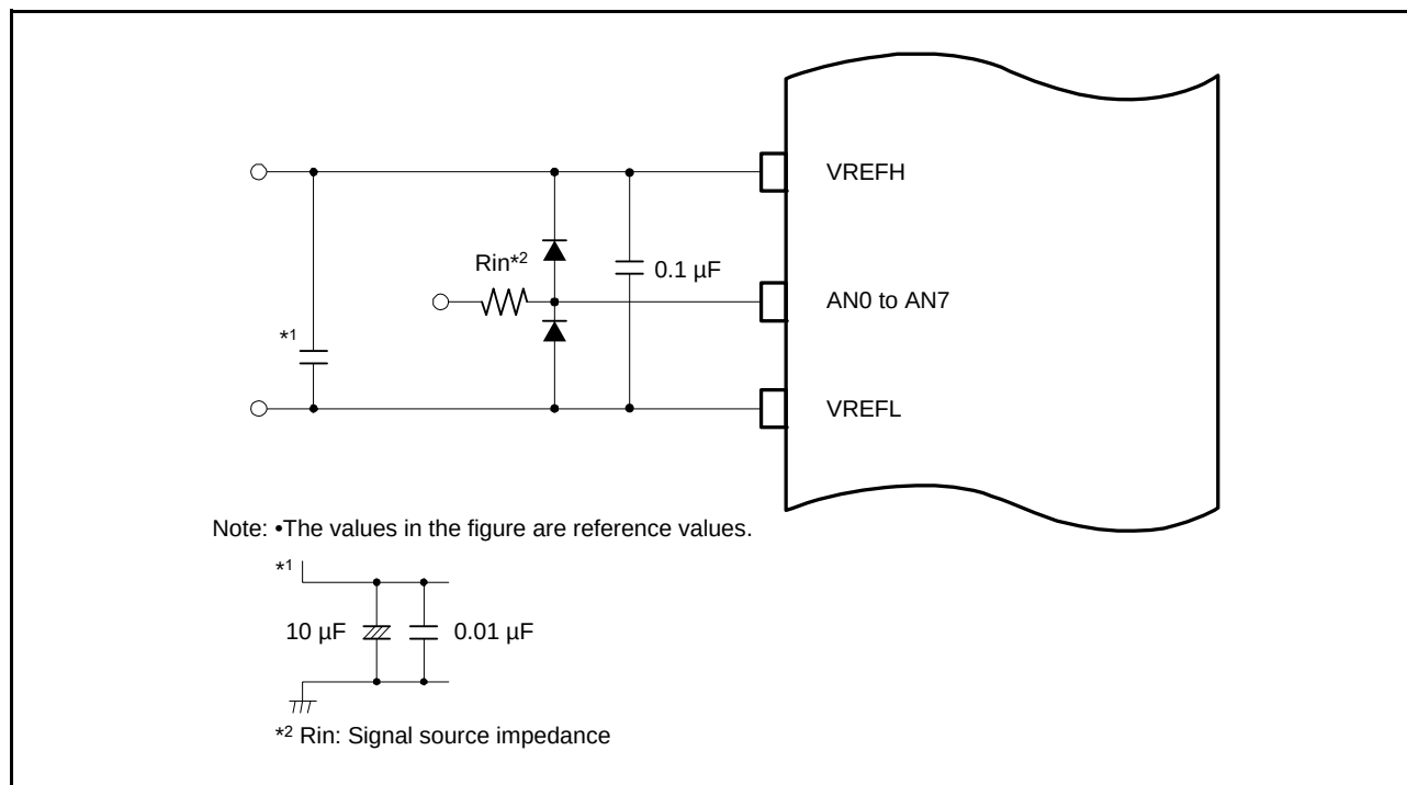
Figure 39.18 Example of Analog Input Pin Protection Circuit
