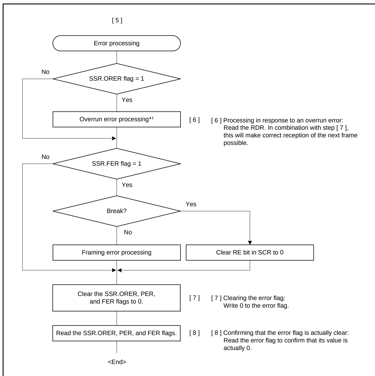
Figure 32.19 Example of Multi-Processor Serial Reception Flowchart (2)
