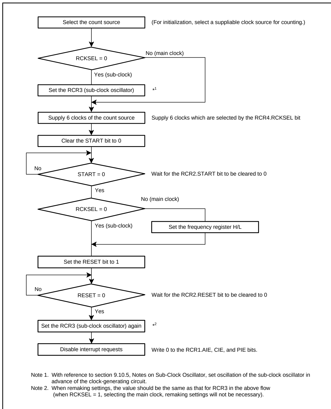
Figure 28.14 Initialization Procedure
