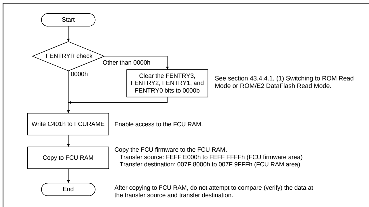
Figure 43.11 Procedure for Firmware Transfer to FCU RAM
