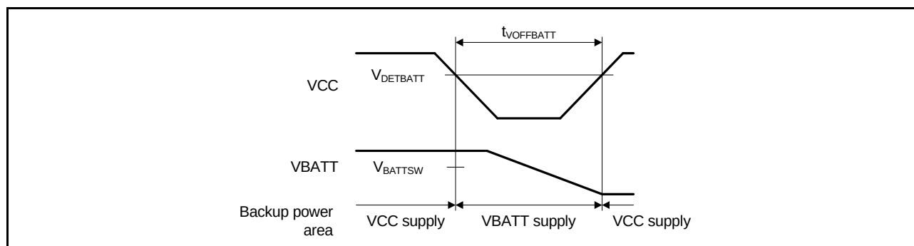
Figure 45.45 Battery Backup Function Characteristics
