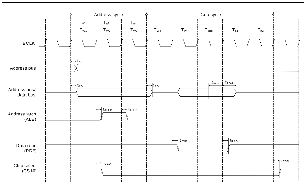
Figure 45.17 Address/Data Multiplexed Bus Read Access Timing
