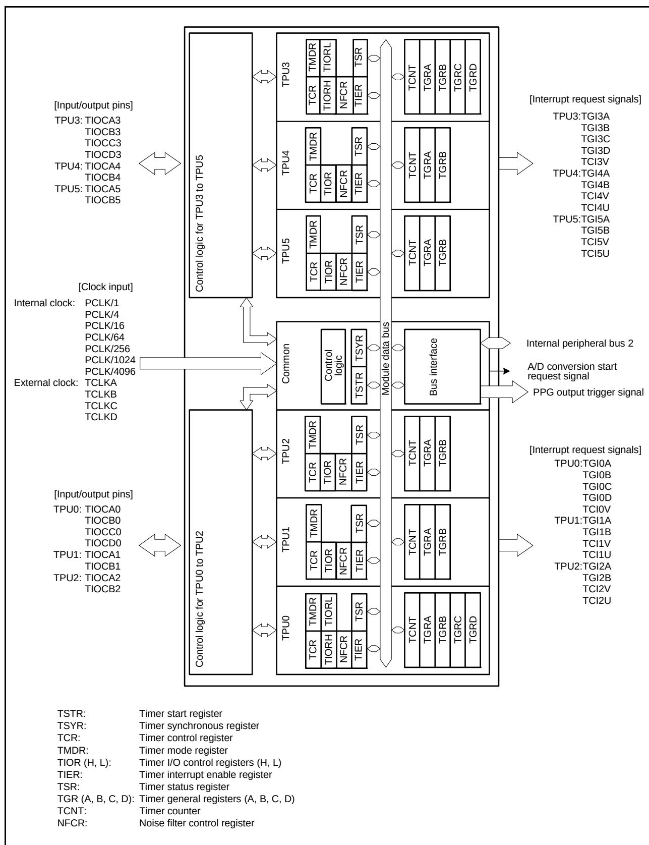
Figure 24.1 Block Diagram of TPU (Unit 0)
