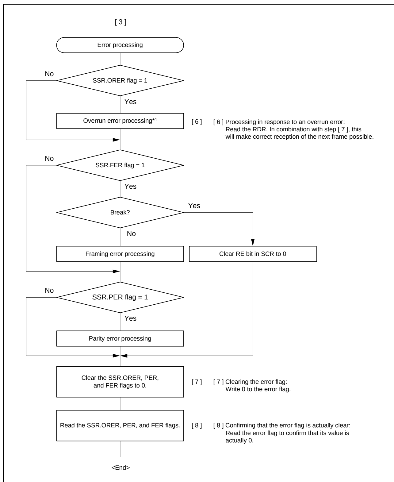
Figure 32.14 Example of Serial Reception Flowchart (2) (Asynchronous Mode)
