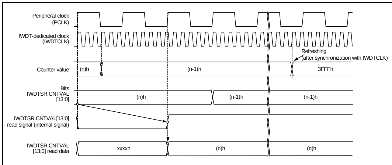
Figure 30.9 Processing for Reading IWDTCR Down-Counter Value (IWDTCR.CKS[3:0] = 0010b, IWDTCR.TOPS[1:0] = 11b)
