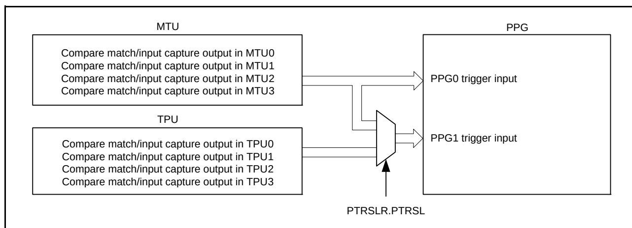
Figure 25.3 Block Diagram of PPG Trigger Selection
