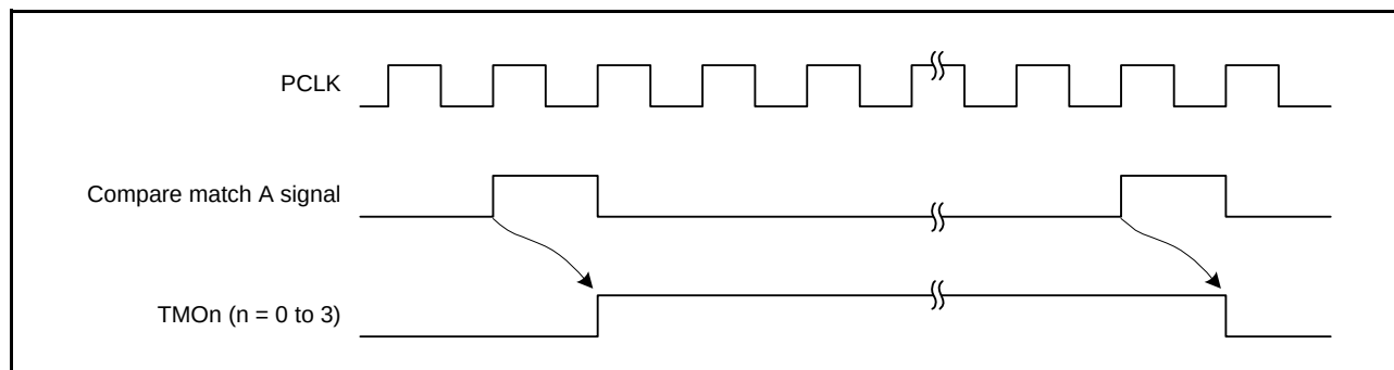
Figure 26.8 Timing of Timer Output at Compare Match A Signal
