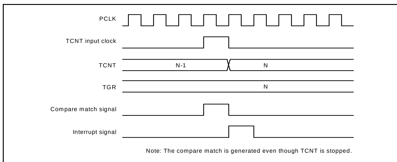
Figure 22.101 TGI Interrupt Timing (Compare Match) (MTU5)
