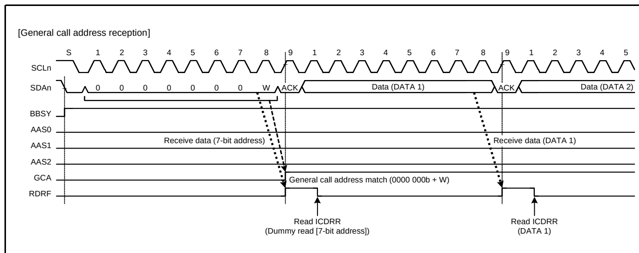
Figure 33.26 Timing of GCA Flag Setting during Reception of General Call Address
