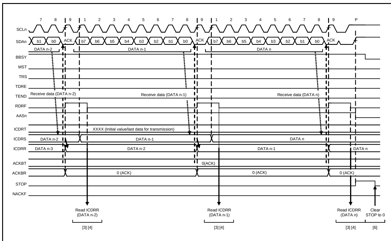
Figure 33.19 Slave Receive Operation Timing (2) (when RDRFS = 0)
