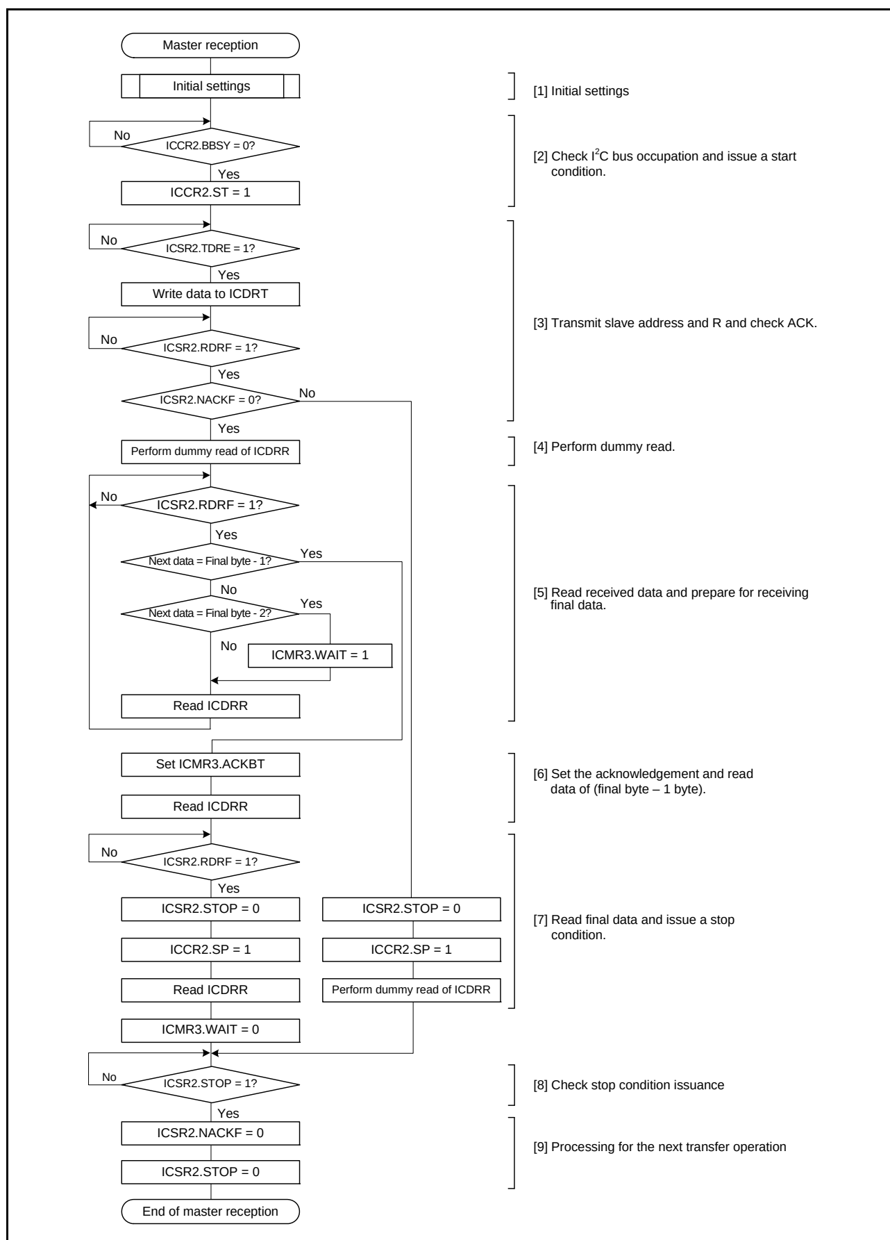
Figure 33.10 Example of Master Reception Flowchart (7-Bit Address Format)
