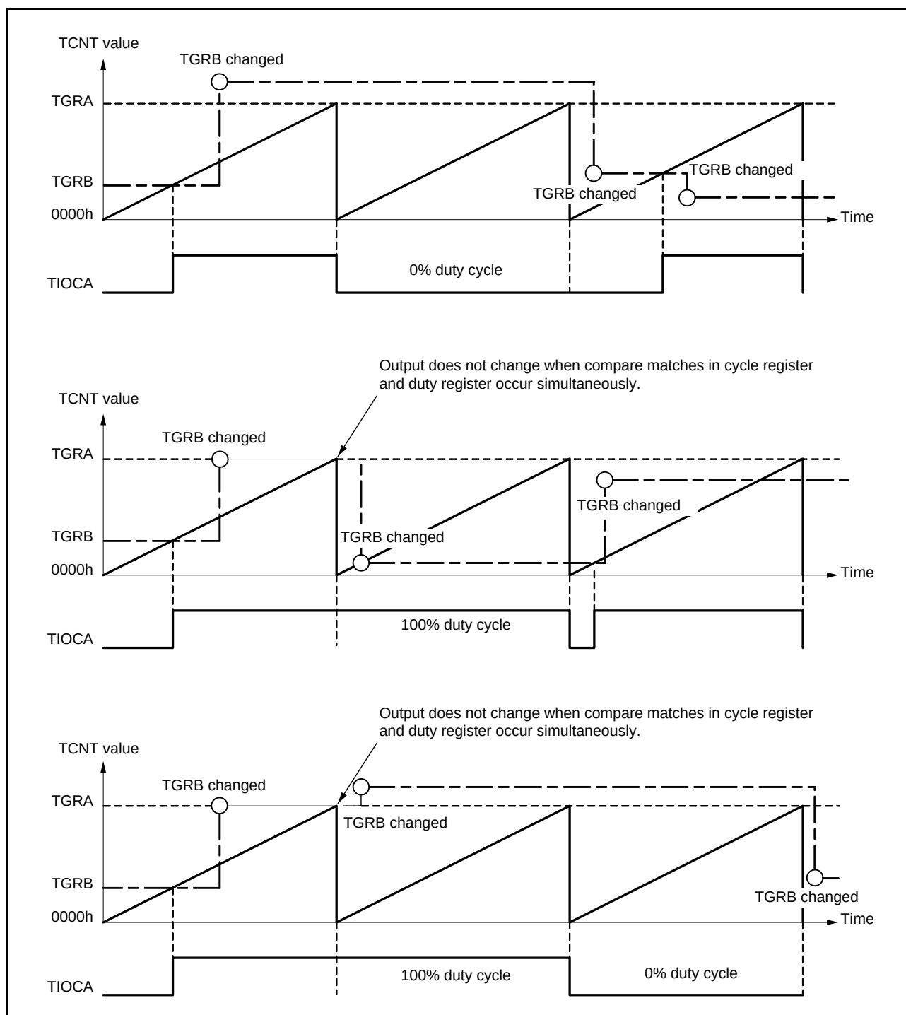
Figure 24.24 Example of PWM Mode Operation (3)
