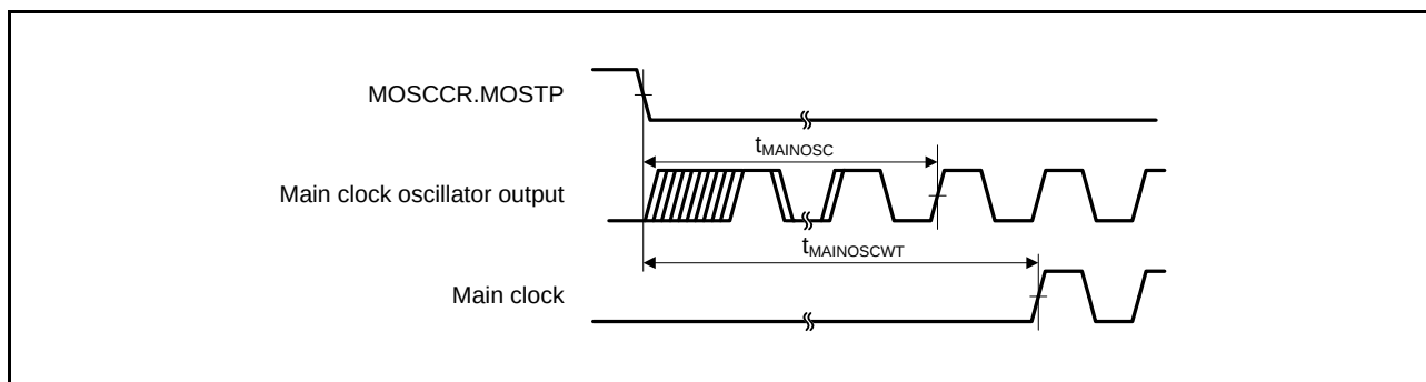
Figure 45.5 Main Clock Oscillation Start Timing
