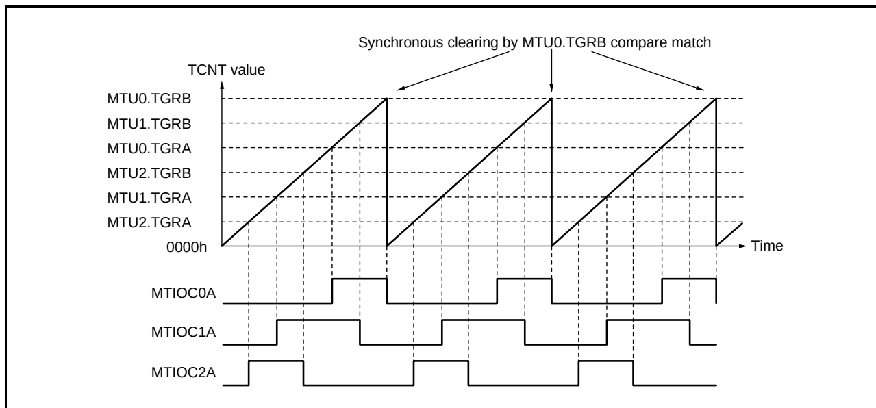
Figure 22.13 Example of Synchronous Operation
