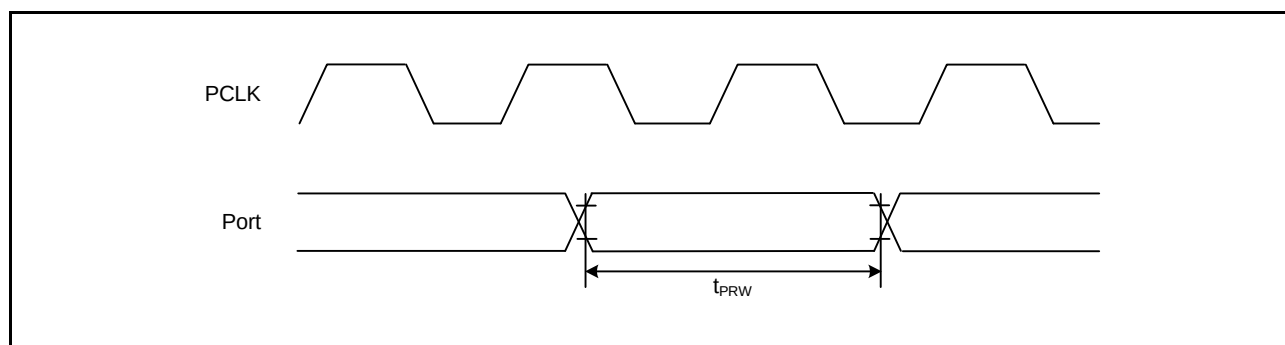
Figure 45.24 I/O Port Input Timing
