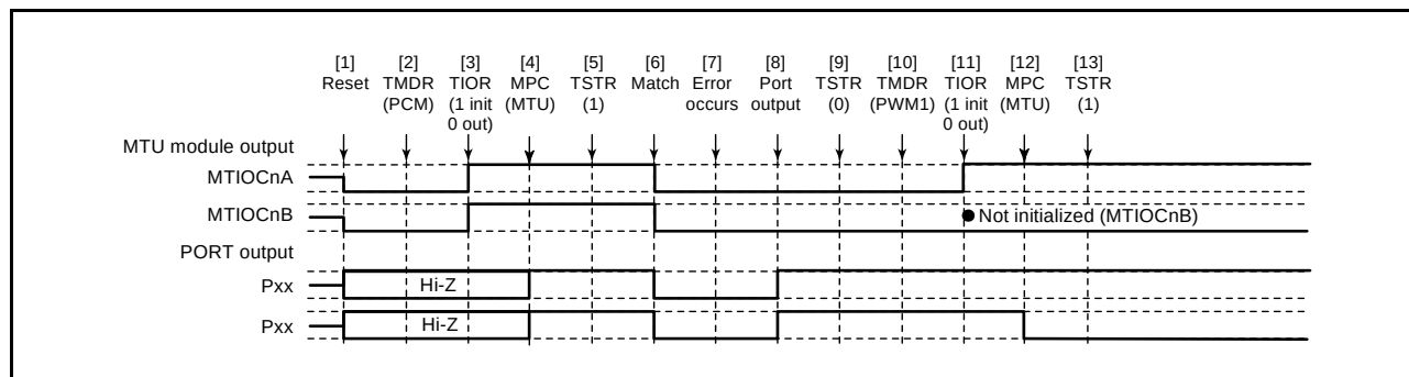
Figure 22.142 Error Occurrence in Phase Counting Mode, Recovery in PWM Mode 1
