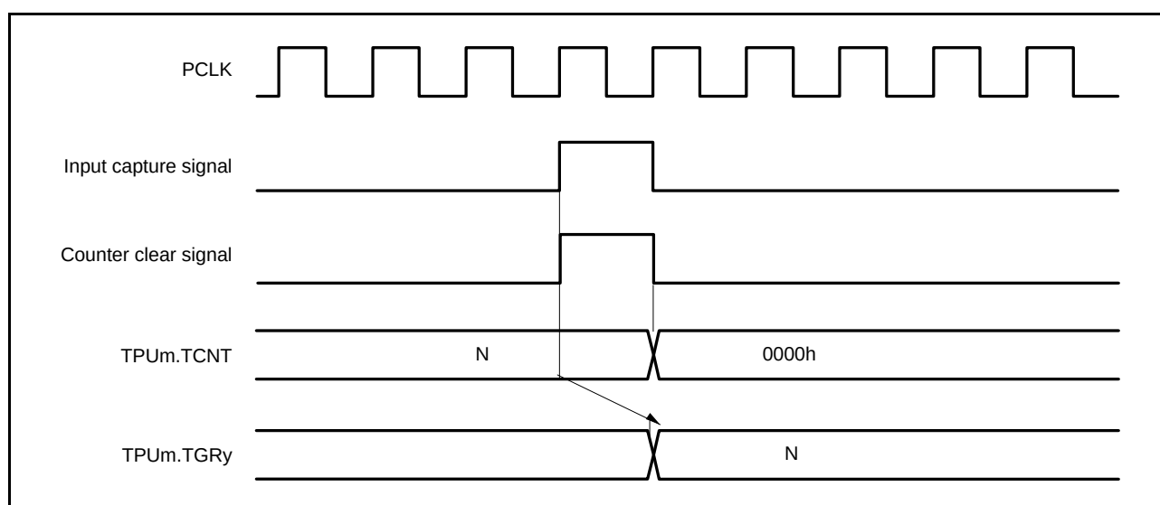
Figure 24.37 Counter Clear Timing (Input Capture)
