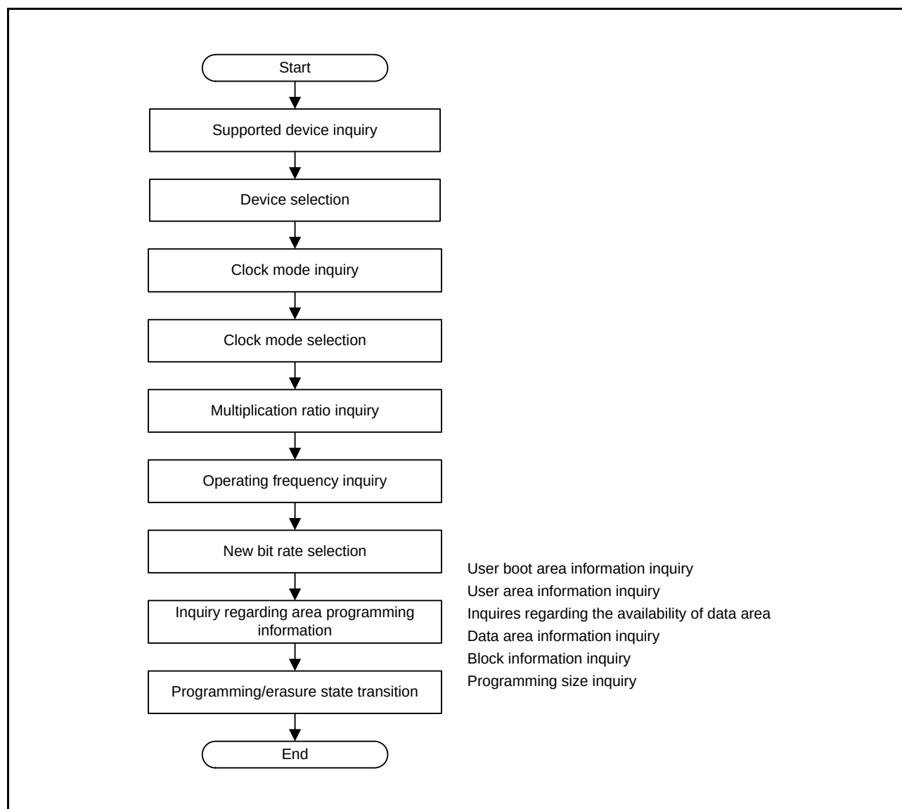
Figure 43.31 Example of Procedure to Use Inquiry/Selection Commands
