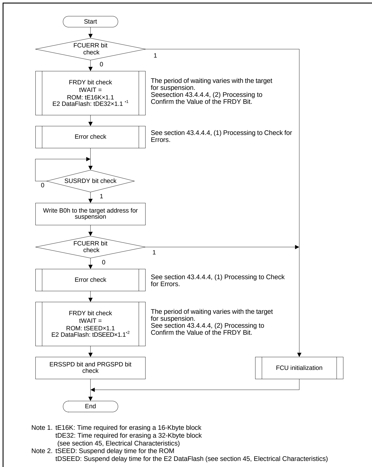
Figure 43.18 Procedure for Programming/Erasure Suspension
