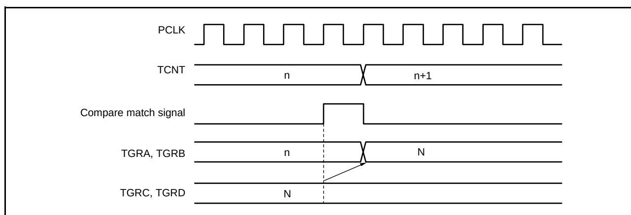
Figure 22.94 Buffer Operation Timing (Compare Match)
