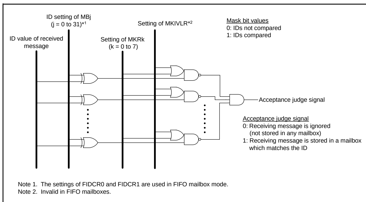
Figure 34.17 Acceptance Filtering
