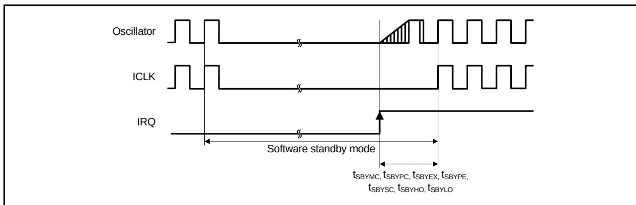
Figure 45.13 Software Standby Mode Cancellation Timing
