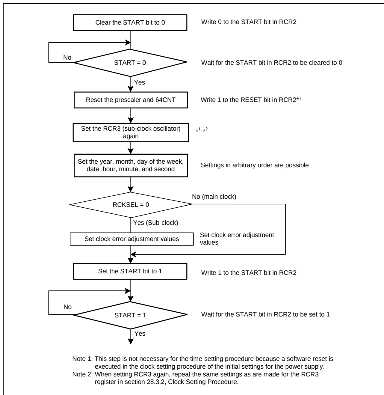
Figure 28.4 Setting the Time
