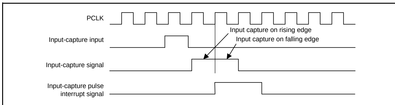
Figure 24.55 Continuous Output of Input-Capture Pulse Interrupt Signal
