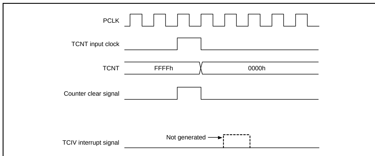
Figure 22.120 Contention between Overflow and Counter Clearing
