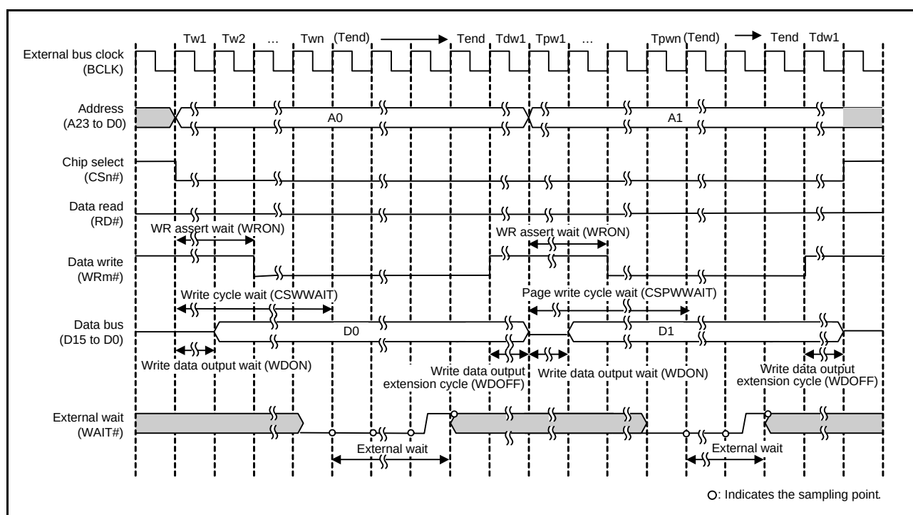
Figure 16.34 Example of External Wait Timing (Page-Write Access to 16-Bit Bus Space, in Byte Strobe Mode) ( n = 0 to 7, m = 0, 1 )
