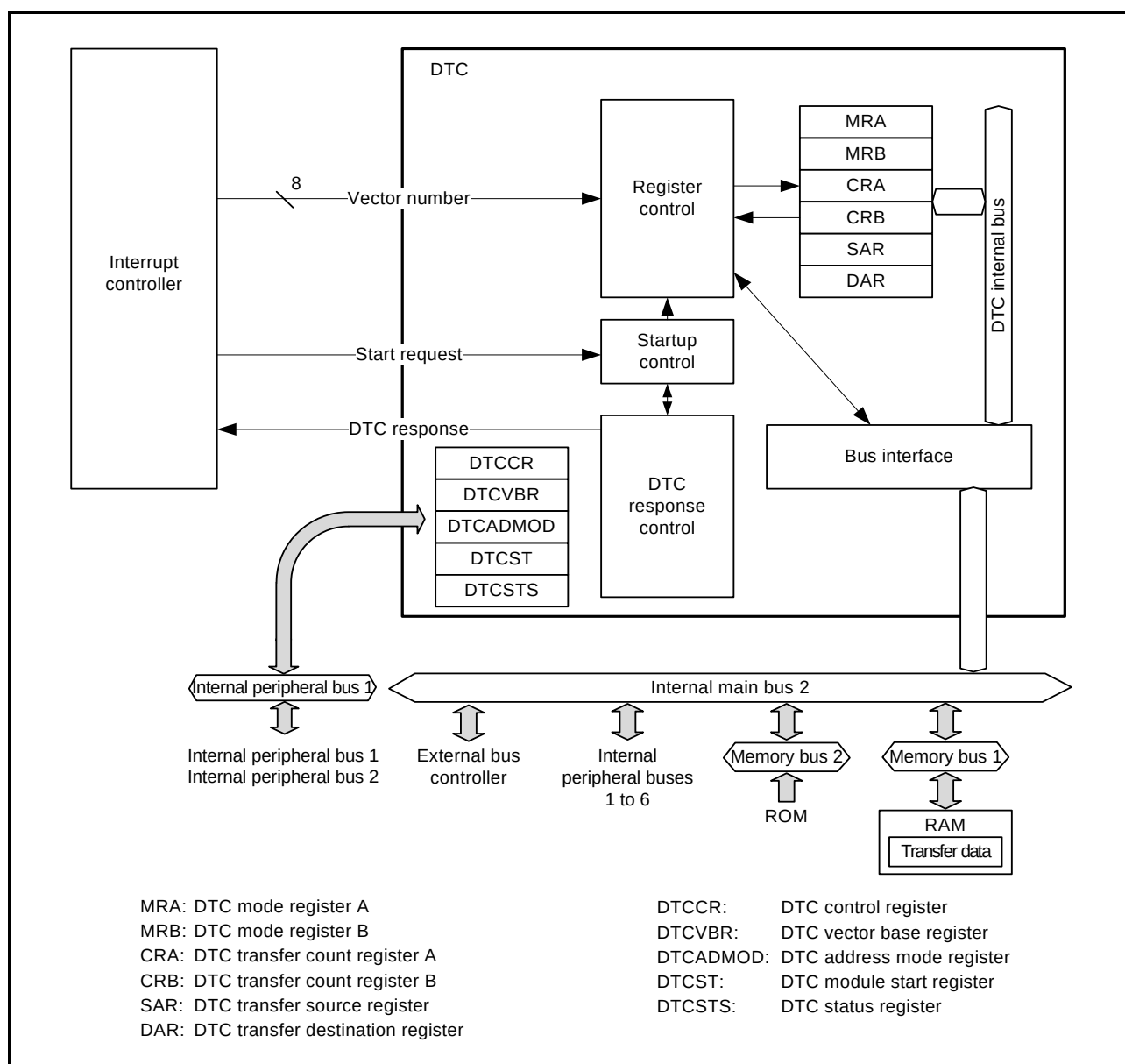
Figure 19.1 Block Diagram of DTC
