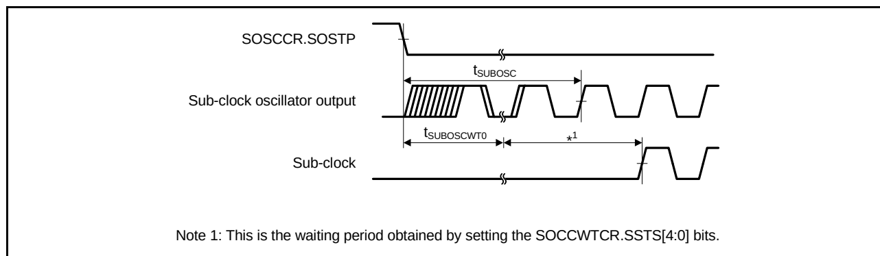
Figure 45.12 Sub-Clock Oscillation Start Timing
