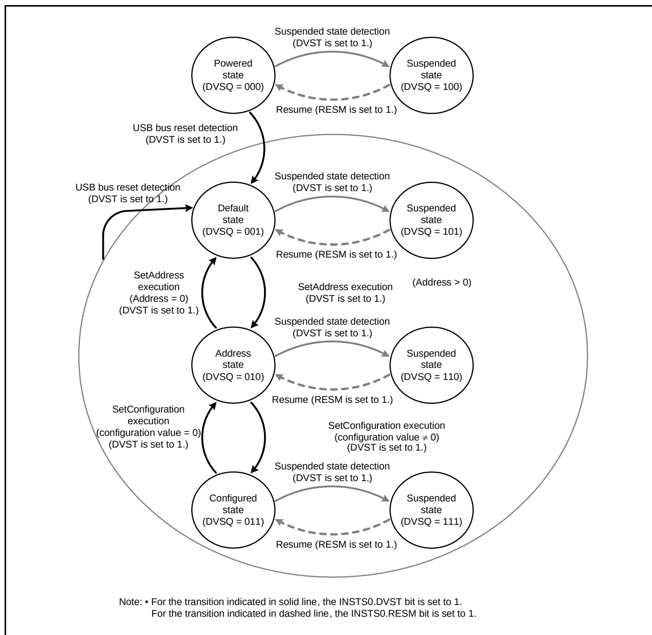
Figure 31.11 Device State Transitions
