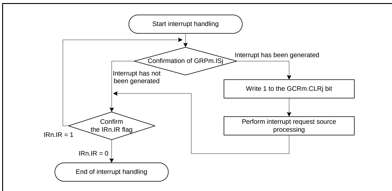
Figure 15.13 Procedure for Interrupt Handling of Edge Detection Groups 1 to 6
