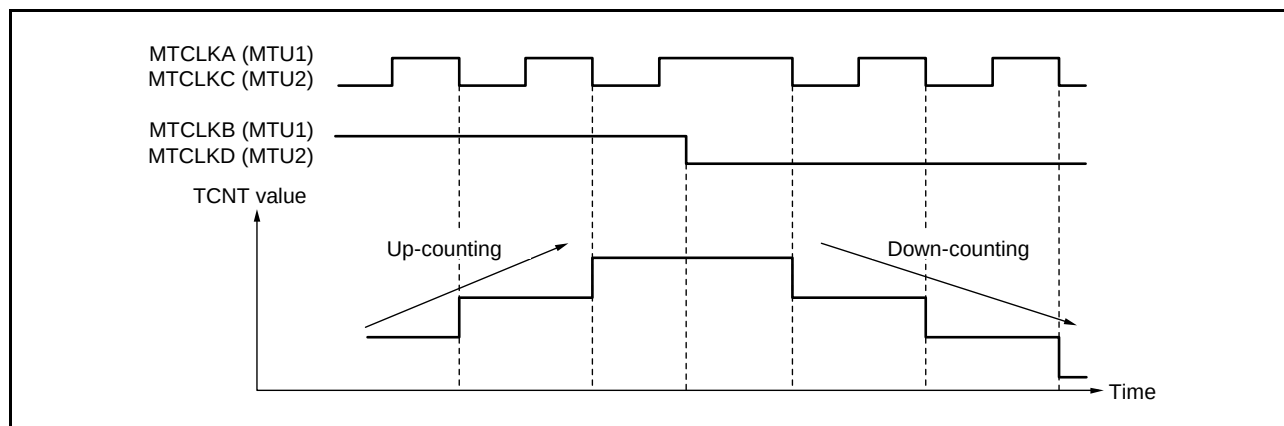
Figure 22.31 Example of Operation in Phase Counting Mode 2
