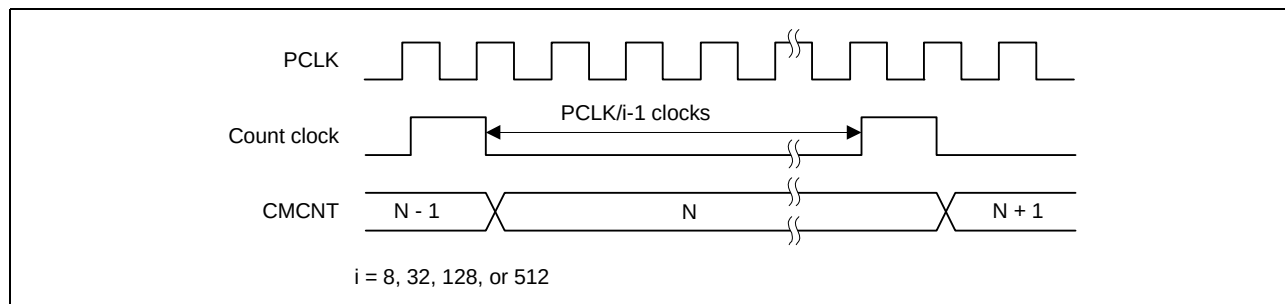
Figure 27.3 CMCNT Count Timing
