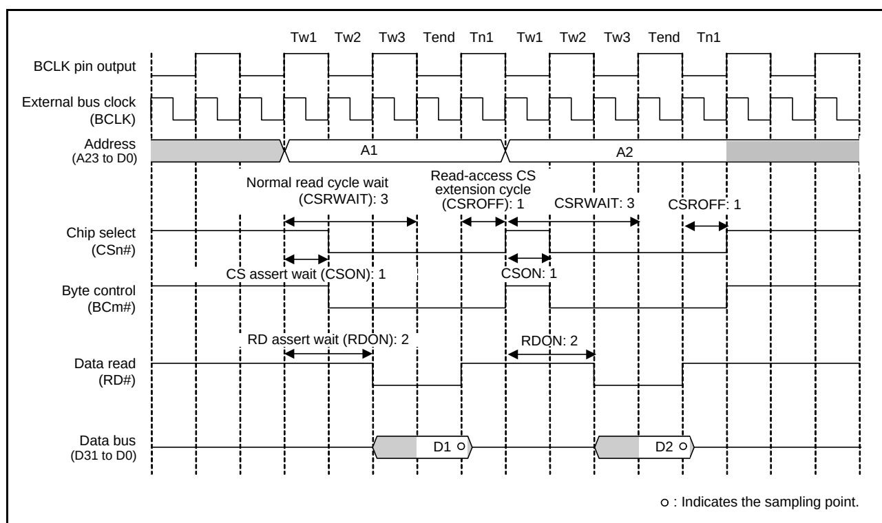
Figure 16.22 Example of Normal-Read Operation (when 1/2 BCLK is Selected with the BCLK Pin Output Select Bit and Two Rounds of Bus Access are Generated in Response to a Single Request for Transfer) (n = 0 to 7, m = 0 to 3)
