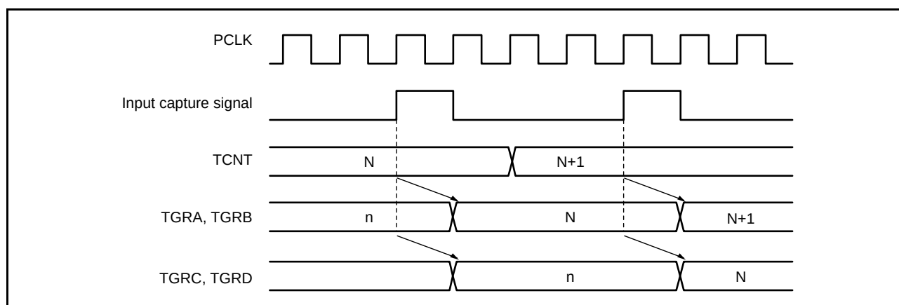
Figure 22.95 Buffer Operation Timing (Input Capture)
