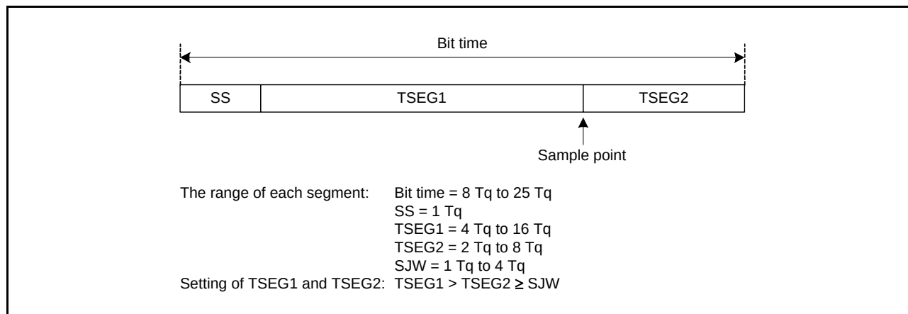
Figure 34.12 Bit Timing
