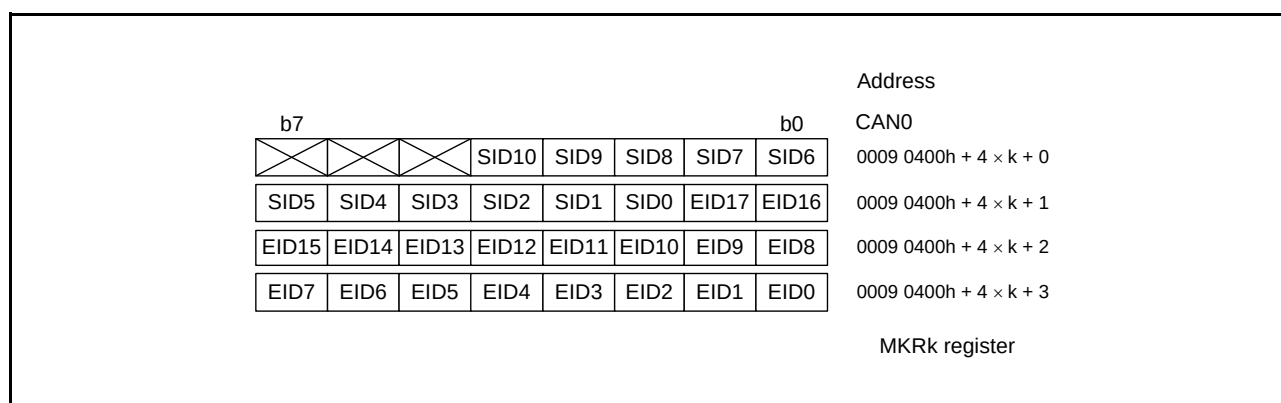
Figure 34.14 Structure of MKRk (k = 0 to 7)
