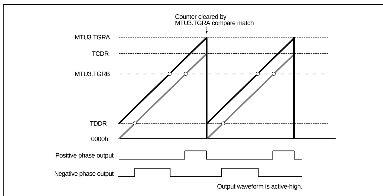
Figure 22.62 Example of Counter Clearing Operation by MTU3.TGRA Compare Match
