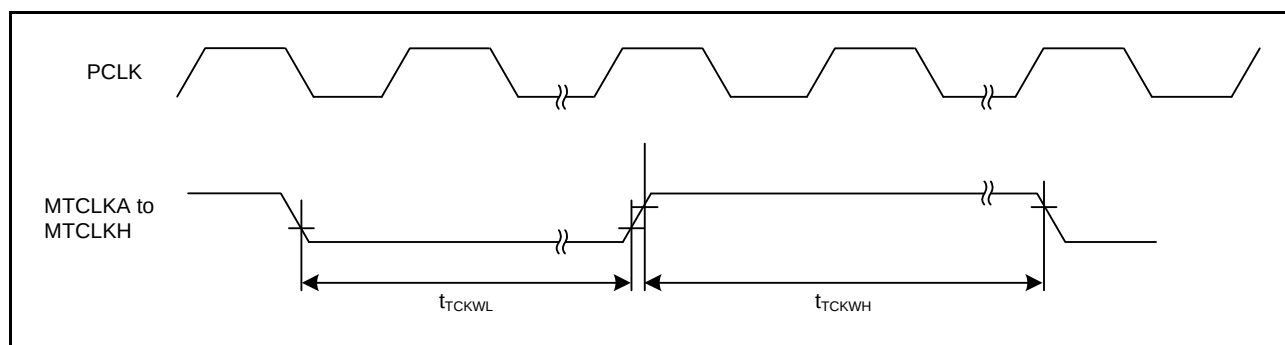
Figure 45.26 MTU Clock Input Timing
