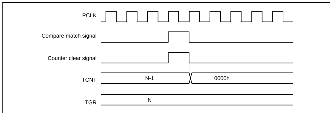
Figure 22.92 Counter Clear Timing (Compare Match) (MTU5)
