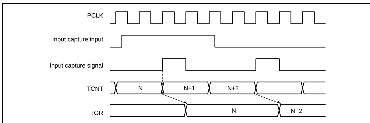
Figure 22.90 Input Capture Input Signal Timing
