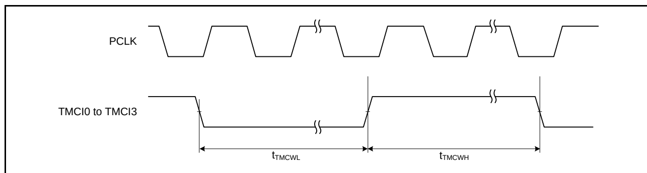
Figure 45.28 8-Bit Timer Clock Input Timing
