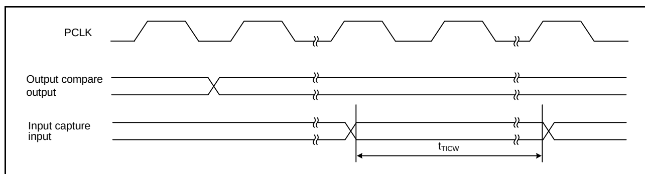
Figure 45.25 MTU Input/Output Timing
