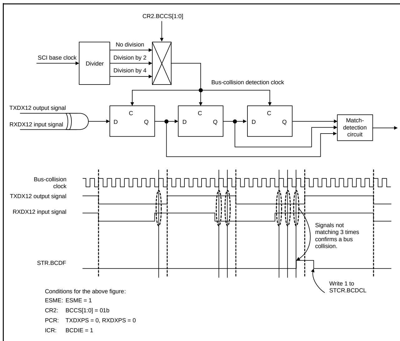
Figure 32.62 Example of Operations with Bus-Collision Detection
