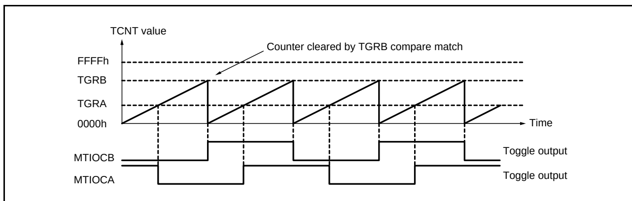
Figure 22.9 Example of Toggle Output Operation
