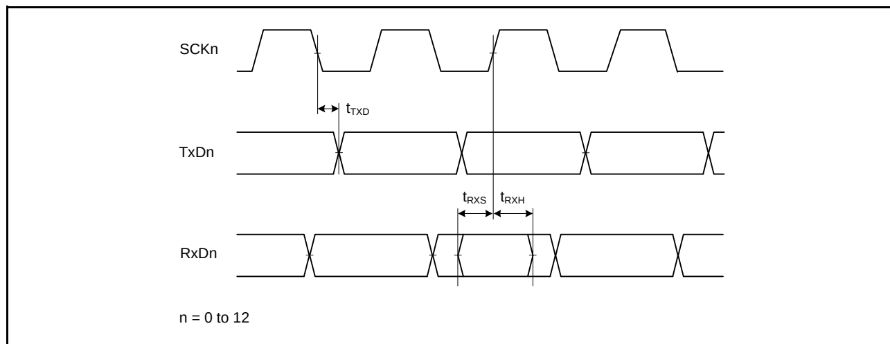
Figure 45.30 SCI Input/Output Timing: Clock Synchronous Mode
