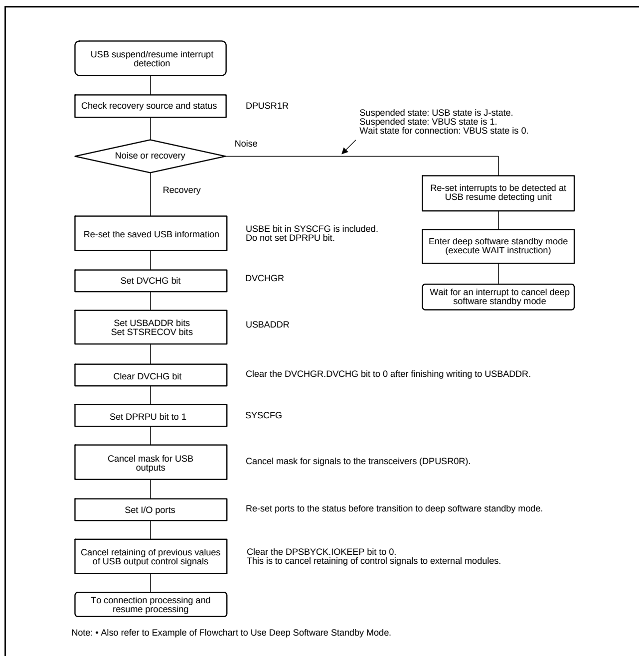
Figure 31.6 USB Setting Flowchart for Canceling Deep Software Standby Mode
