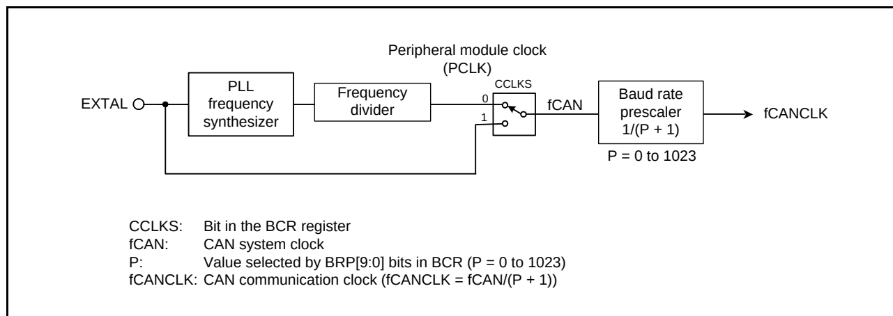
Figure 34.11 Block Diagram of CAN Clock Generator
