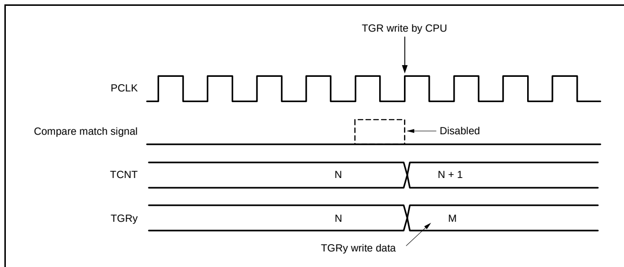
Figure 24.47 Conflict between TPUm.TGRy Write and Compare Match
