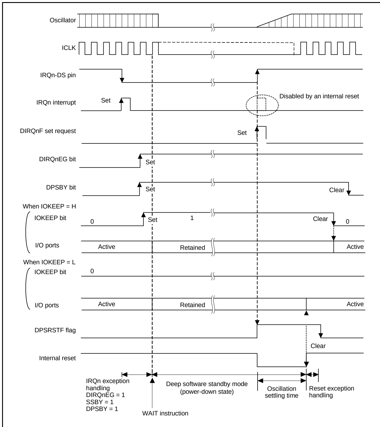
Figure 11.3 Example of Deep Software Standby Mode Application
