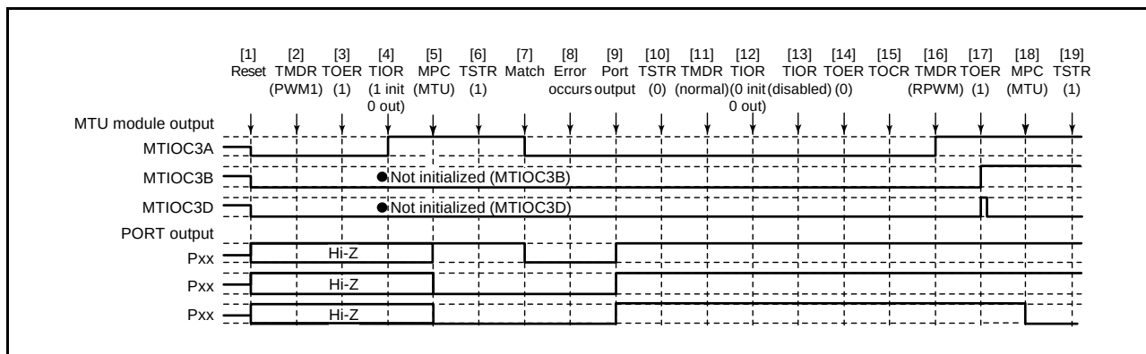
Figure 22.136 Error Occurrence in PWM Mode 1, Recovery in Reset-Synchronized PWM Mode
