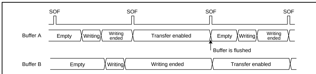
Figure 31.16 Example of Buffer Flush Operation
