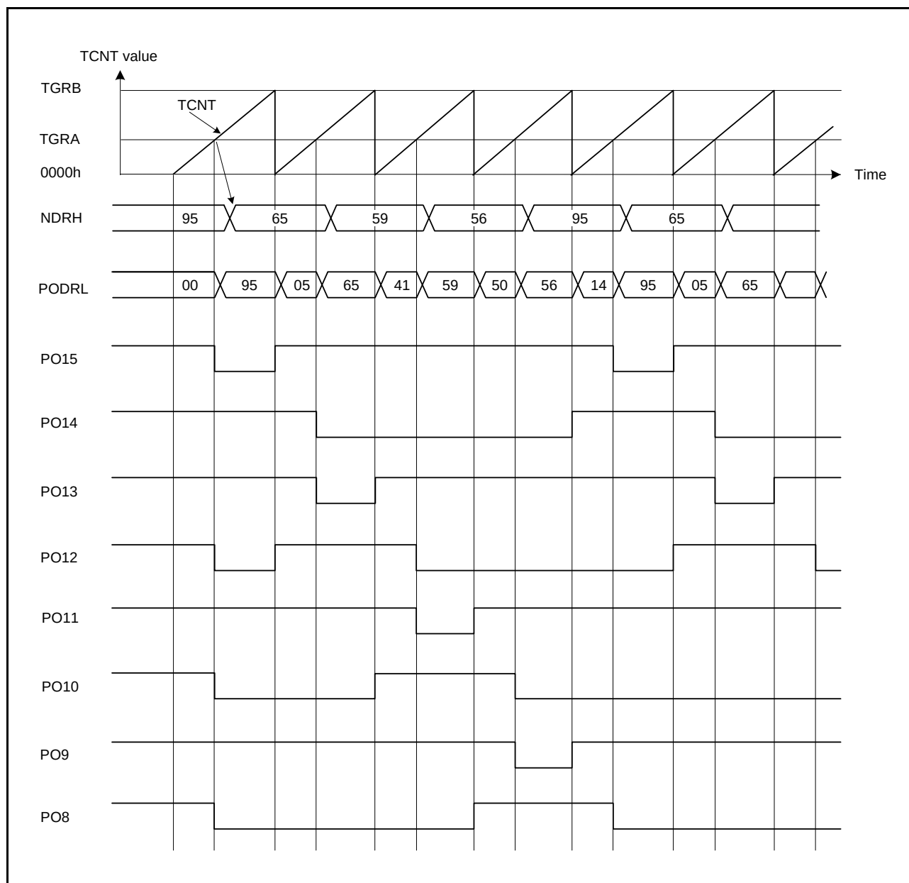
Figure 25.14 Inverted Pulse Output (Example)
