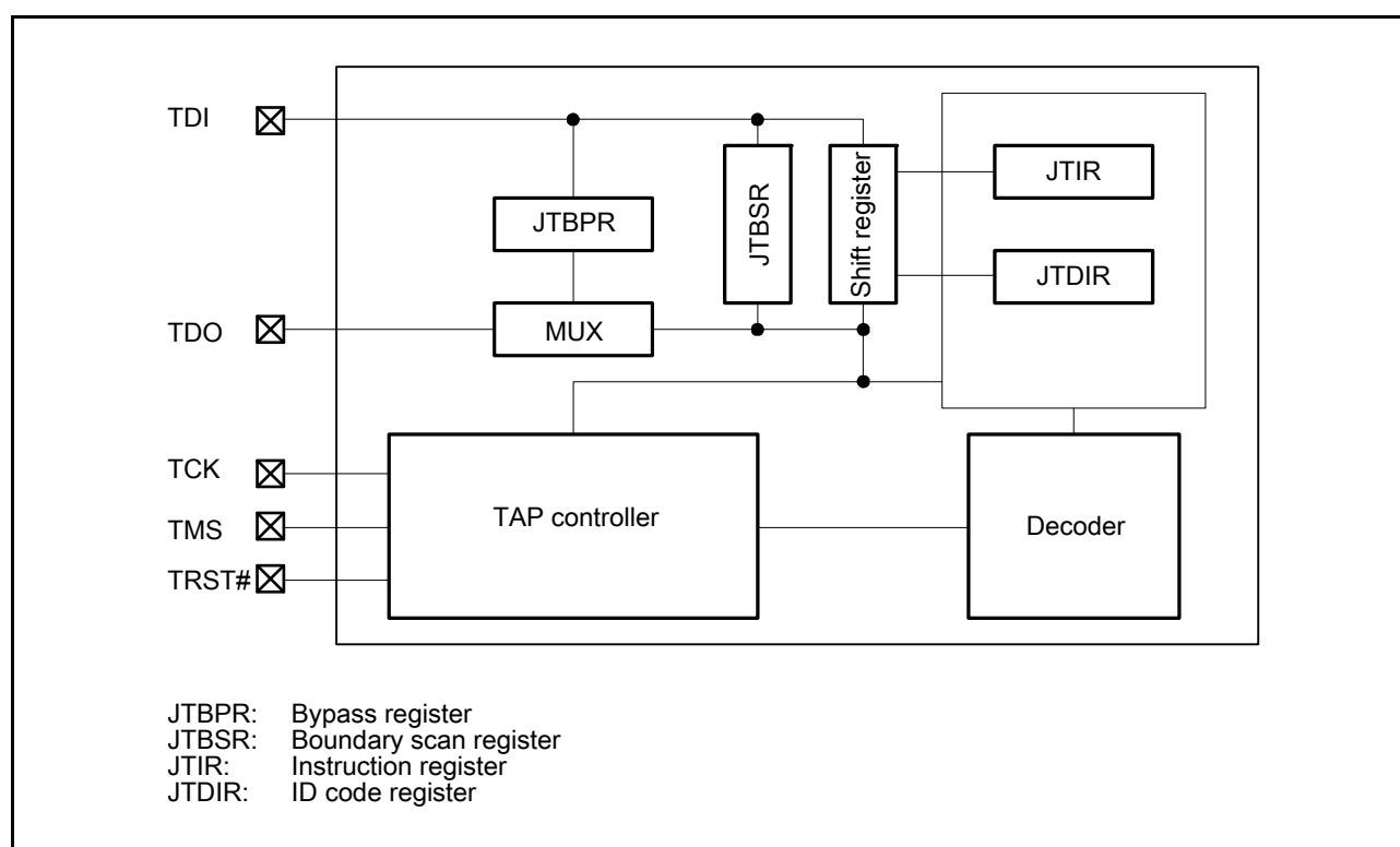
Figure 44.1 Block Diagram of JTAG
