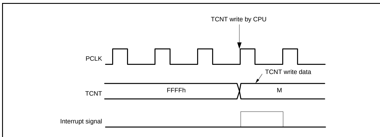
Figure 24.53 Conflict between TPUm.TCNT Write and Overflow
