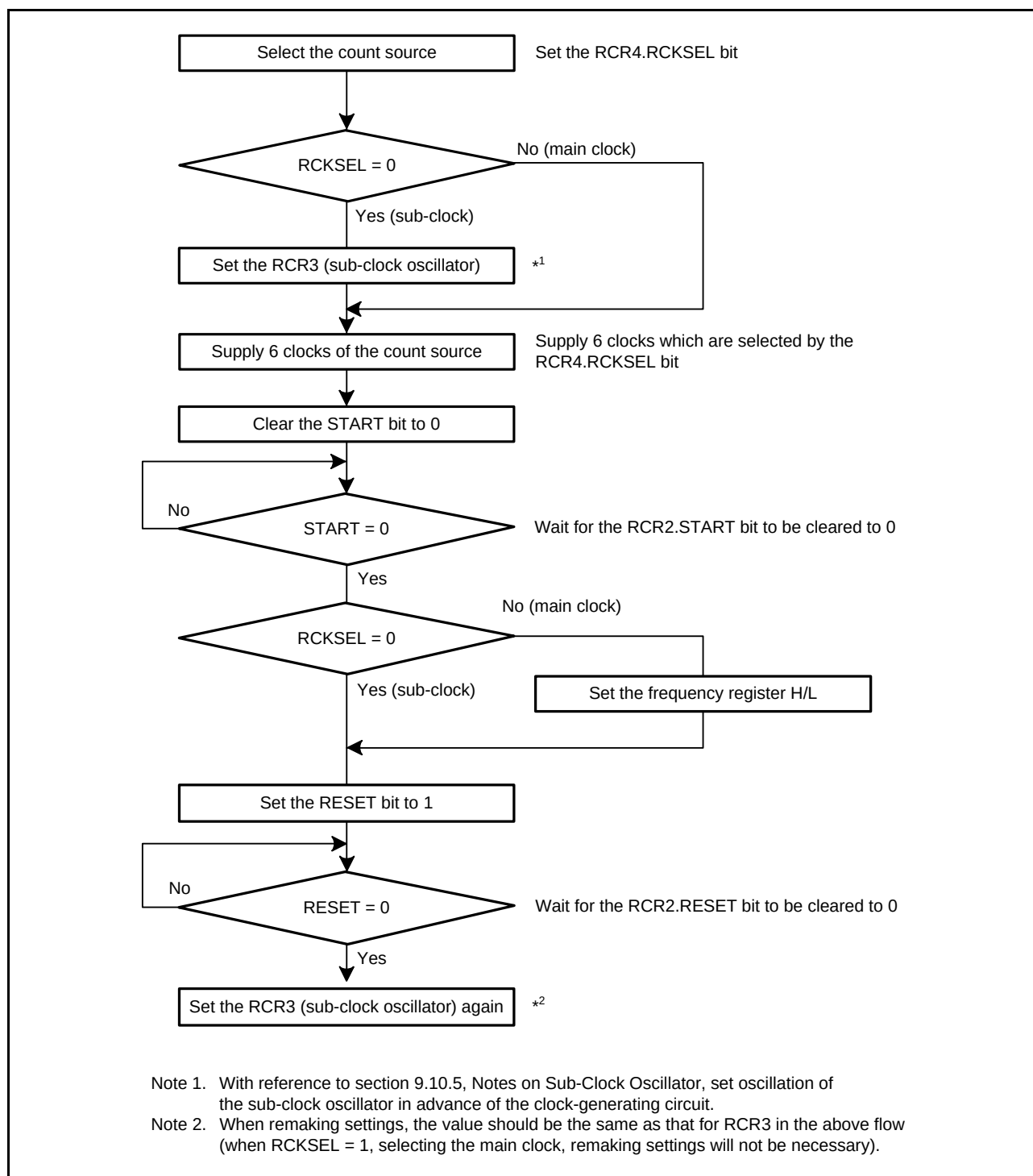
Figure 28.3 Clock Setting Procedure
