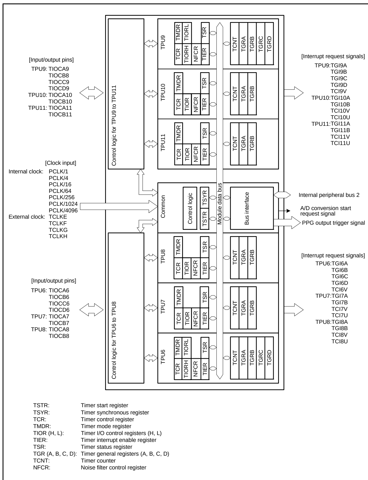
Figure 24.2 Block Diagram of TPU (Unit 1)
