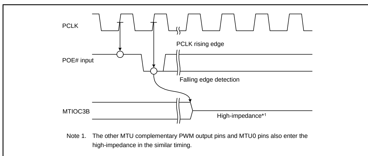
Figure 23.2 Falling Edge Detection
