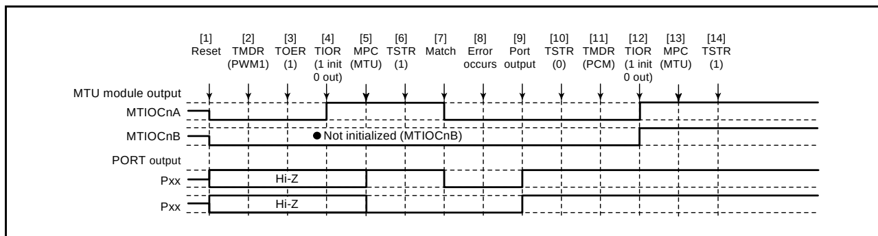
Figure 22.134 Error Occurrence in PWM Mode 1, Recovery in Phase Counting Mode
