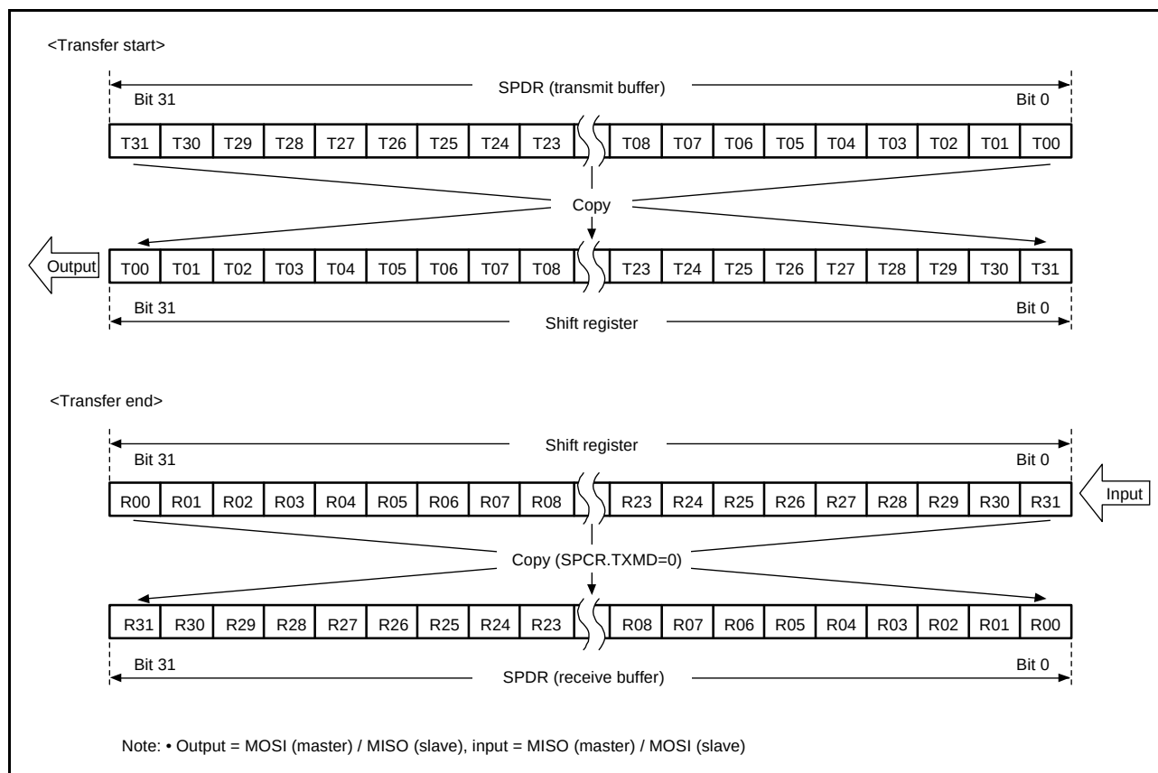
Figure 35.17 LSB-First Transfer (32-Bit Data, Parity Disabled)
