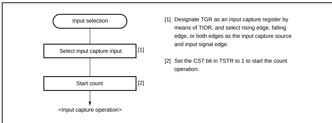
Figure 22.10 Example of Input Capture Operation Setting Procedure
