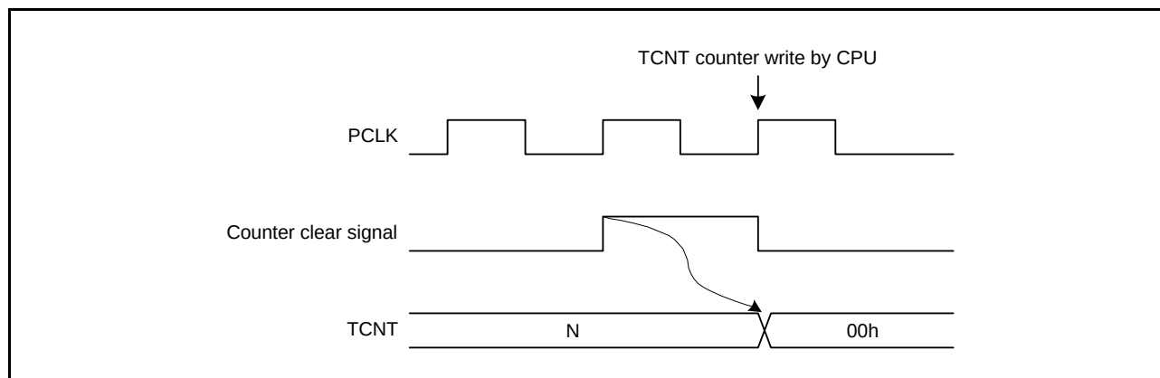
Figure 26.13 Conflict between TCNT Write and Counter Clear
