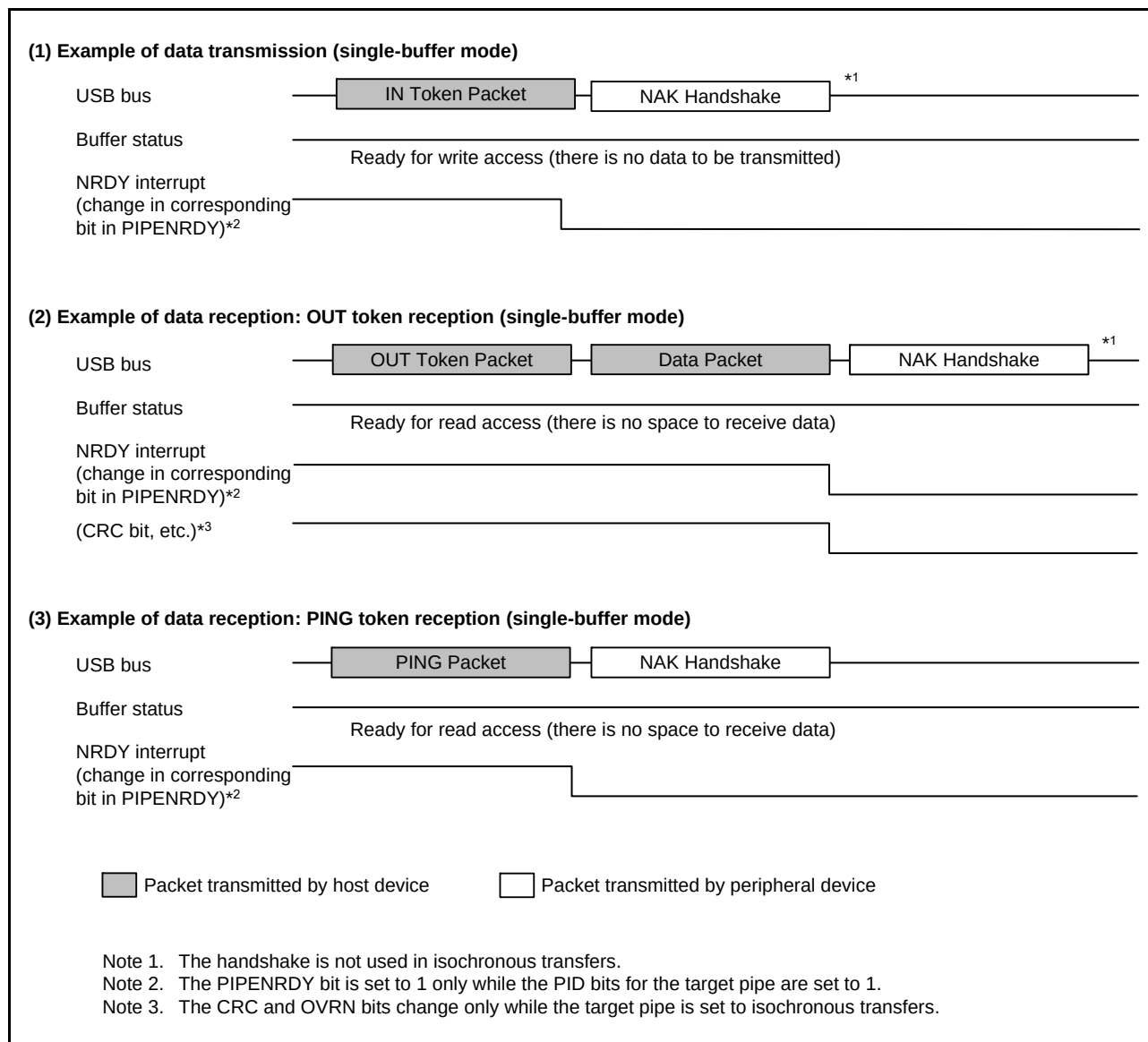
Figure 31.9 Timing of NRDY Interrupt Generation
