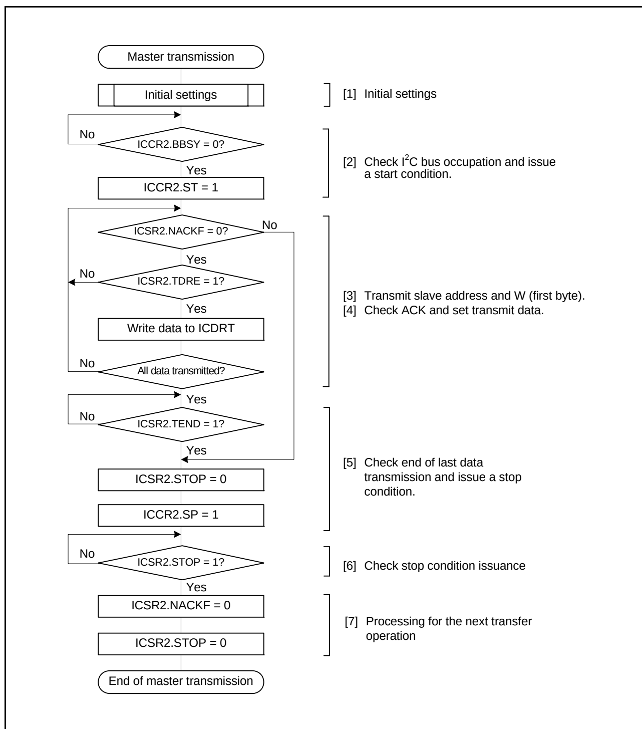
Figure 33.6 Example of Master Transmission Flowchart
