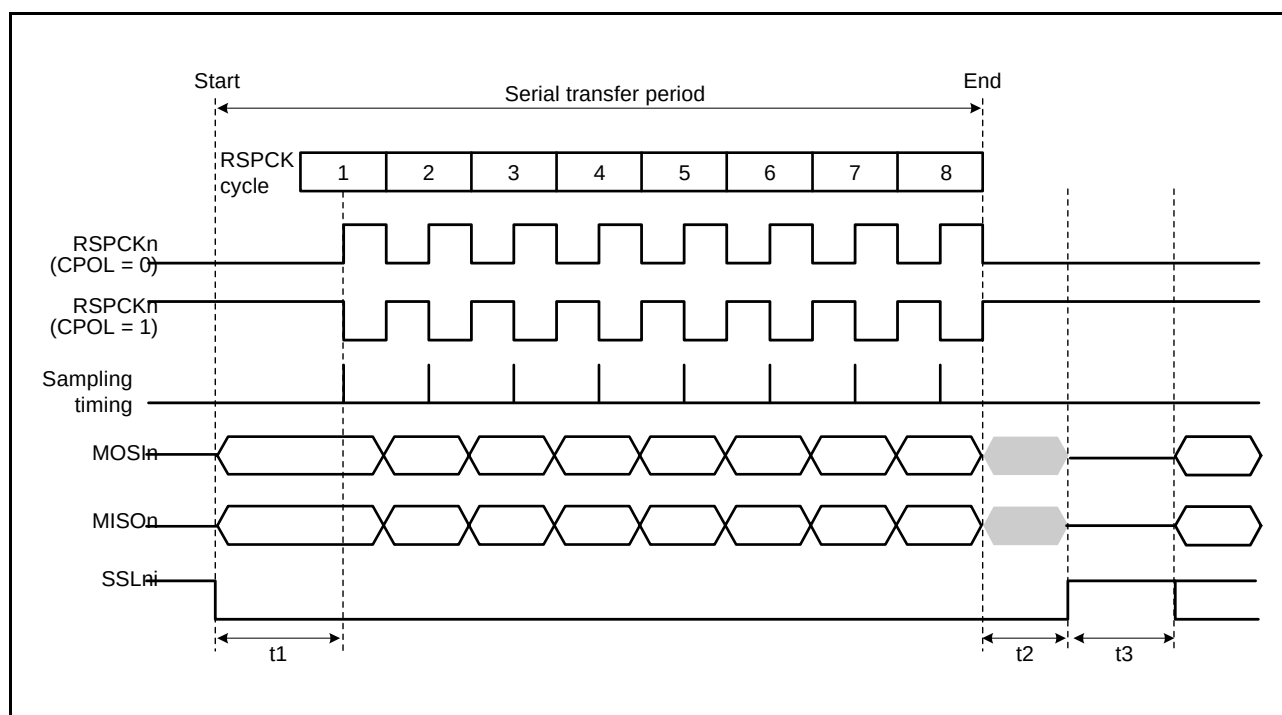
Figure 35.23 RSPI Transfer Format (CPHA = 0)
