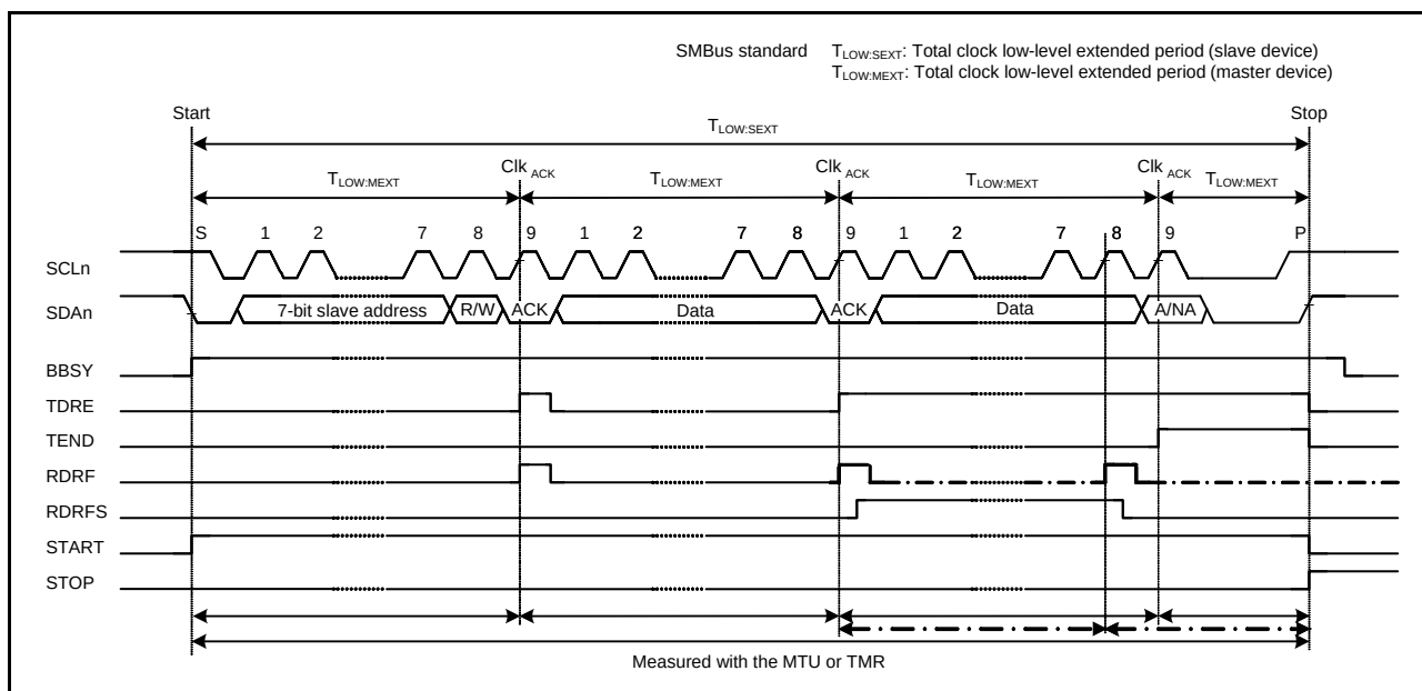
Figure 33.40 SMBus Timeout Measurement
