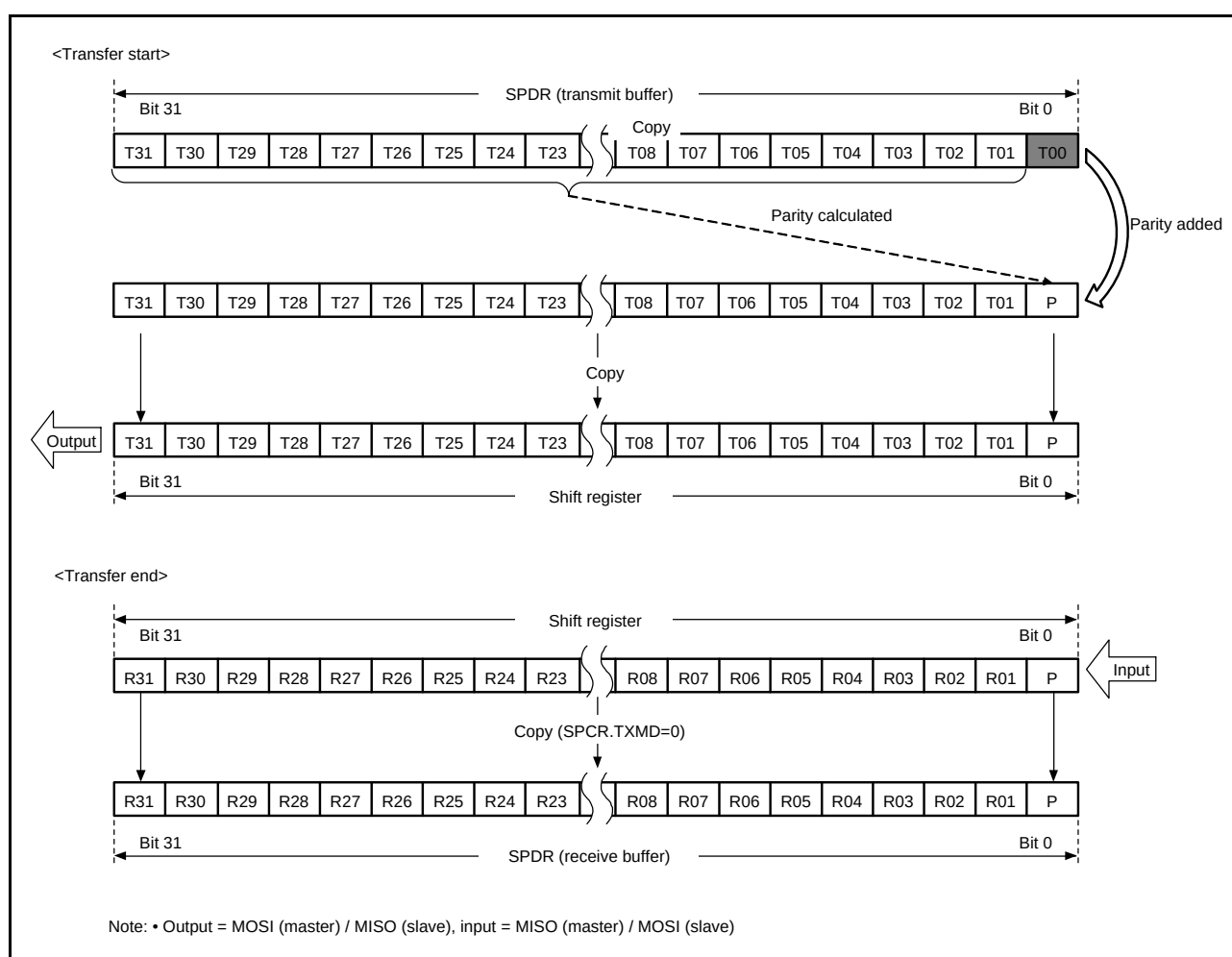
Figure 35.19 MSB-First Transfer (32-Bit Data, Parity Enabled)
