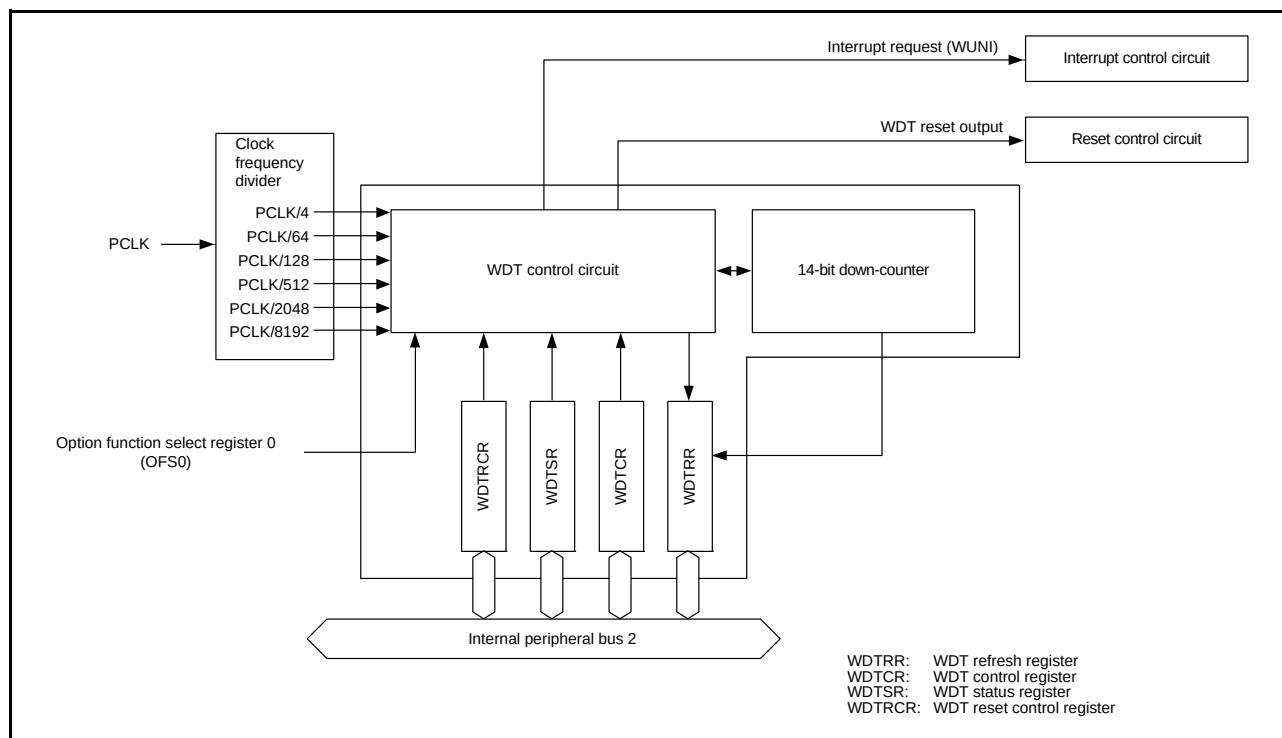
Figure 29.1 Block Diagram of WDT
