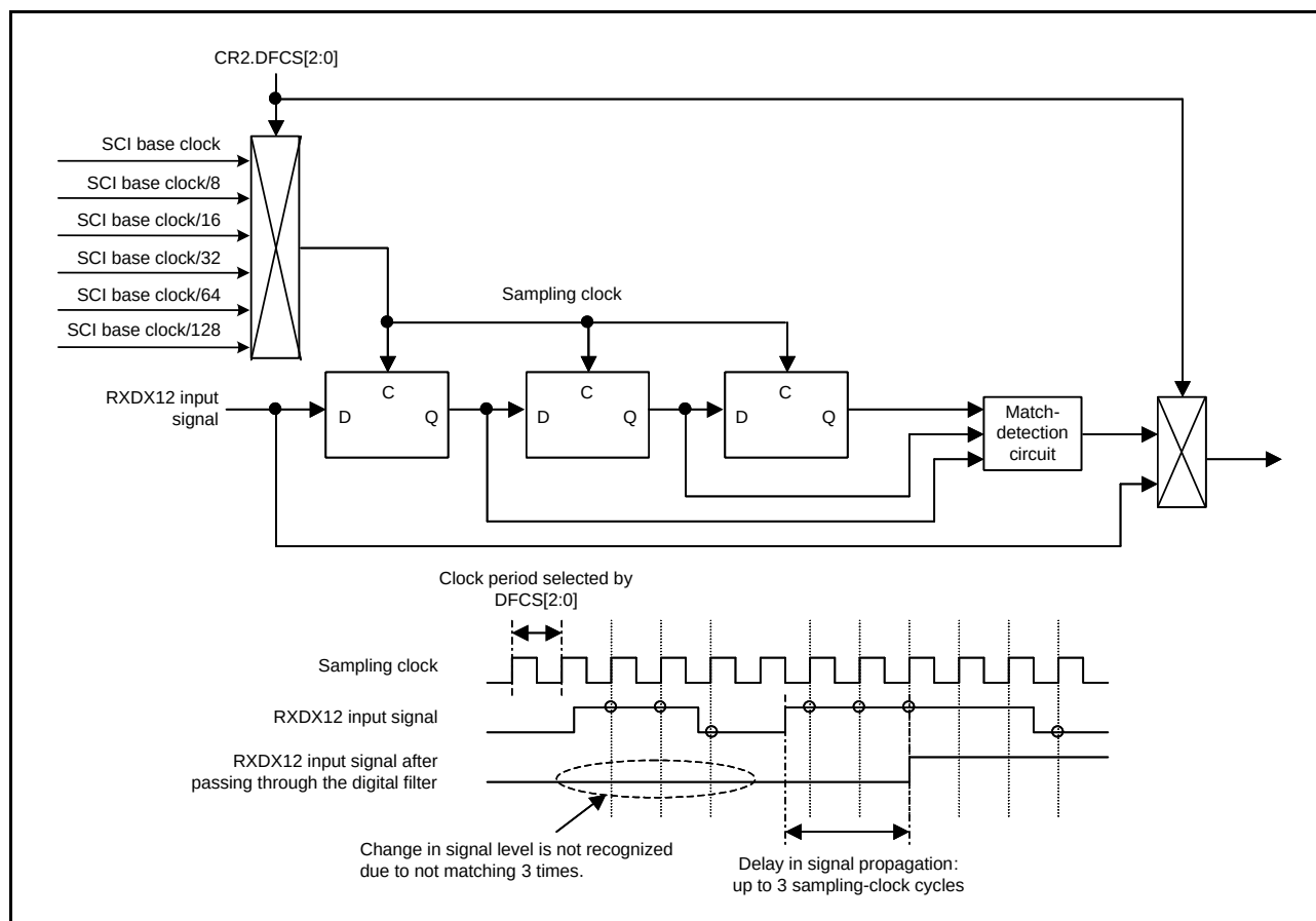
Figure 32.63 Example of Operations with the Digital Filter
