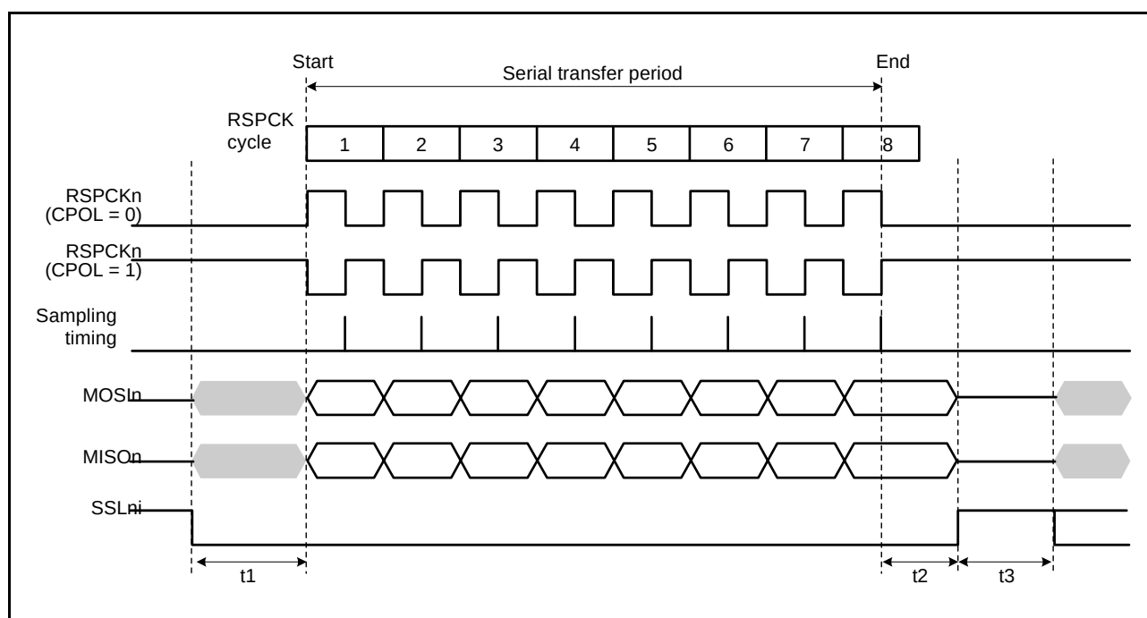
Figure 35.24 RSPi Transfer Format (CPHA = 1)
