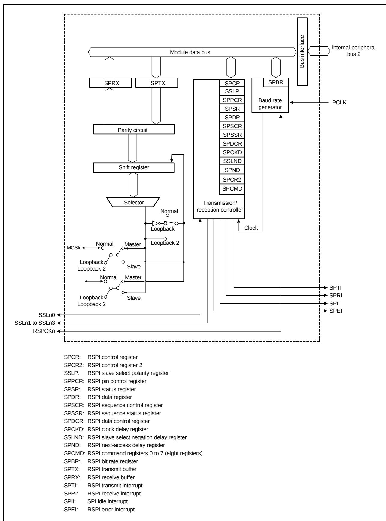
Figure 35.1 Block Diagram of RSPi
