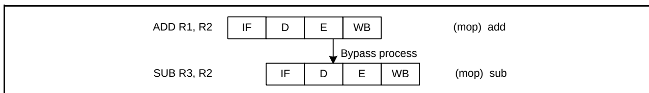
Figure 2.20 Bypass Process
