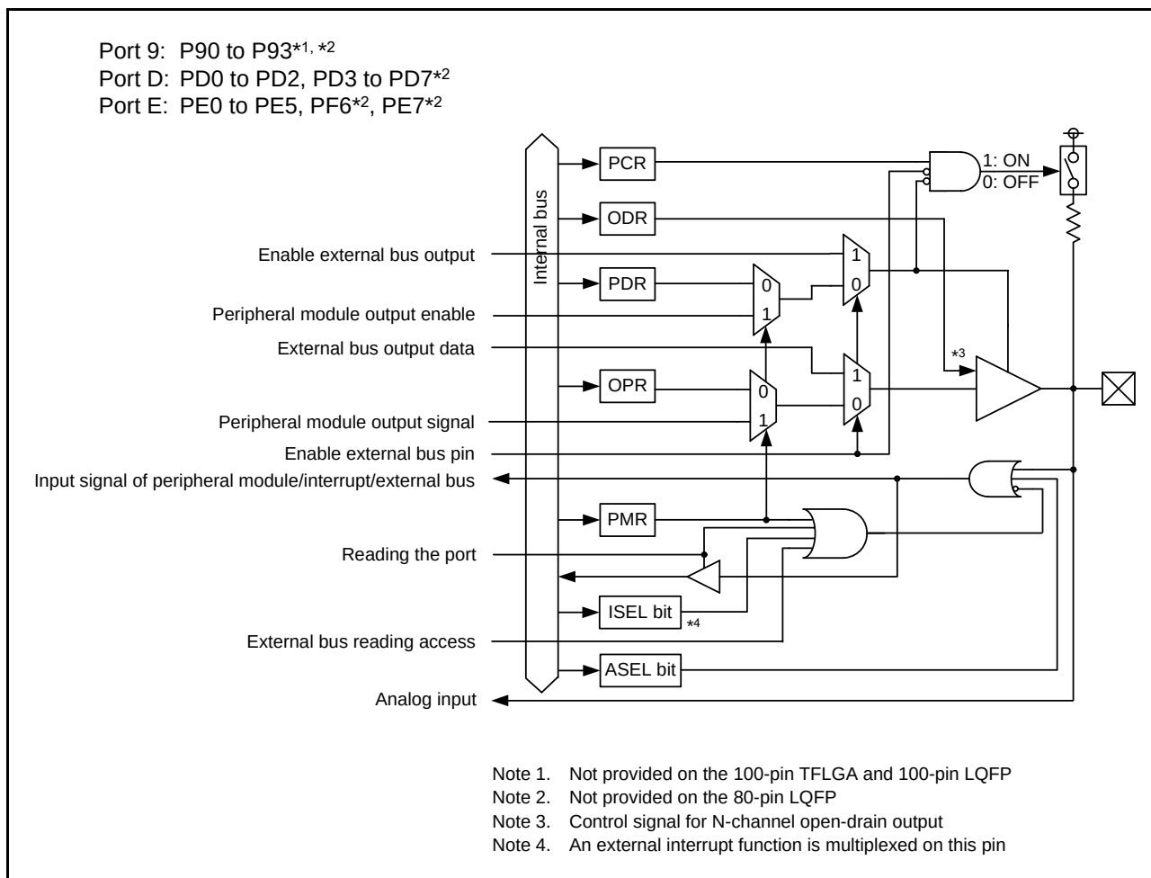
Figure 20.4 I/O Port Configuration (4)
