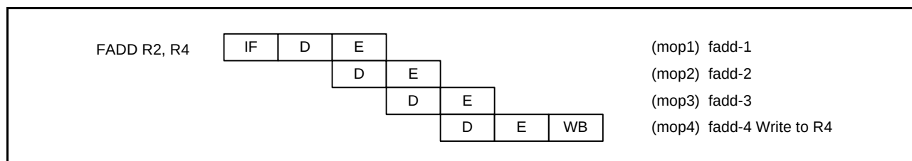
Figure 2.15 Floating-Point Operation Instruction (Register-Register, Immediate-Register)
