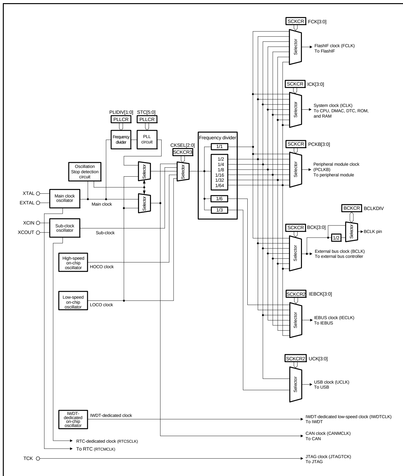
Figure 9.1 Block Diagram of Clock Generation Circuit
