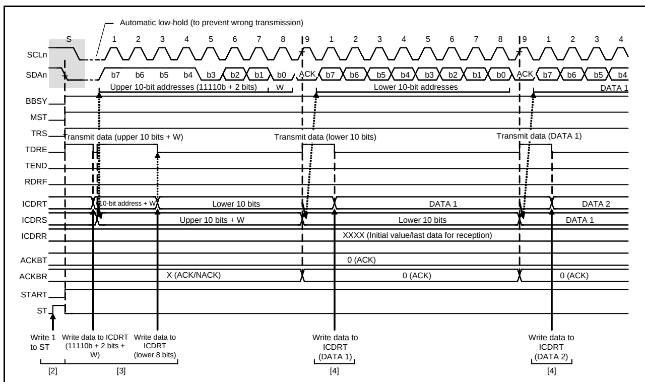
Figure 33.8 Master Transmit Operation Timing (2) (10-Bit Address Format)
