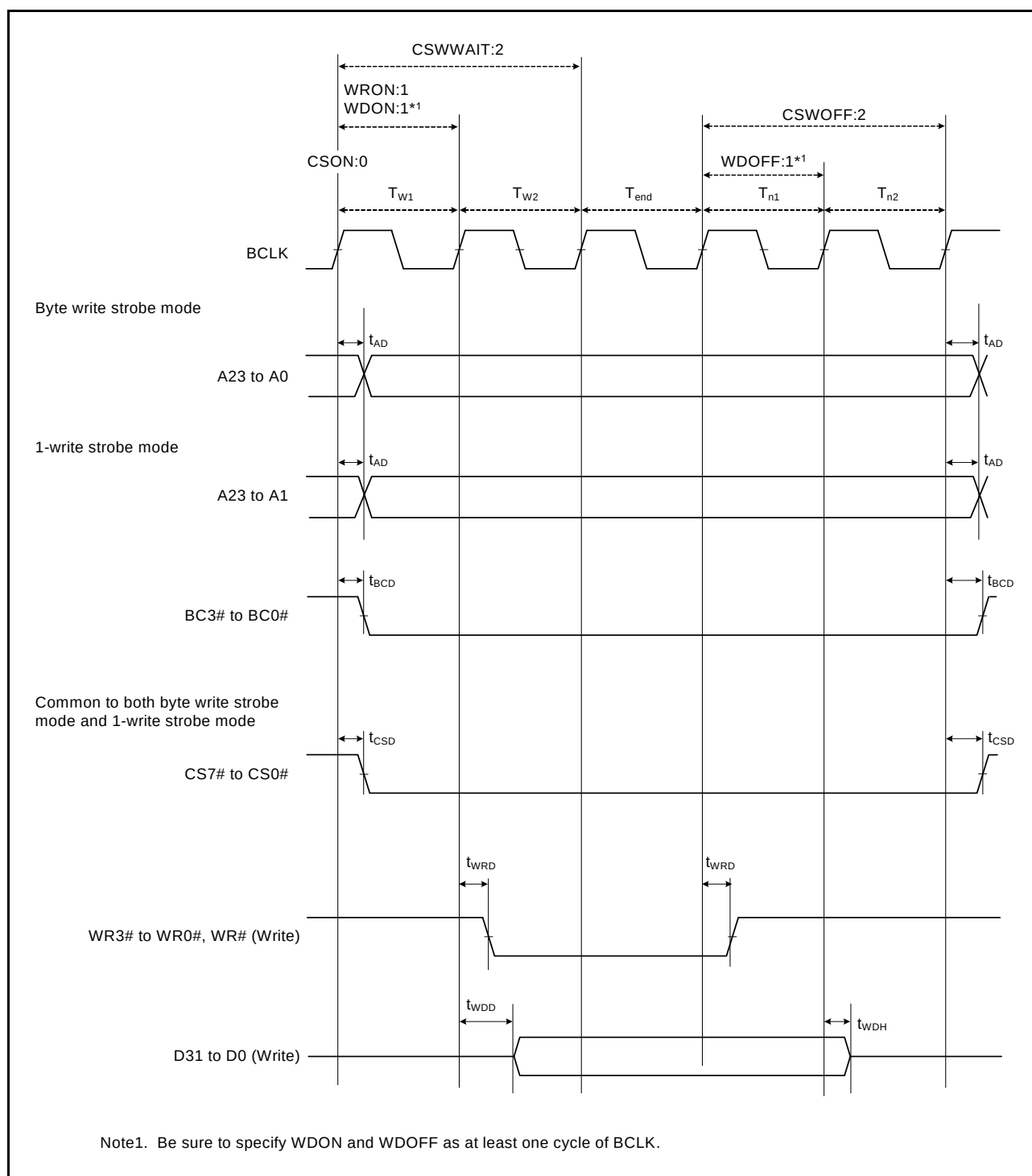
Figure 45.20 External Bus Timing/Normal Write Cycle (Bus Clock Synchronized)
