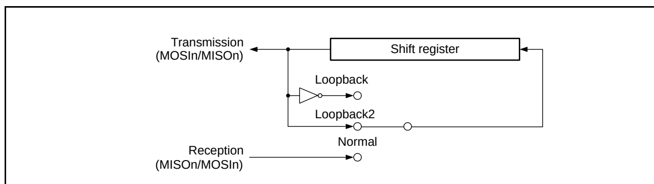
Figure 35.47 Configuration of Shift Register I/O Paths in Loopback Mode (Master Mode)
