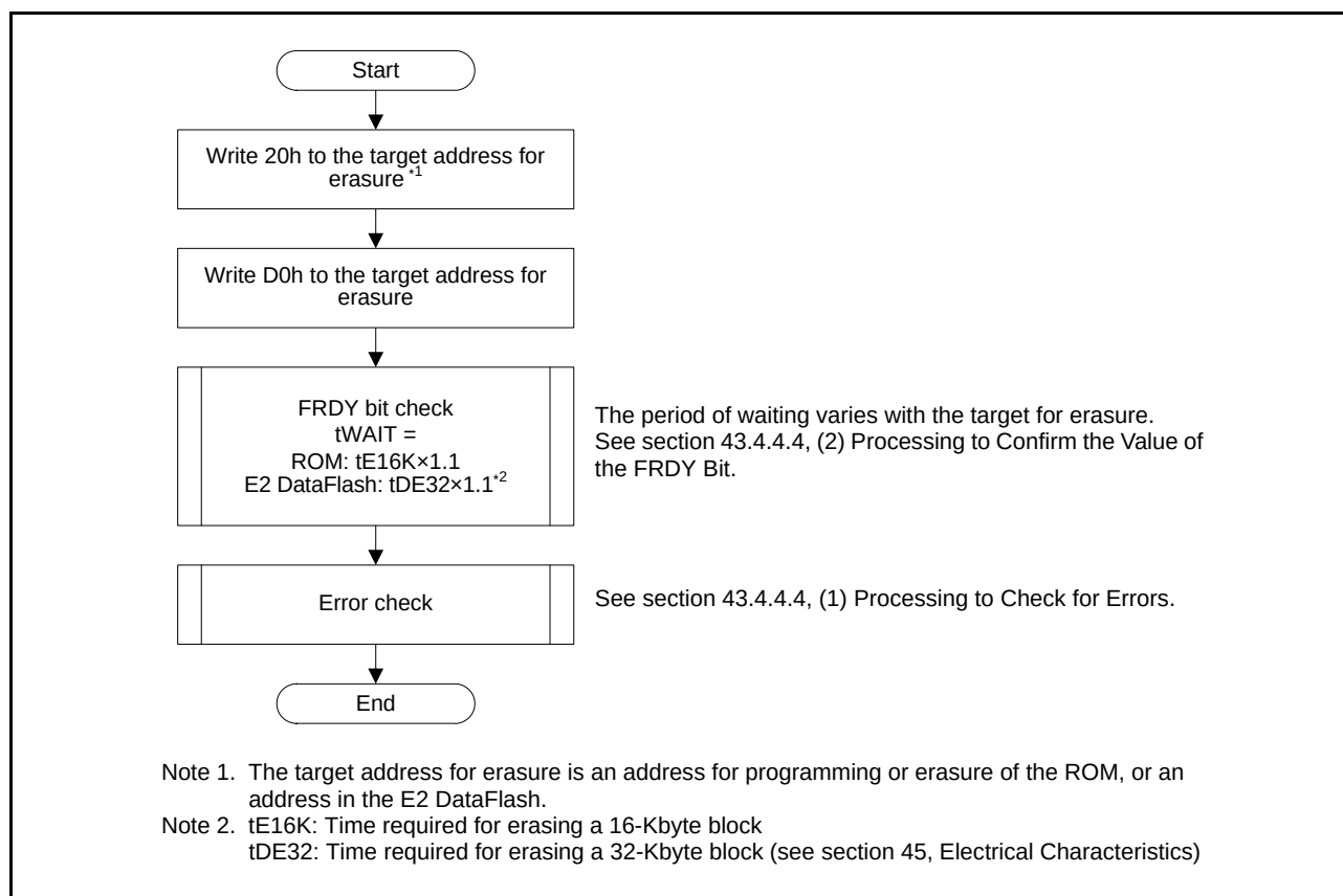
Figure 43.14 Procedure for ROM/E2 DataFlash Erasure
