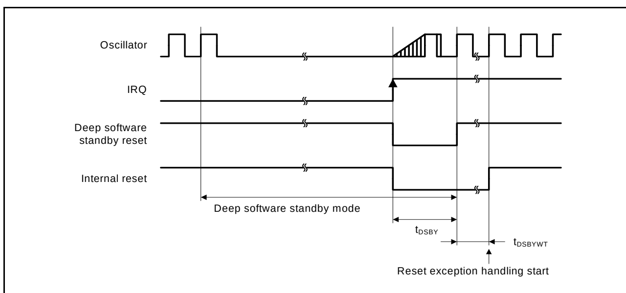
Figure 45.14 Deep Software Standby Mode Cancellation Timing
