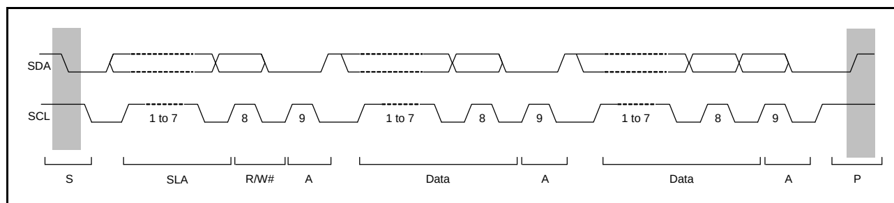
Figure 33.4 I 2 C Bus Timing (SLA = 7 Bits)
