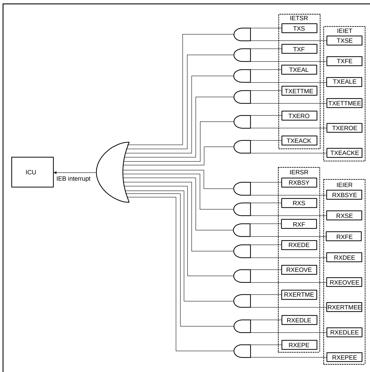
Figure 36.15 Relations between IEB Interrupt Sources
