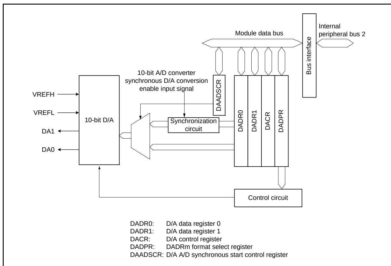
Figure 40.1 Block Diagram of D/A Converter
