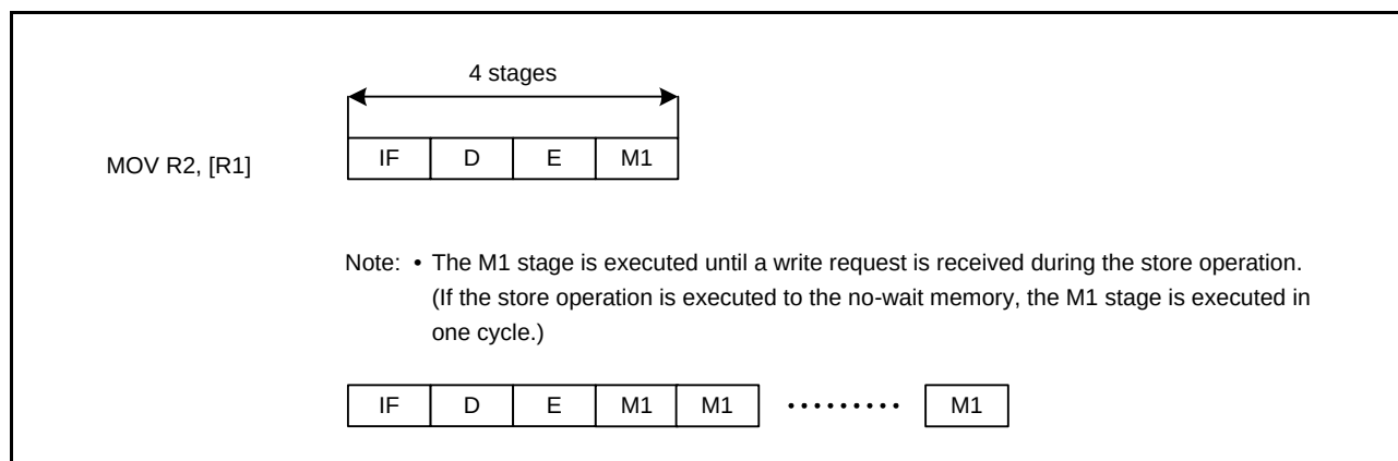
Figure 2.9 Store Operation
