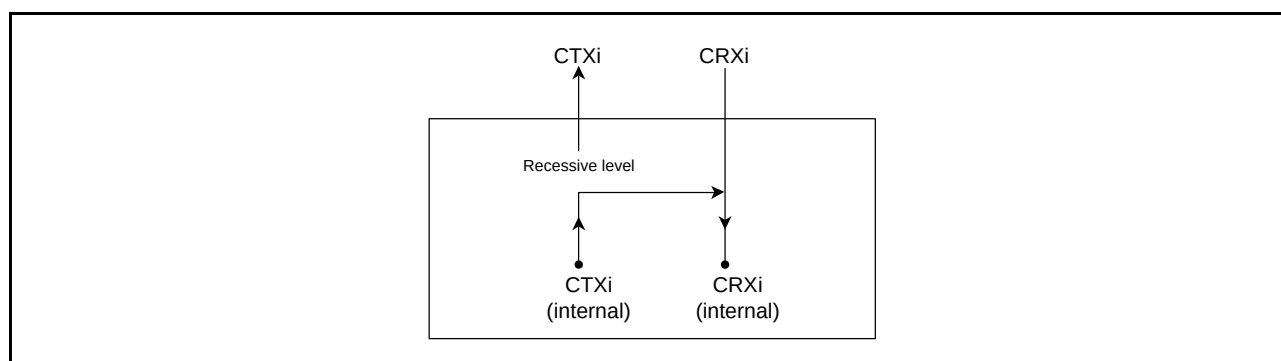
Figure 34.6 Connection when Listen-Only Mode is Selected ( i = 0 to 2)
