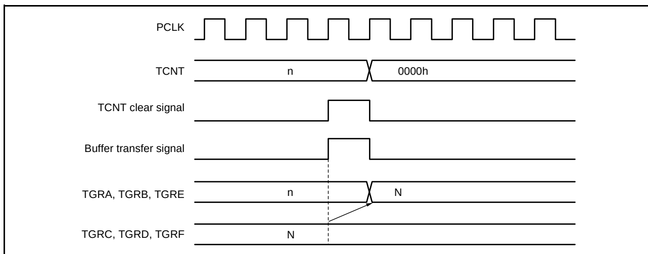
Figure 22.96 Buffer Operation Timing (when TCNT Cleared)
