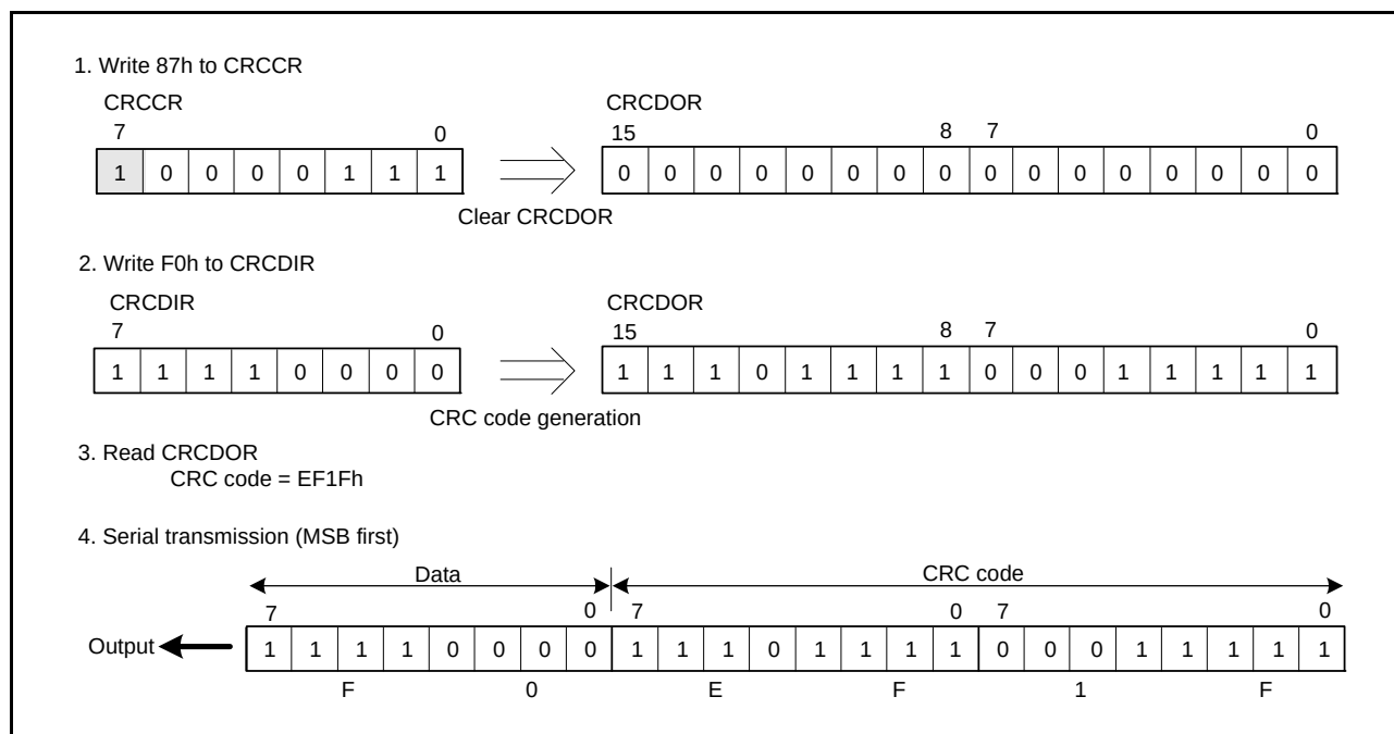
Figure 37.3 MSB-First Data Transmission
