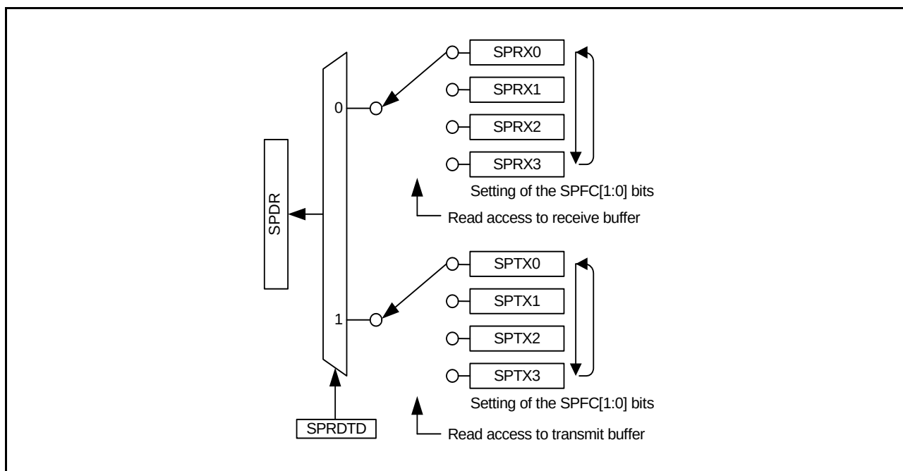
Figure 35.4 Configuration of SPDR (Reading)
