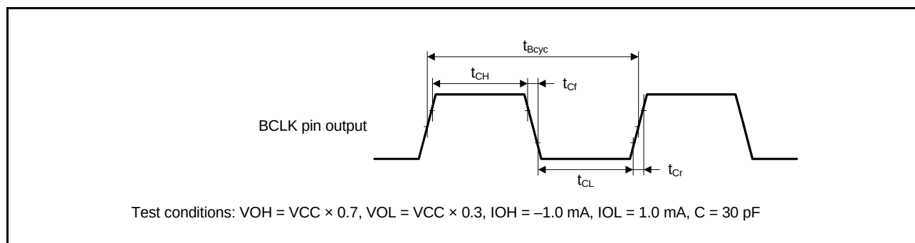
Figure 45.3 BCLK Pin Output Timing
