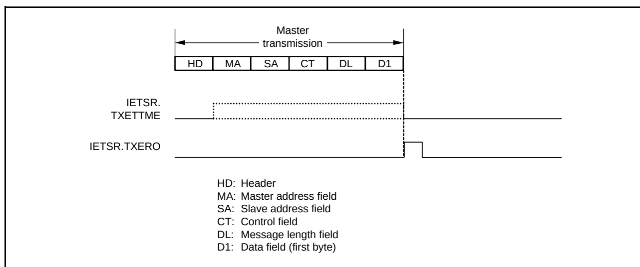
Figure 36.18 Timing of Operations when Transmit Message Length is Greater than Maximum Number of Transfer Bytes
