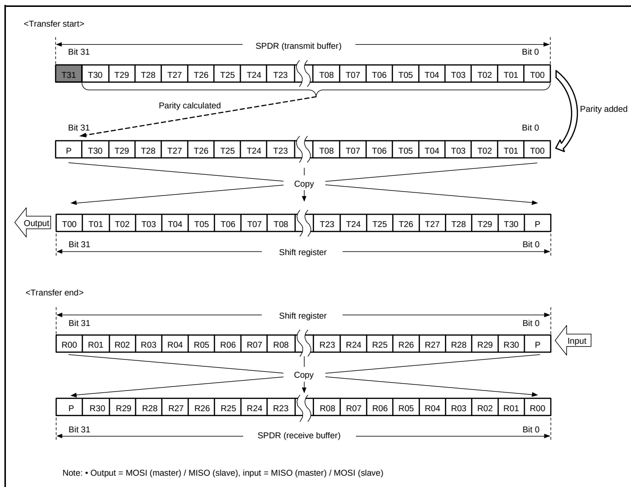
Figure 35.21 LSB-First Transfer (32-Bit Data, Parity Enabled)
