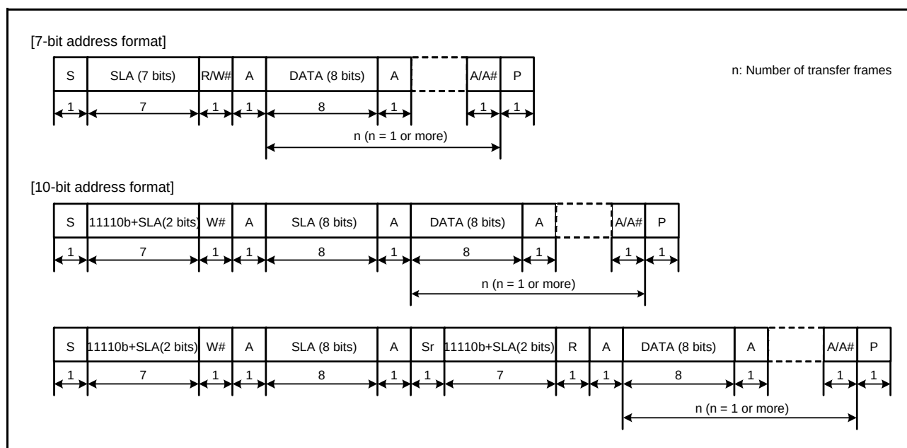
Figure 33.3 I 2 C Bus Format
