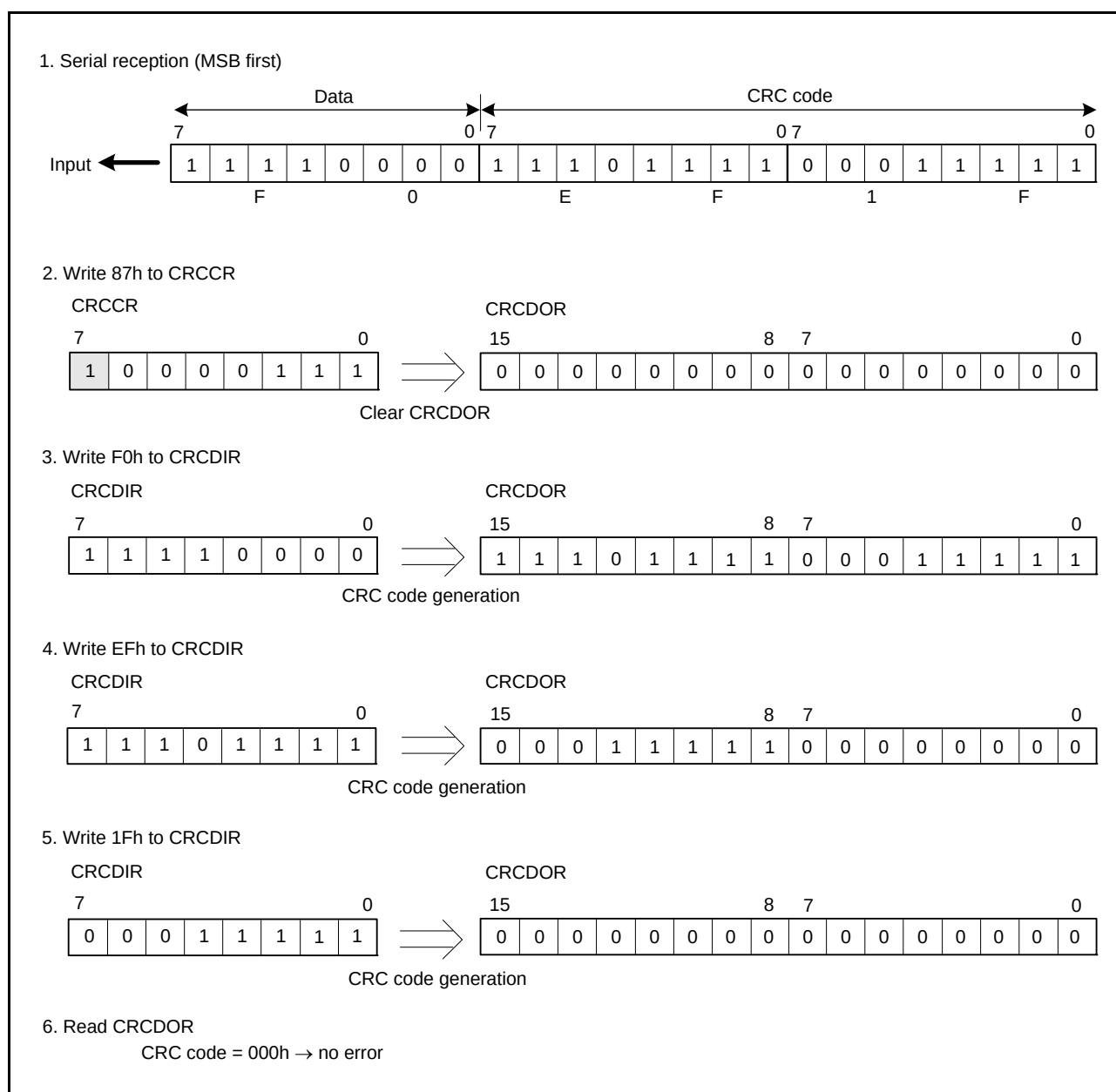
Figure 37.5 MSB-First Data Reception
