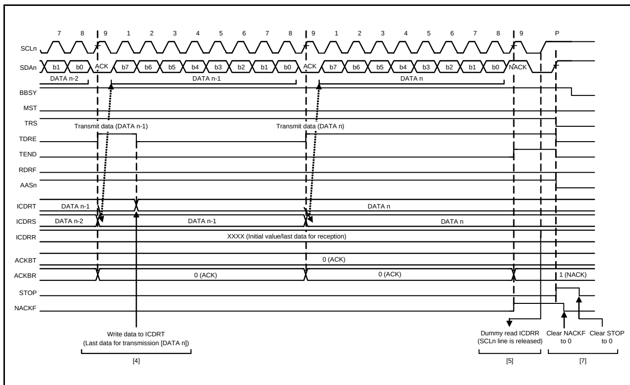
Figure 33.16 Slave Transmit Operation Timing (2)
