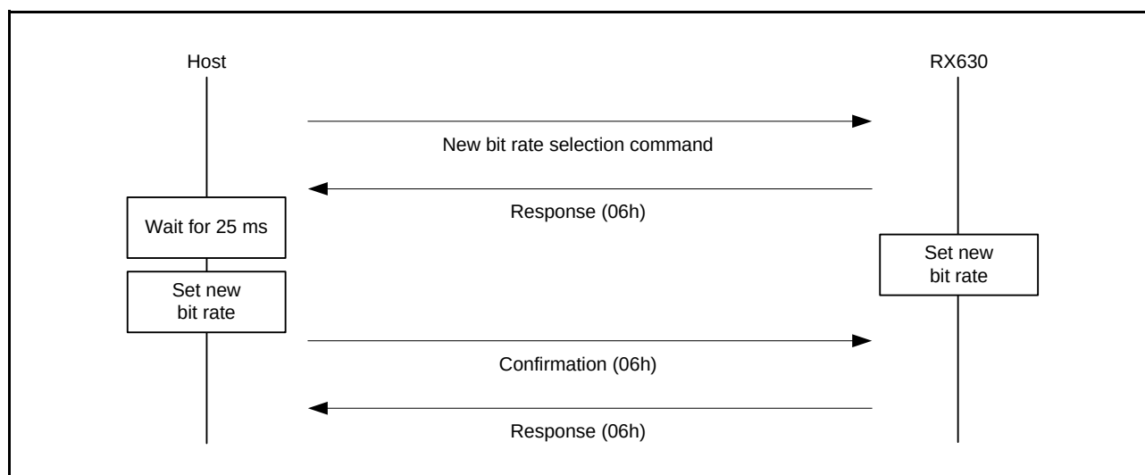
Figure 43.32 New Bit Rate Selection Sequence
