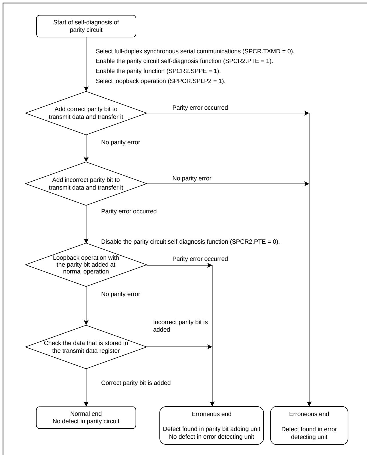
Figure 35.48 Flowchart for Self-Diagnosis of Parity Circuit
