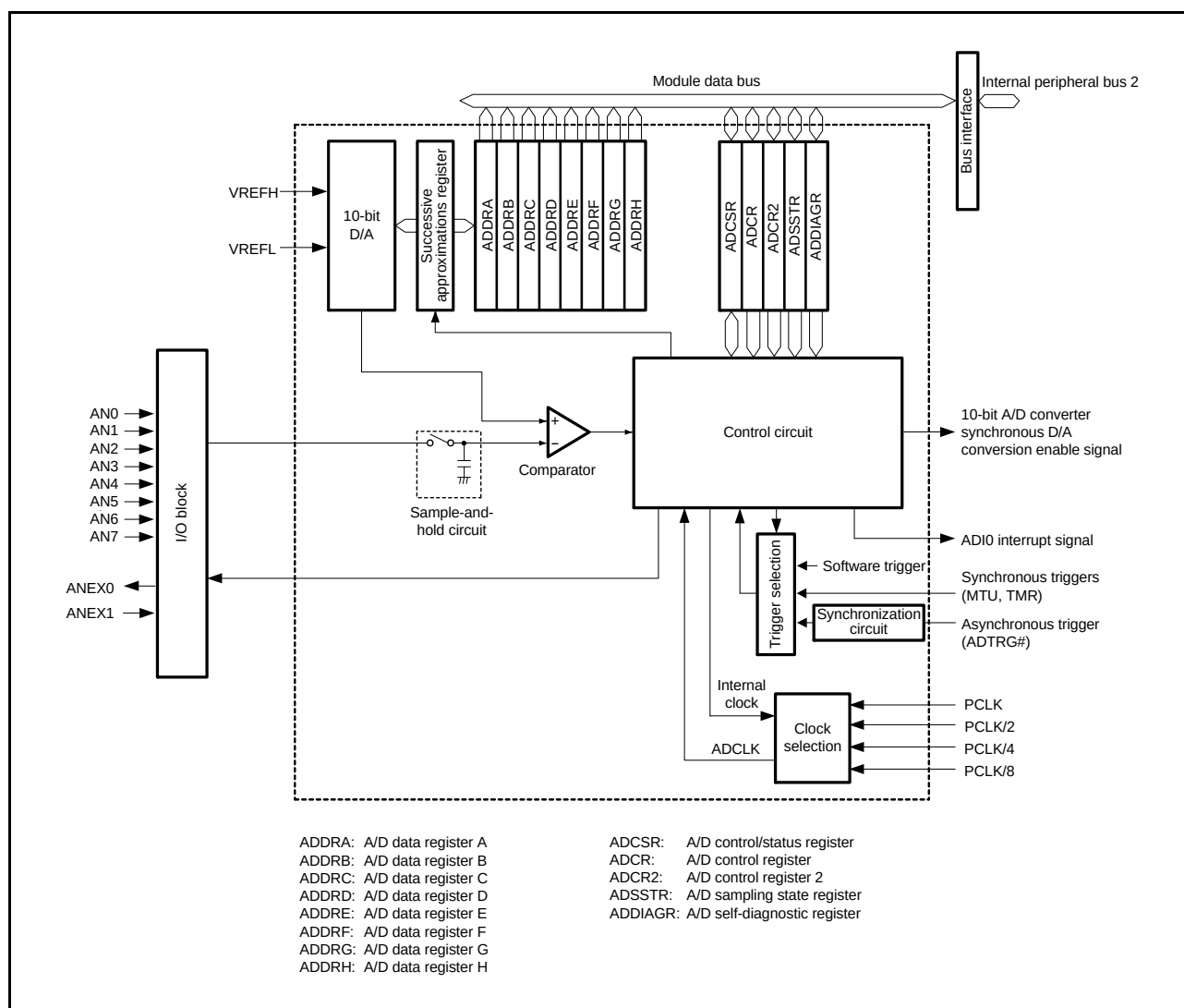
Figure 39.1 Block Diagram of 10-Bit A/D Converter
