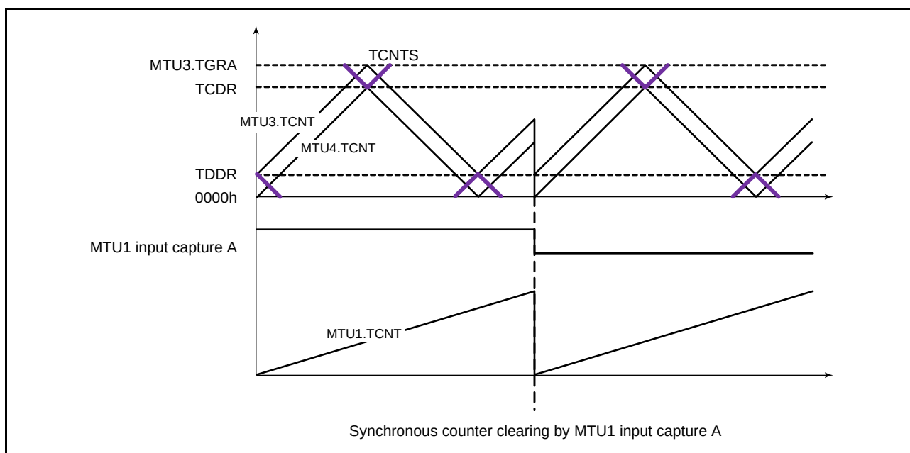
Figure 22.55 Counter Clearing Synchronized with Another Channel
