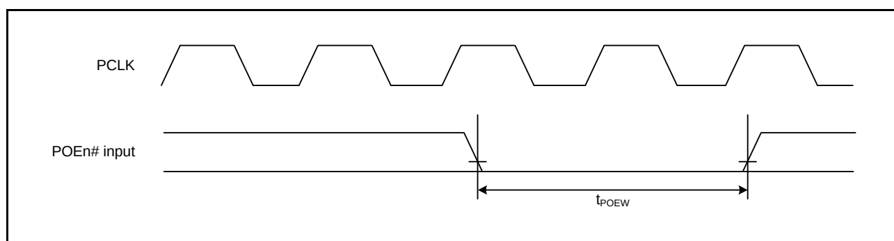
Figure 45.27 POE# Input Timing
