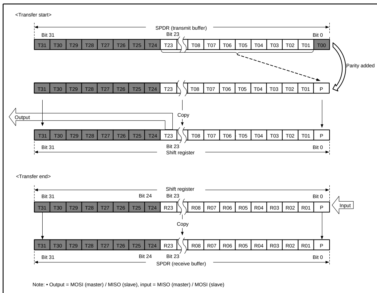
Figure 35.20 MSB-First Transfer (24-Bit Data, Parity Enabled)
