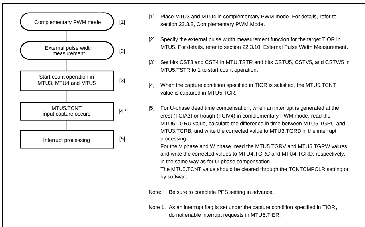
Figure 22.80 Example of Dead Time Compensation Setting Procedure
