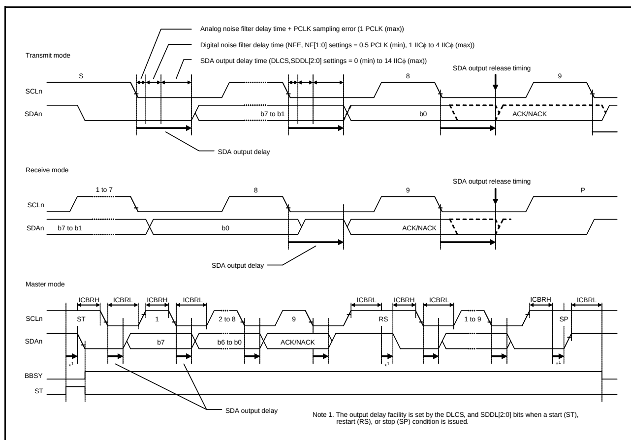
Figure 33.21 SDA Output Delay Facility
