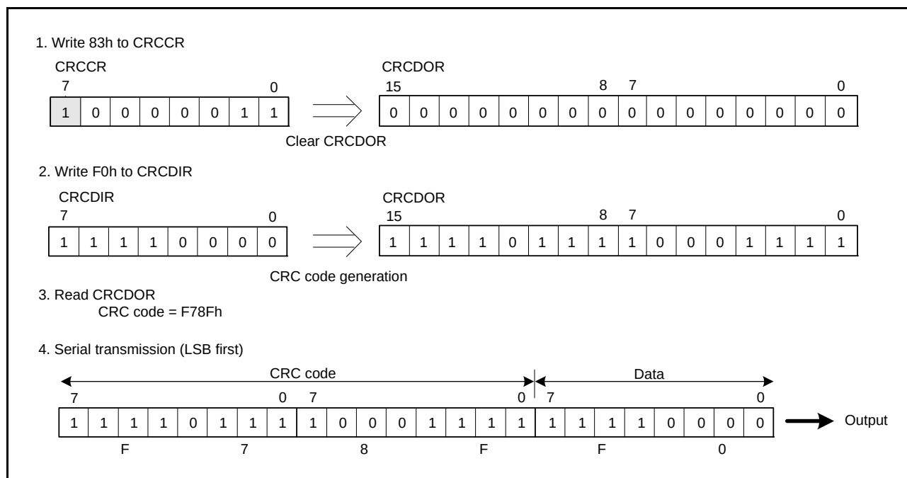
Figure 37.2 LSB-First Data Transmission
