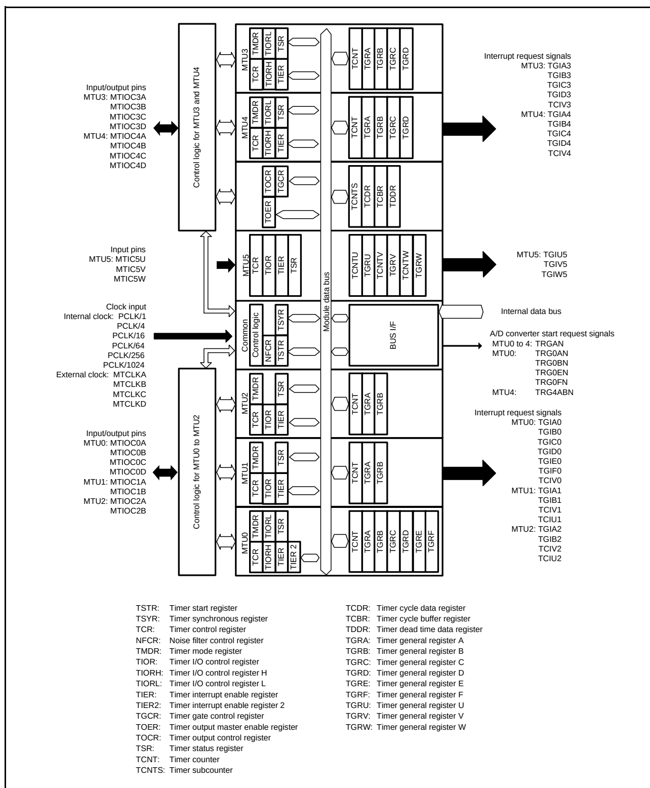
Figure 22.1 Block Diagram of MTU
