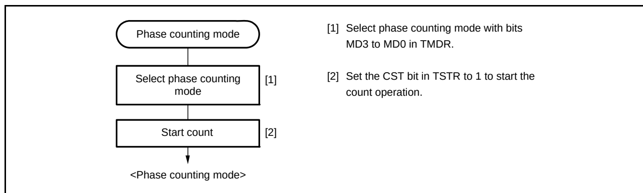
Figure 22.29 Example of Phase Counting Mode Setting Procedure
