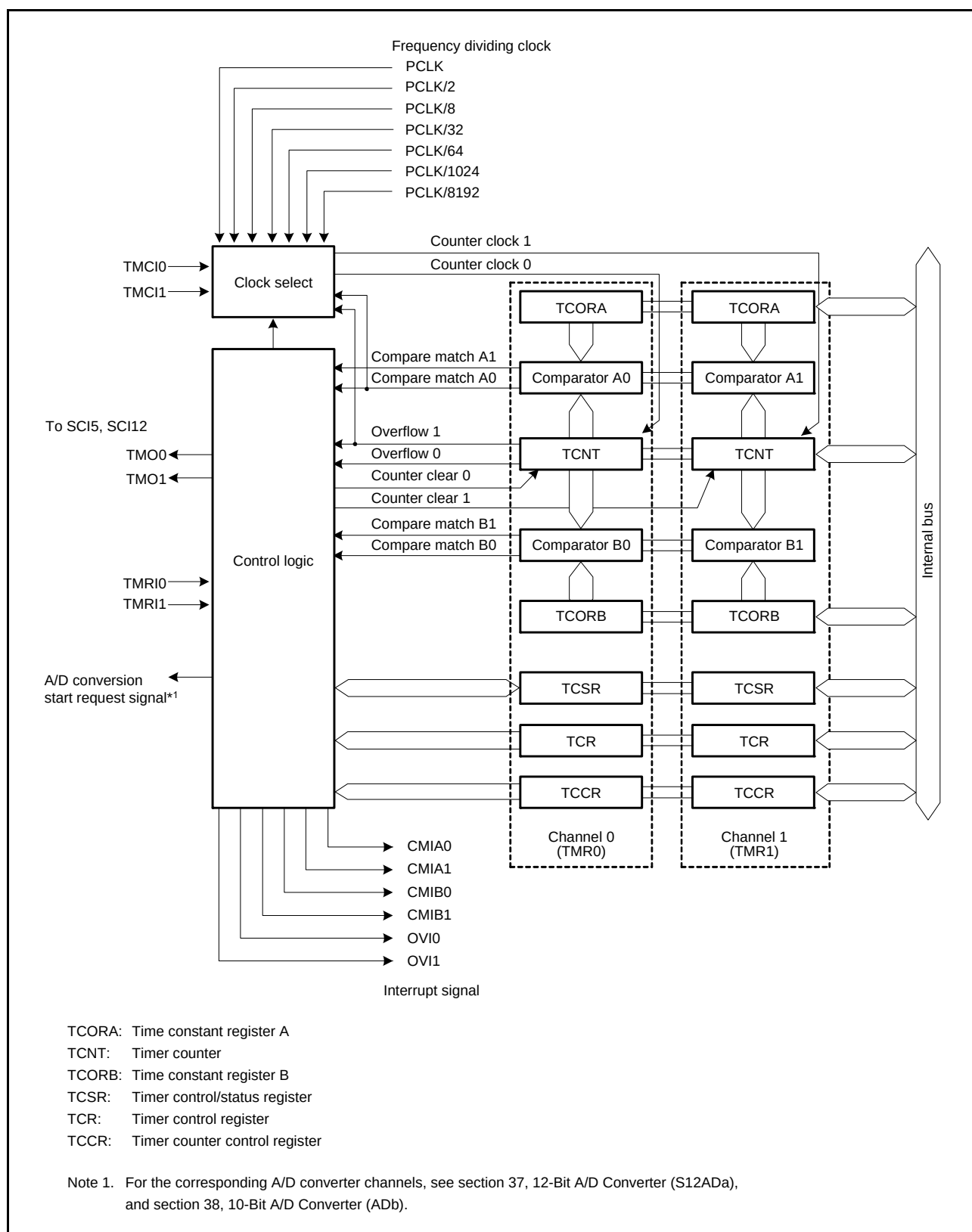
Figure 26.1 Block Diagram of TMR (Unit 0)
