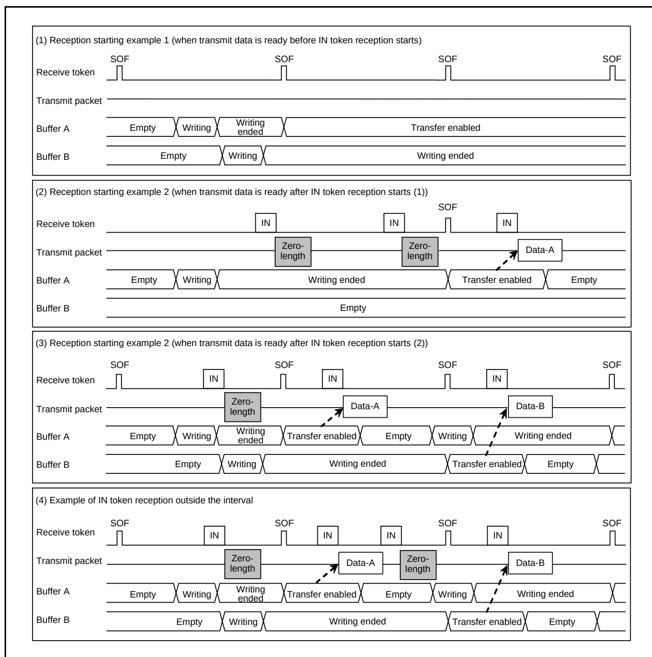
Figure 31.15 Example of Data Setup Function Operation
