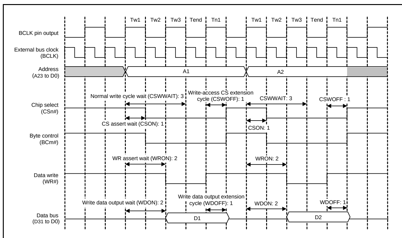
Figure 16.21 Example of Normal-Write Operation (when 1/2 BCLK is Selected with the BCLK Pin Output Select Bit) (n = 0 to 7, m = 0 to 3)
