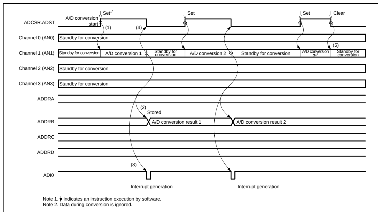
Figure 39.2 Example of 10-Bit A/D Converter Operation (Single Channel Mode)
