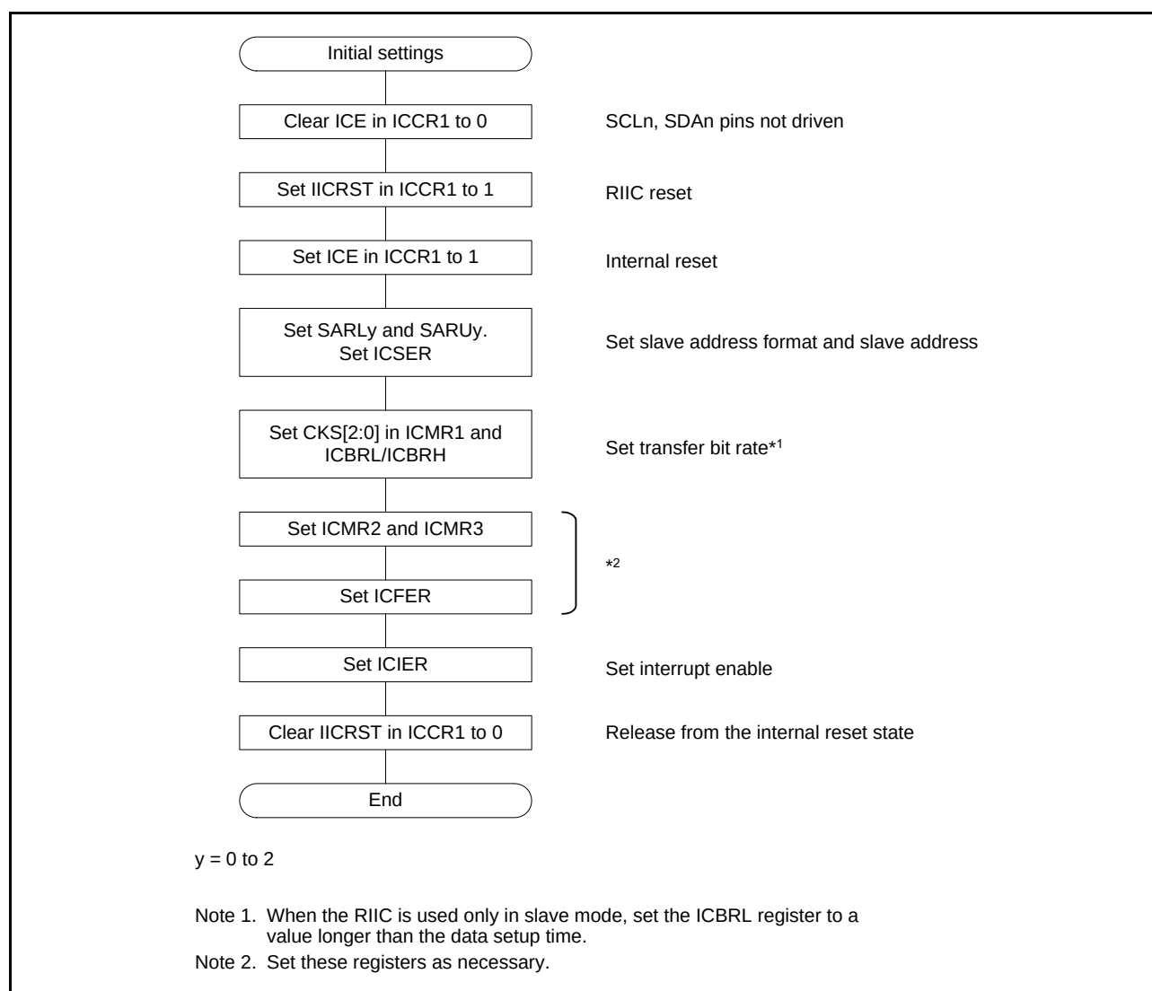
Figure 33.5 Example of RIIC Initialization Flowchart
