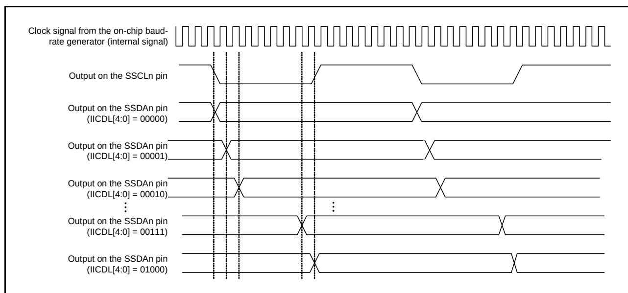
Figure 32.44 Timing of Delays in SSDA Output
