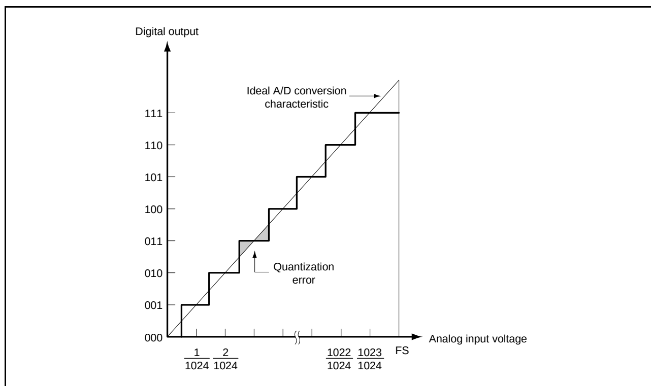
Figure 39.14 A/D Conversion Accuracy Definitions (1)
