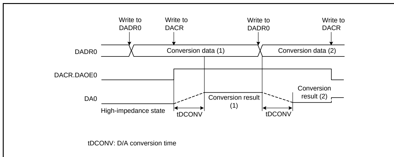
Figure 40.2 Example of D/A Converter Operation
