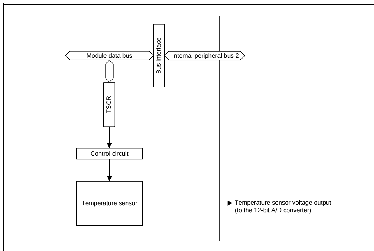
Figure 41.1 Block Diagram of Temperature Sensor
