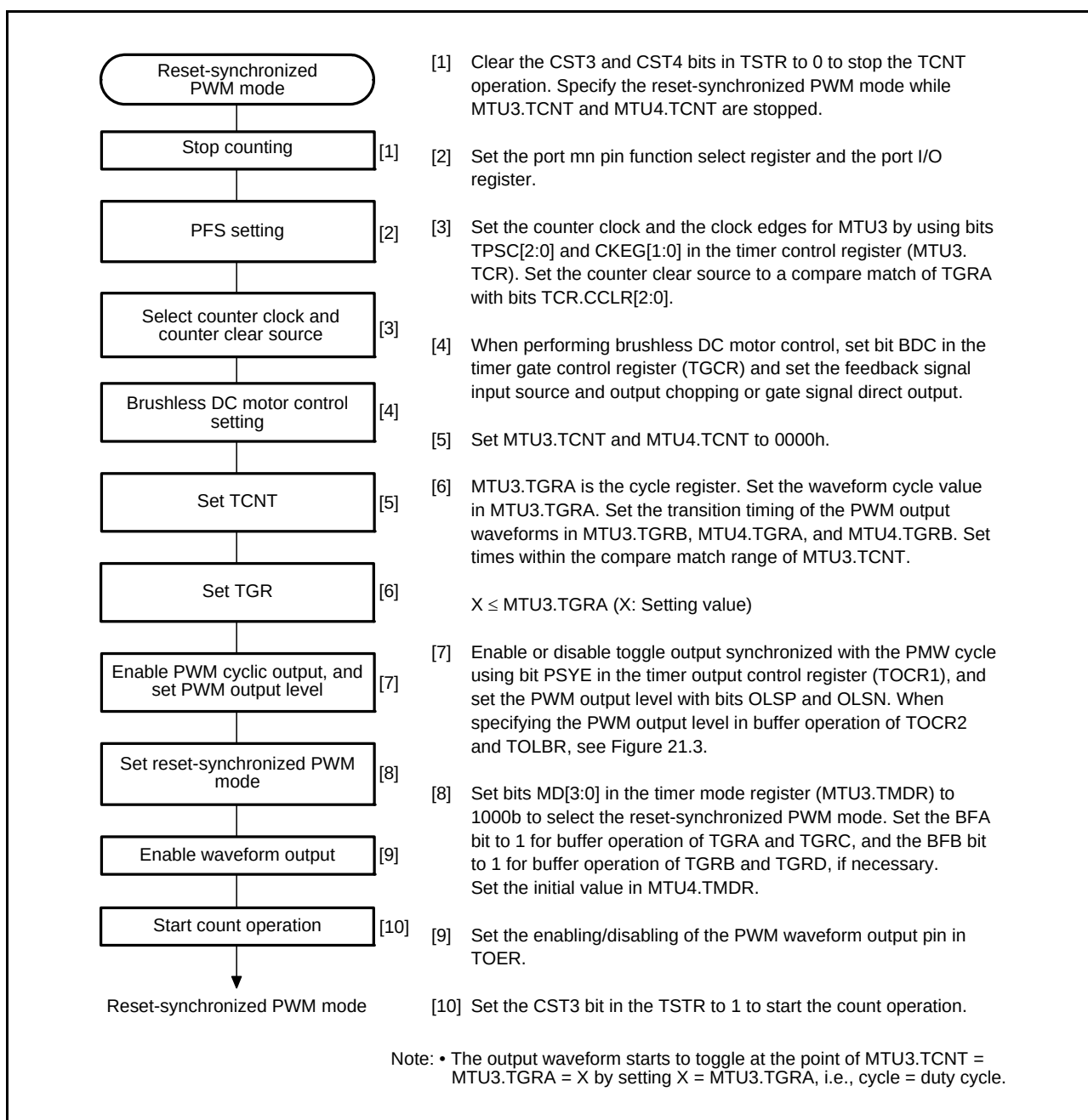
Figure 22.35 Procedure for Selecting Reset-Synchronized PWM Mode
