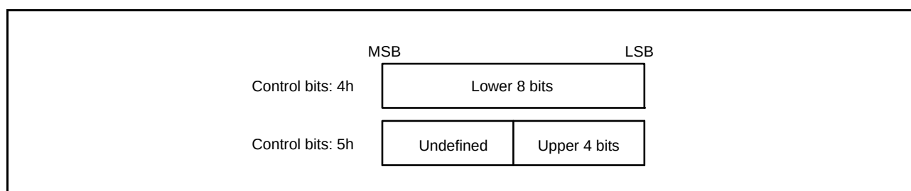
Figure 36.2 Locked Address Configuration
