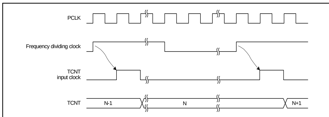
Figure 26.5 Count Timing for Frequency Dividing Clock Input
