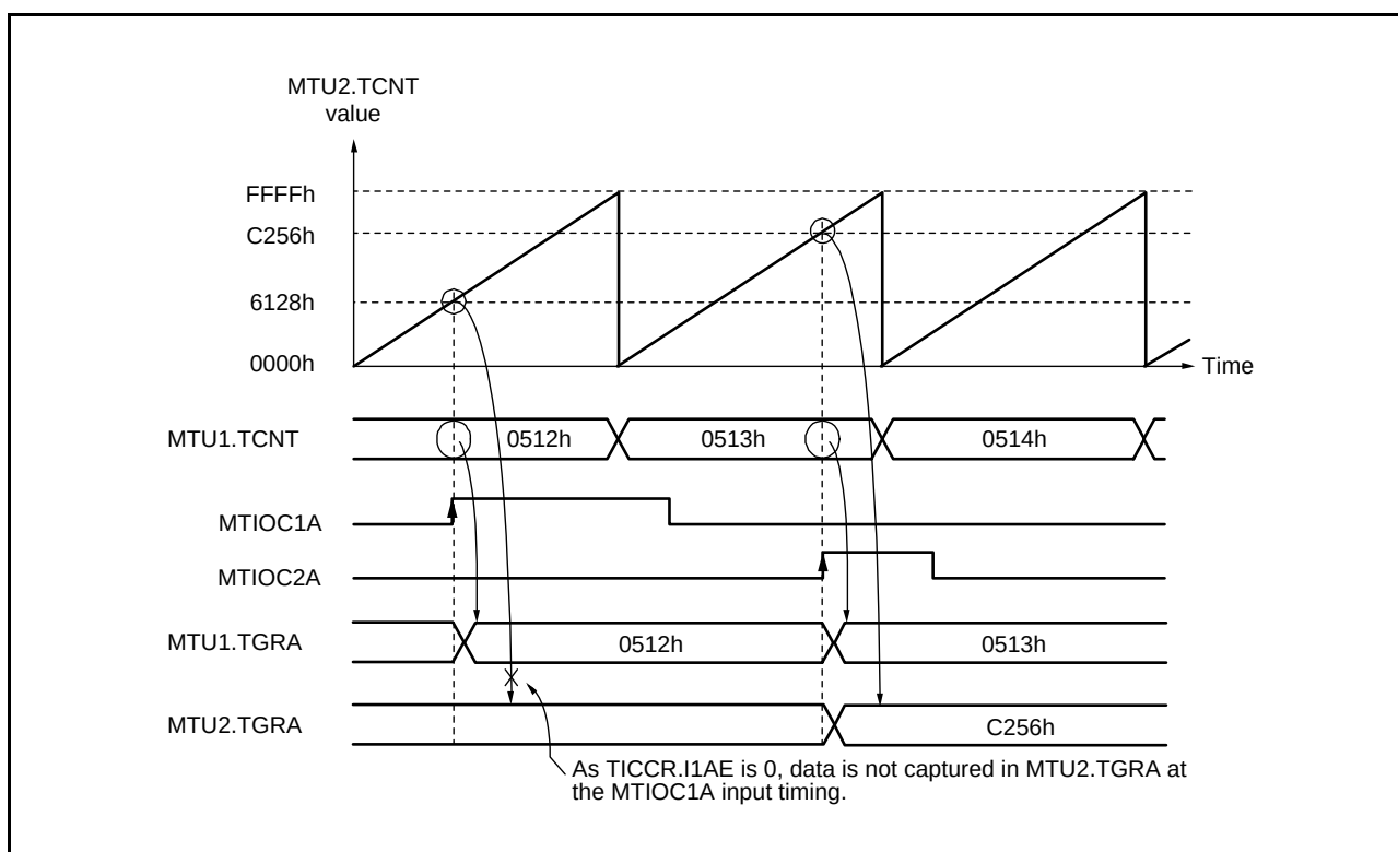
Figure 22.22 Cascaded Operation Example (b)
