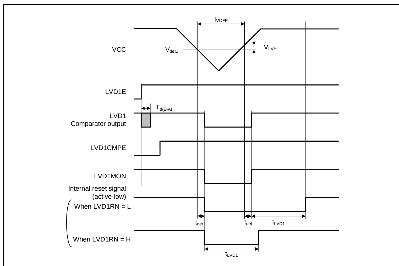
Figure 45.42 Voltage Detection Circuit Timing ( V_{det1} )
