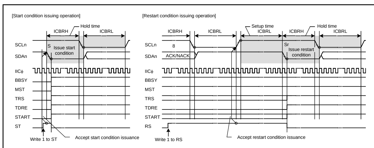
Figure 33.36 Start Condition/Restart Condition Issue Timing (ST and RS Bits)
