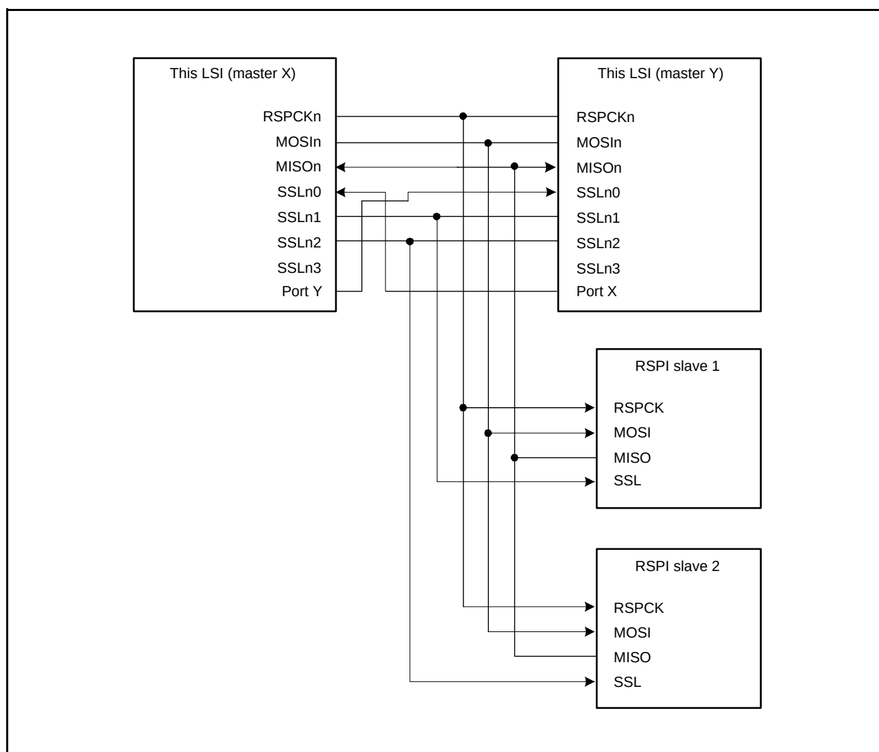
Figure 35.10 Multi-Master/Multi-Slave Configuration Example (This LSI = Master)
