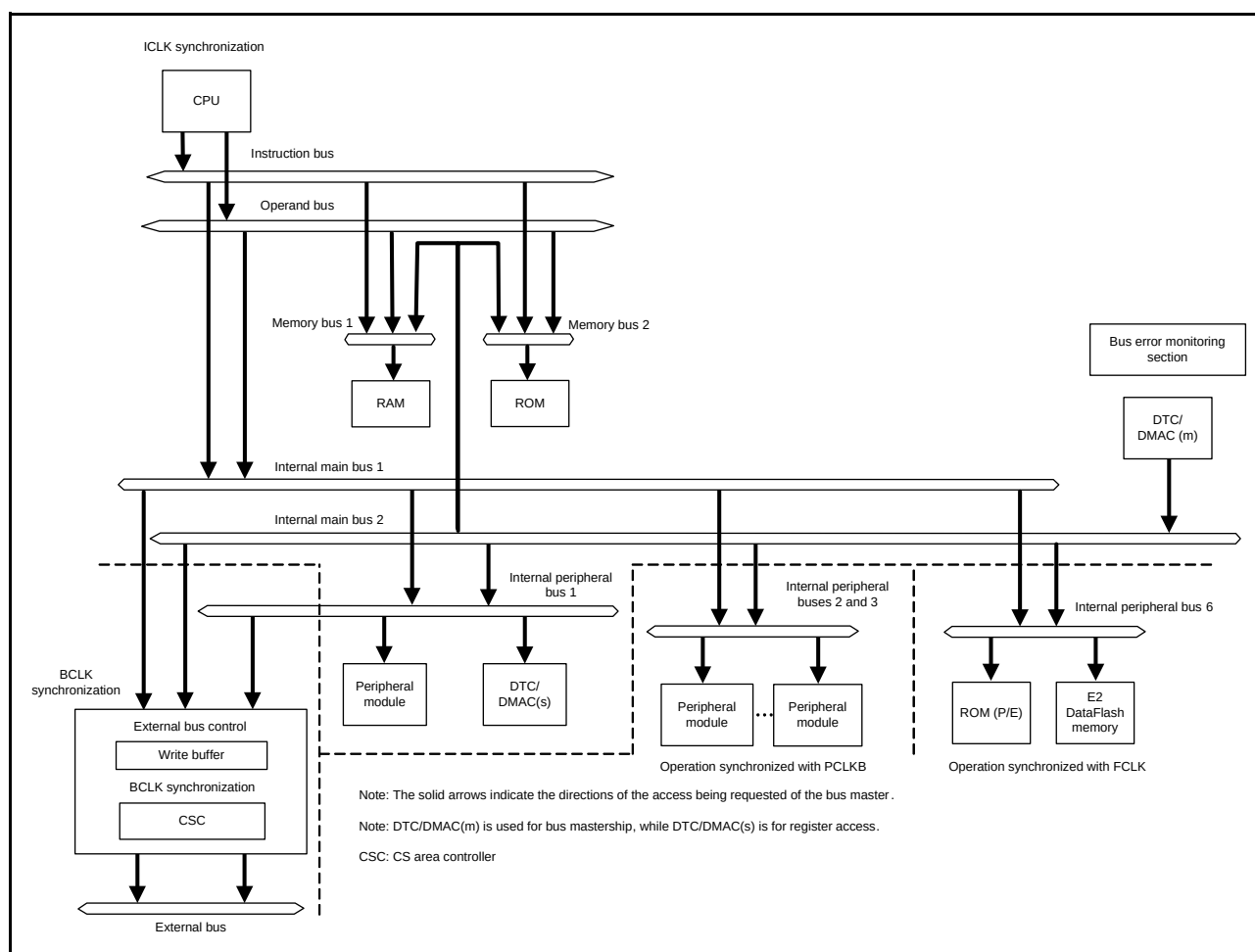
Figure 16.1 Bus Configuration
