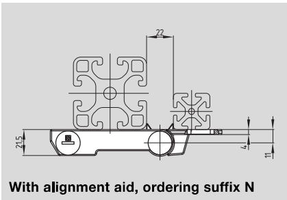
Top connector ST2, ST5
