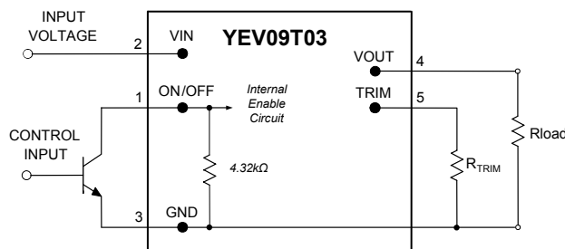
Figure 13. Circuit Configuration For ON/OFF Function
