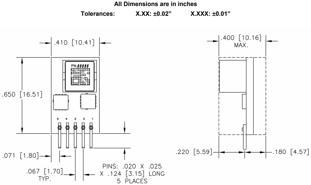
Figure 15. Mechanical Drawing
