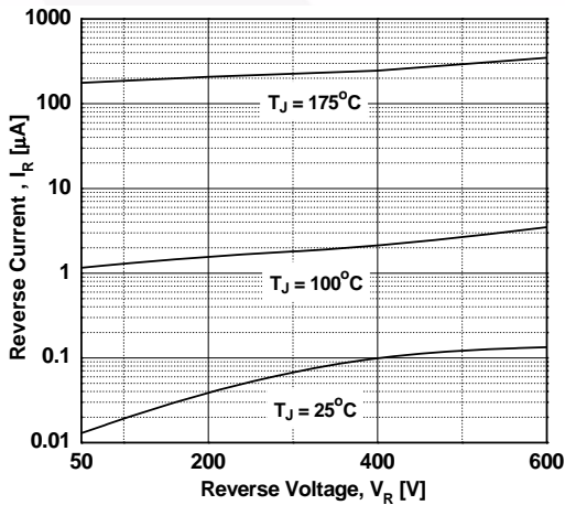
Figure 23. Reverse Current
